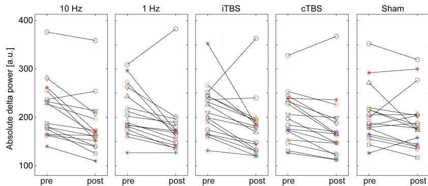
Figure 3: Pre- and post-rTMS absolute delta power on electrode AF3. Each subject is represented using a specific marker.
