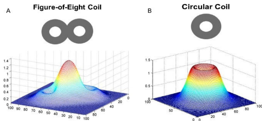
Figure 3.2: Magnetic field generated by the different coils: (a) magnetic field by a figure-of-eight coil and (b) magnetic field by a circular coil [Giordano 2012].
