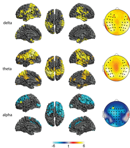
Figure 1: Group analysis of responders and non-responders in a group of patients. Blue colour indicates higher activity in non-responders, red colour higher activity in responders. Scalp and cortical maps are thresholded at p < 0.05 FWE ( T = 3.2 ). Yellow cross on the scalp and cortex indicates the target of stimulation.
