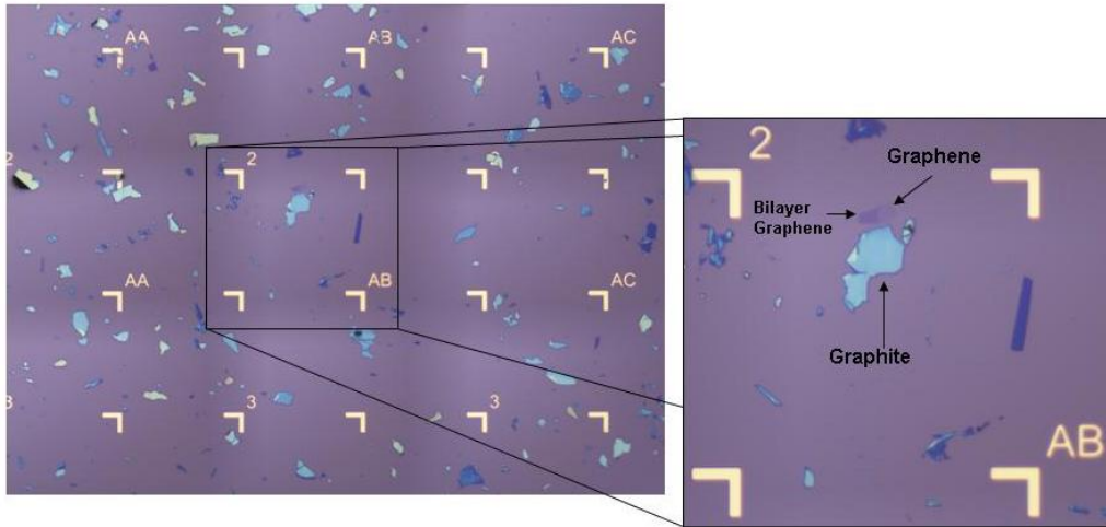
Figure 4.2: Optical observation of a Si/SiO 2 after a mechanical exfoliation and deposition of graphene. Zoom: minimum working area for e-beam lithography (100 \mu\text{m} by side). Marks and alpha-numeric symbols are used to localize the graphene flakes.
