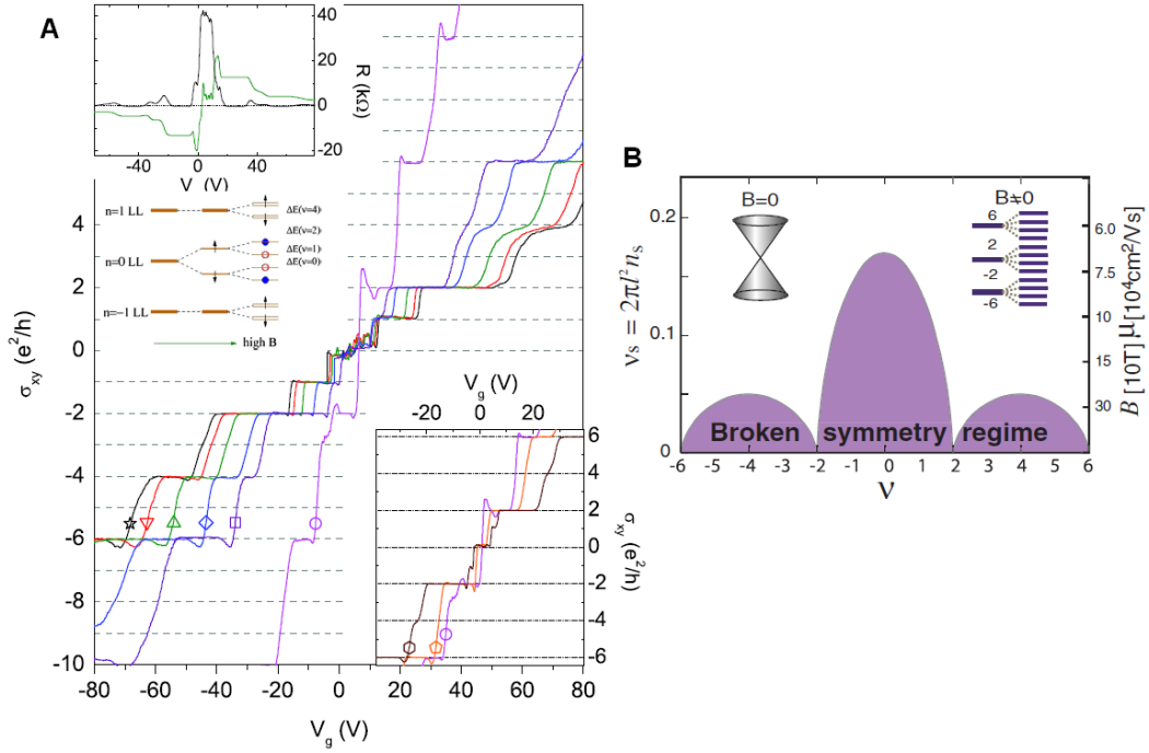
Figure 3.5: A , \sigma_{xy} measured on a graphene monolayer as a function of V_g at different magnetic fields: 9 T (circle), 25 T (square), 30 T (diamond), 37 T (up triangle), 42 T (down triangle), and 45 T (star). The data are taken at T=1.4 K, except for the B=9 T curve, which is taken at 300 mK. Left upper inset: R_{xx} and R_{xy} for the same device measured at 25 T. Left lower inset: a schematic drawing of the Landau levels in low (left) and high (right) magnetic fields. Right inset: detailed \sigma_{xy} data near the Dirac point for B=9 T (circle), 11.5 T (pentagon) and 17.5 T (hexagon) at T=30 mK. Adapted from [Zhang 2006]. B , Phase diagram for SU(4) quantum Hall ferromagnetism for the N=0 and N=1 Landau levels of graphene. Adapted from [Nomura 2006].
