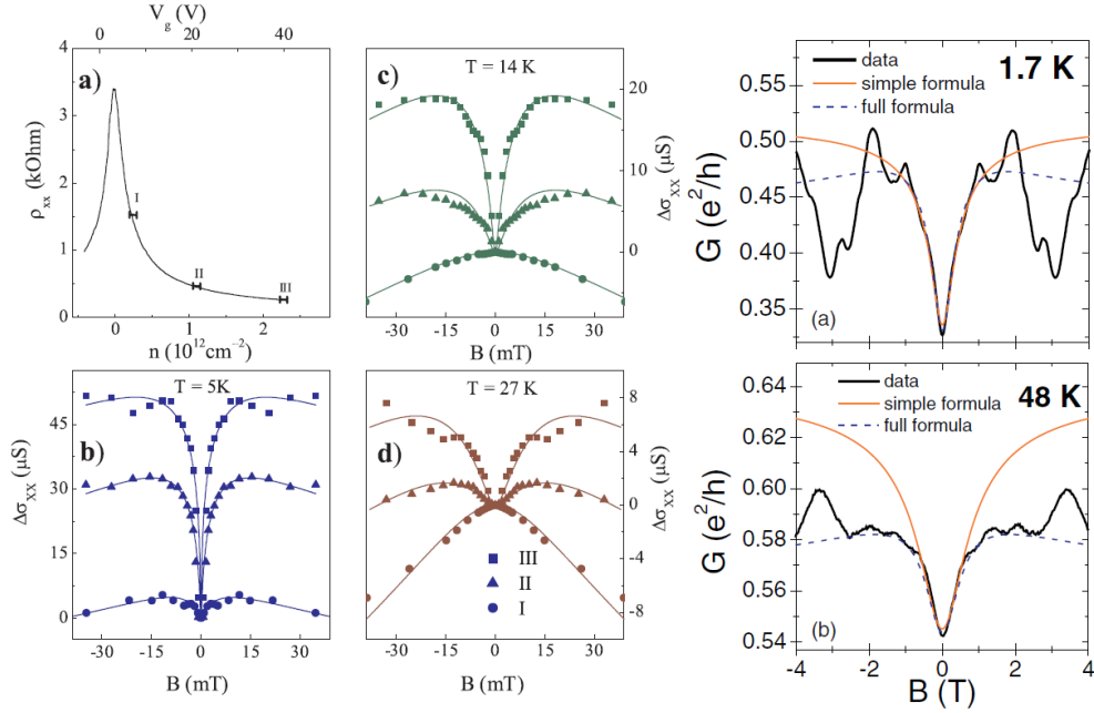
Figure 2.5: Left , (a) Resistivity as a function of the carrier density, with the three regions where the magneto-conductance is studied indicated by bars. (b)-(d) evolution of the magneto-conductance with decreasing the electron density at three temperatures: (b) T = 5 K, (c) T = 14 K and (d) T = 27 K. Adapted from [Tikhonenko 2009]. Right , Magneto-conductance for two different temperatures T = 1.7 K (a) and 48 K (b). Experimental curves (black) are fitted using the 1D expression for weak localization in metals eq. (2.11) (orange) and the expression for GNRs eq. (2.13) (dashed blue). Adapted from [Minke 2012a].
