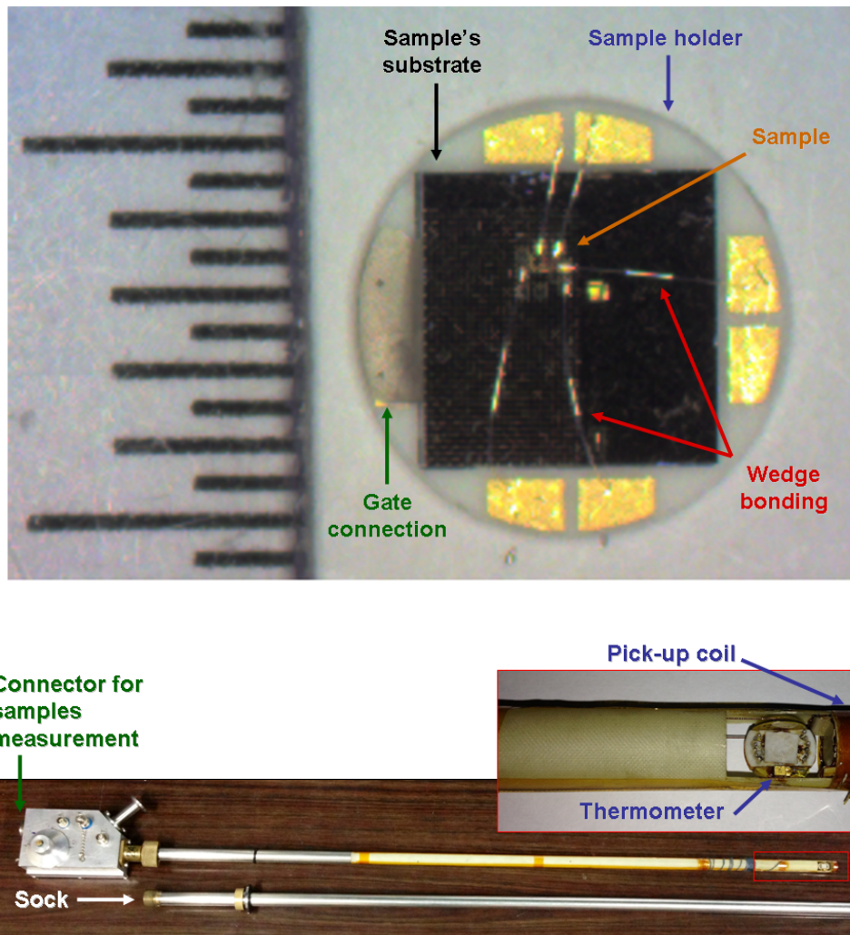
Figure 4.7: Top , GNRs sample connected to the sample holder through wedge bonding. Millimeter scale on the left. Bottom , photo of the magneto-transport insert specially designed for pulse magnetic field and cryogenic temperatures.
