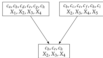
Figure 5.27: Region-graph resulting from the split of a TS(5,3) in two quadruplets
