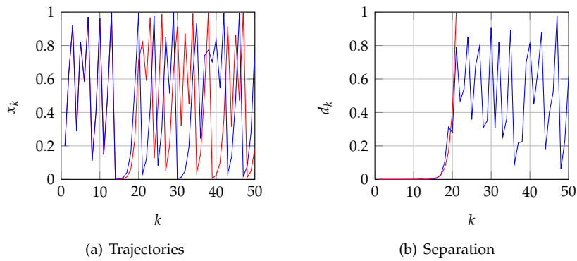
Figure 3.2: Logistic map
