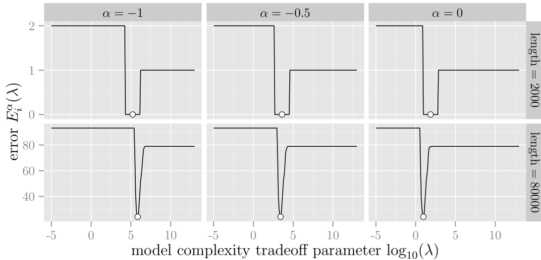
Figure 4.14: Breakpoint detection error curves for several penalty exponents \alpha and 2 samples of varying length in base pairs l_i . The penalty contains a term l_i^\alpha .
