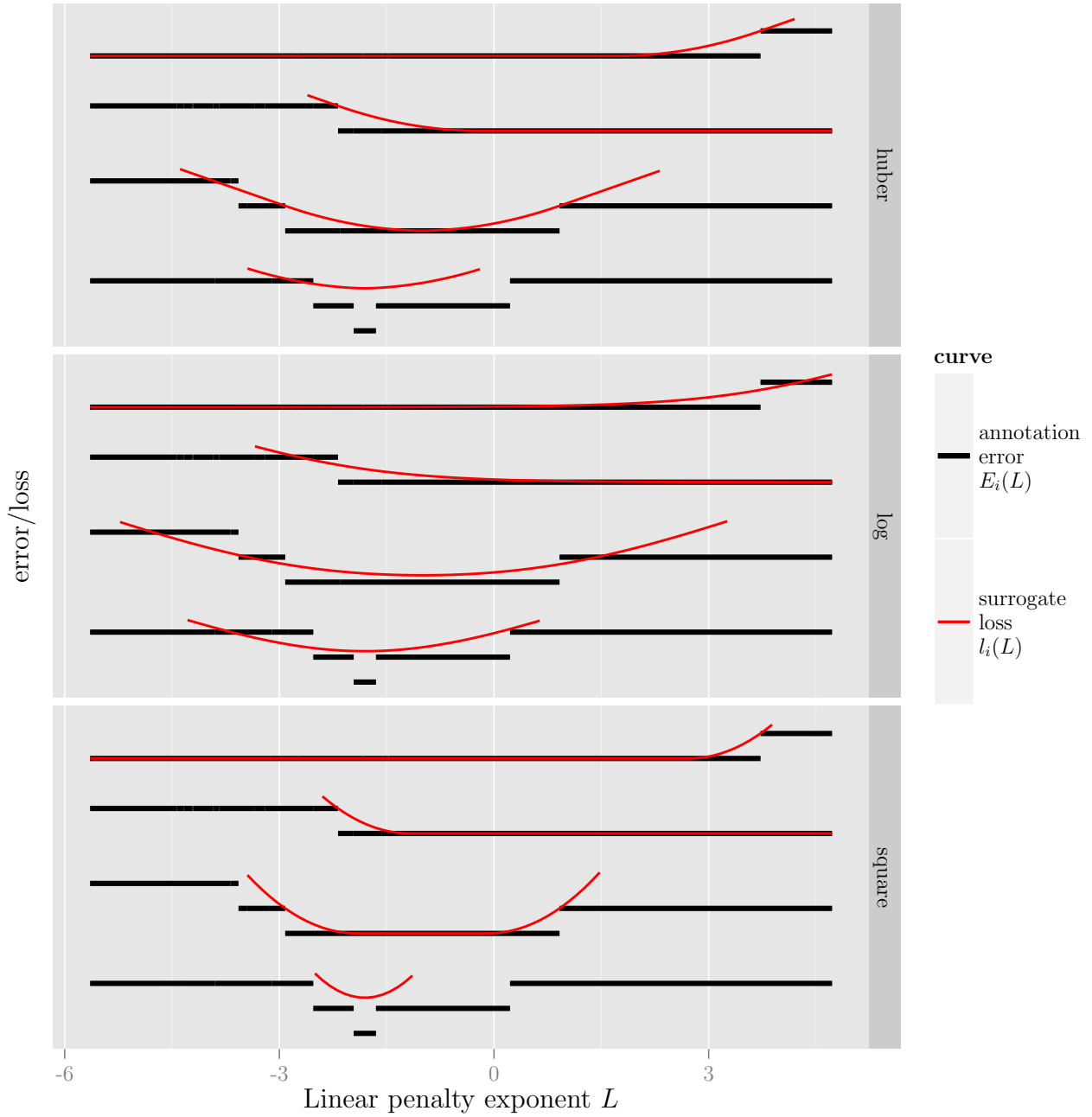
Figure 5.4: Several relaxations of the annotation error (panels from top to bottom). Each panel shows the annotation error E_i and its convex relaxation l_i for four signals i .
