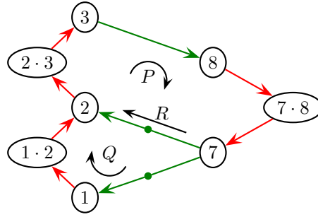
Figure 6.6: Cycle \mathcal{C} = 2 \xrightarrow{P} 7 \xrightarrow{Q} 1 \xrightarrow{R} 2 is a conflict-cycle (it contains 7 \rightarrow 1 \in X ). The length-1 path R forms a shortcut for \mathcal{C} (with \mathcal{C}' = 2 \xrightarrow{P} 7 \xrightarrow{R} 2 , \mathcal{C}' is a conflict-cycle, and W(Q) = \{\langle 1, 2 \rangle\} ). So \mathcal{C}' is the only minimal conflict-cycle.
