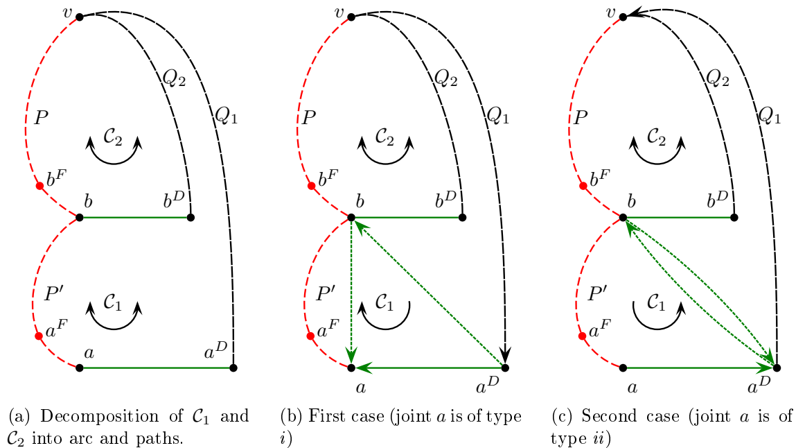
Figure 6.9: Path decomposition of \mathcal{C}_1 and \mathcal{C}_2 and case study for Lemma 6.12.
