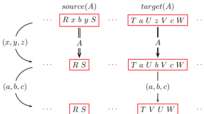
Figure 1.9: The activation of a variable A = [(a, b, c), (x, y, z)] is written with a double arc in the behavior graph of the source block of A and with a thick arc in the behavior graph of its target block. It can be followed by the 3DT-step \xrightarrow{(a, b, c)} , impacting only the target block of A . Dot symbols ( \cdot ) are omitted. We denote by R, S, T, U, V, W some factors of the source and target blocks of A : the consequence of activating A is to allow U and V to be swapped in target(A) .
