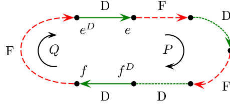
Figure 6.8: Illustration of Lemma 6.10, with \lambda = 6 . Here e_s = e^D , e_t = e , f_s = f^D , f_t = f .
