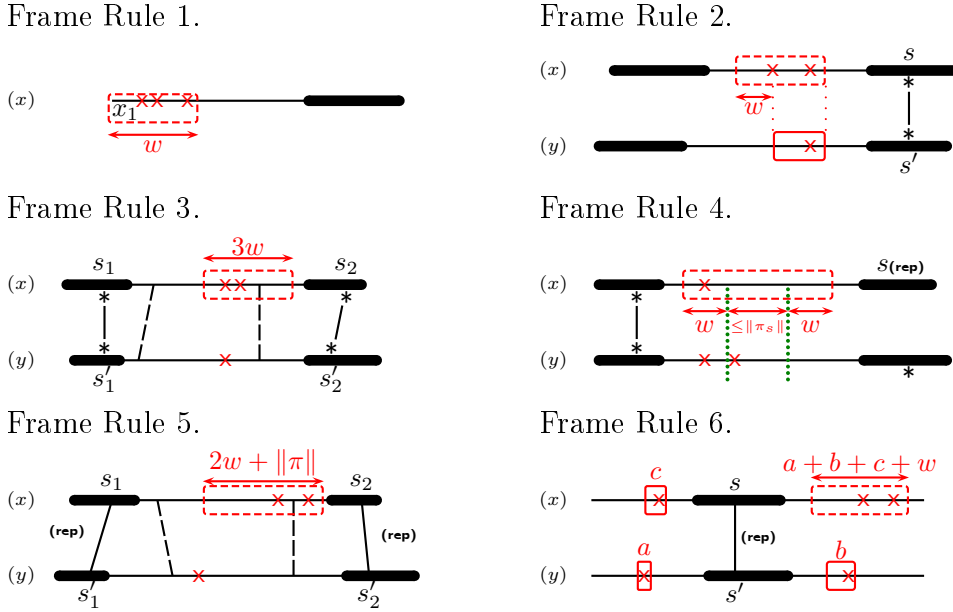
Figure 4.4: Frame Rules 1–6 of frames. Frames are drawn as red boxes, the frame created at each step is dashed. Possible breakpoint positions in \mathcal{P} are shown as red crosses.
