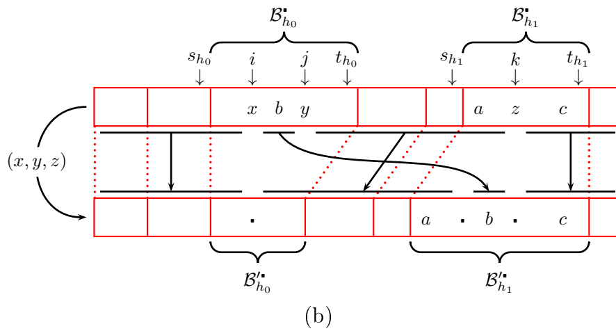
Figure 1.8: Effects of a 3DT-step \underline{(d, e, f)} on an l -block decomposition if (a) (d, e, f) is an internal triple, or (b) there exists a variable A = [(a, b, c), (x, y, z)] such that (d, e, f) = (x, y, z) . Both figures are in fact derived from Figure 1.3 in the context of an l -block decomposition.
