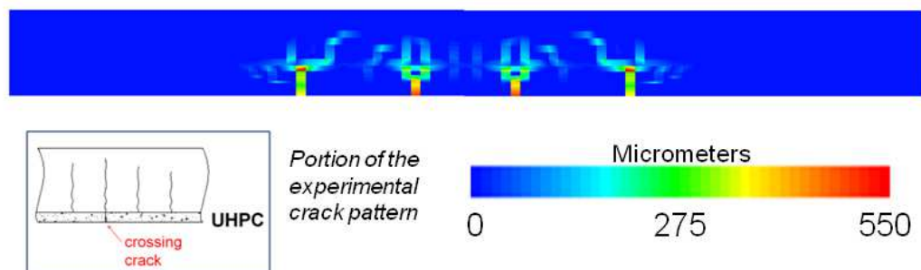
Figure 3.26 - Cracks width of the UHPC repaired beam at 15 mm of imposed vertical displacement. Numerical results for the entire beam obtained by symmetry
