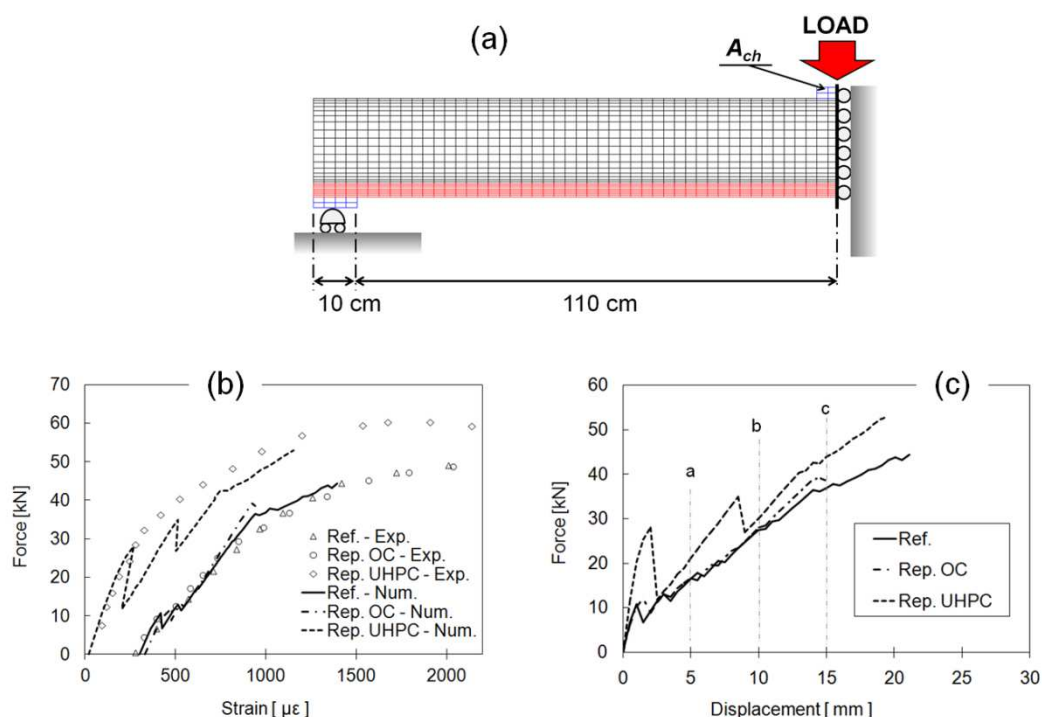
Figure 3.24 - Mechanical boundary conditions and geometrical configuration for the three points bending test (a); Force versus averaged strain of the compressed fiber optic sensor (b); Force versus displacement curves (numerical results) (c)
