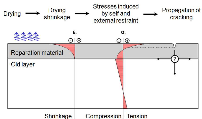
Figure 3.15 - Drying cracking due to self and external restraint in a reparation (adapted from Molez, 2003)
