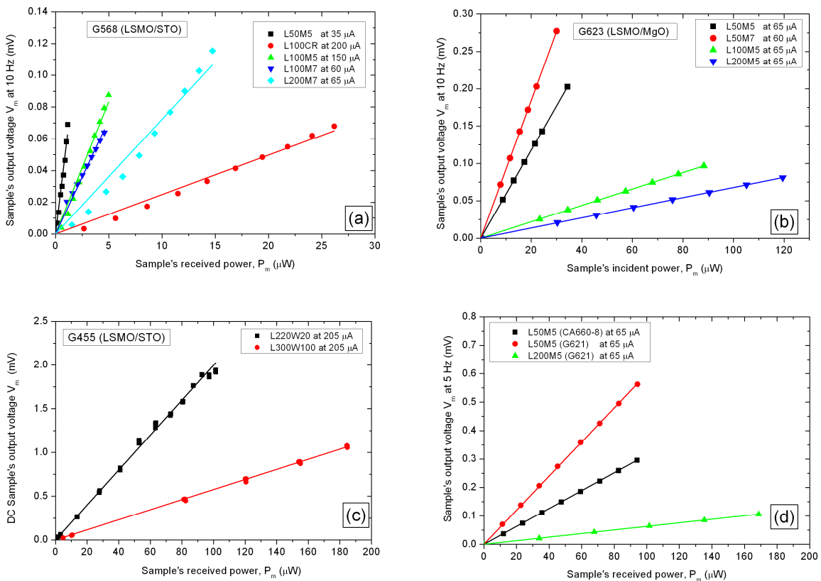
Figure 3-16. The output voltage ( V_m ) versus the received power ( P_m ) at T_{opt} for (a) G568(LSMO/STO) samples at modulation frequency 10 Hz, (b) G623 (LSMO/MgO) samples at modulation frequency 10 Hz, (c) G455 (LSMO/STO) samples at DC, and (d) G621 and CA660-8 (LSMO/STO/Si) samples at modulation frequency 5 Hz. The lines are guides for the eyes
