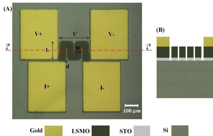
Figure 2-30. (A) Optical photography of the mask-A CA656-7(L150W50) sample with the measurement current ( I+ , I- ) and voltage ( V+ , V- ) probes. (B) Schematic cross-section of the sample.
