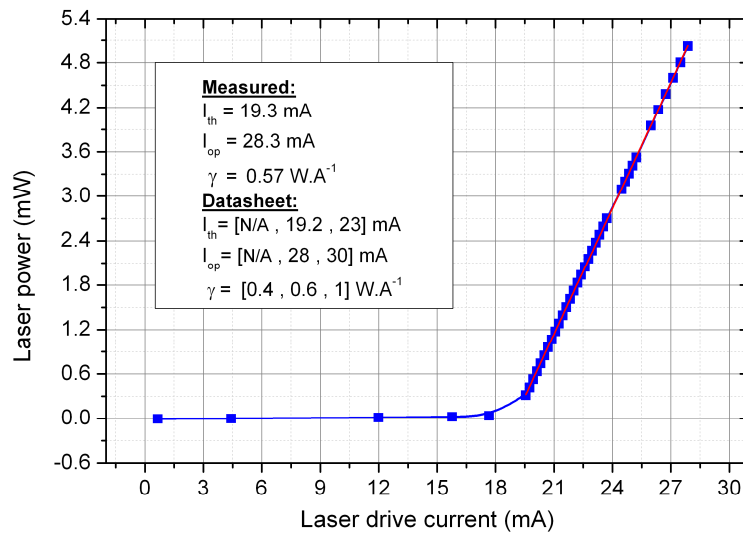
Figure 2-8. The measured laser diode power versus laser drive current at 21 °C. The legend shows the measured and datasheet characteristics
