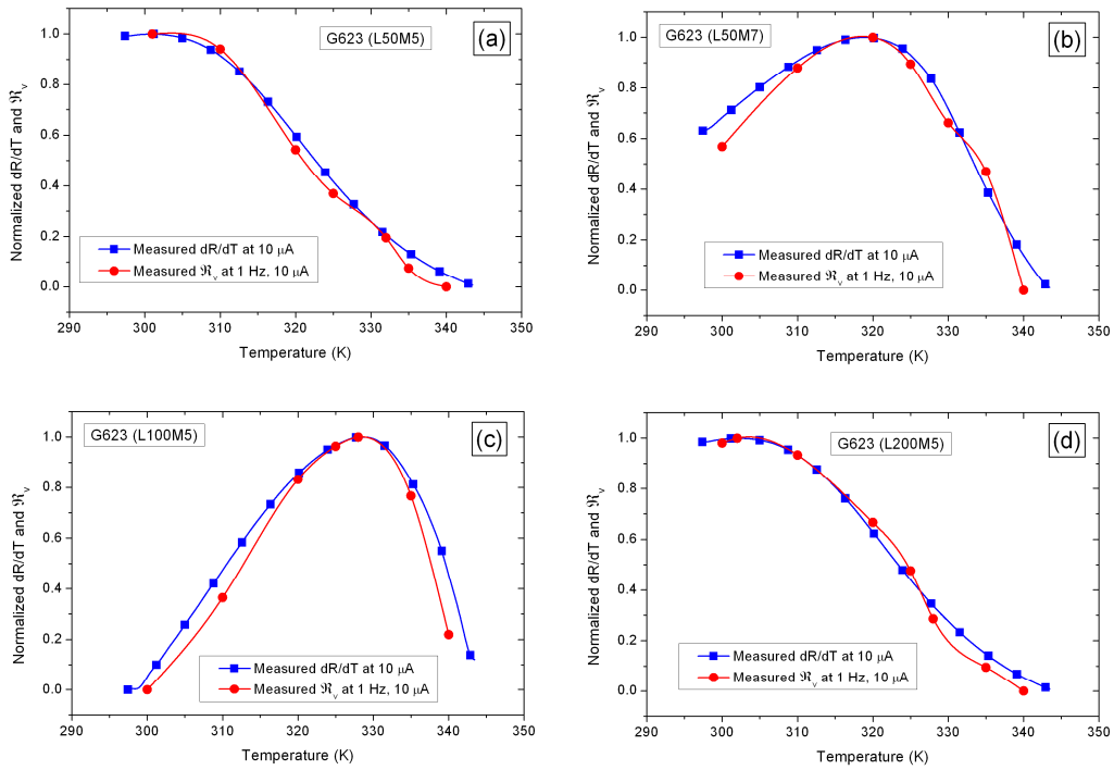
Figure 3-18. The normalized optical responsivity (at 10 \mu\text{A} and frequency 1 Hz) and dR/dT (measured at 10 \mu\text{A} ) versus temperature curves for G623 (LSMO/MgO) samples
