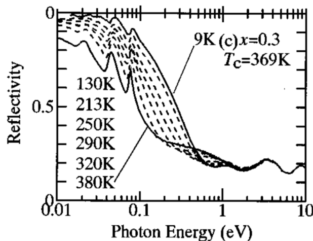
Figure 1-18. Reflectivity spectra at various temperatures in La_{0.7}Sr_{0.3}MnO_3 [37]
