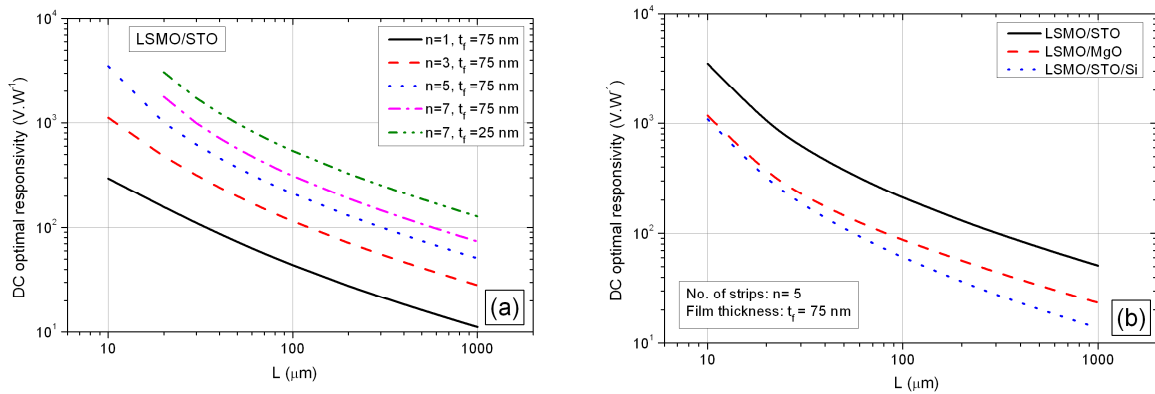
Figure 3-37. The calculated DC optimal responsivity versus pixel size, L , for (a) square and meander geometries with n number of strips and STO substrate material, (b) for 5 strips and 75 nm film thickness, and for the three types of substrate materials
