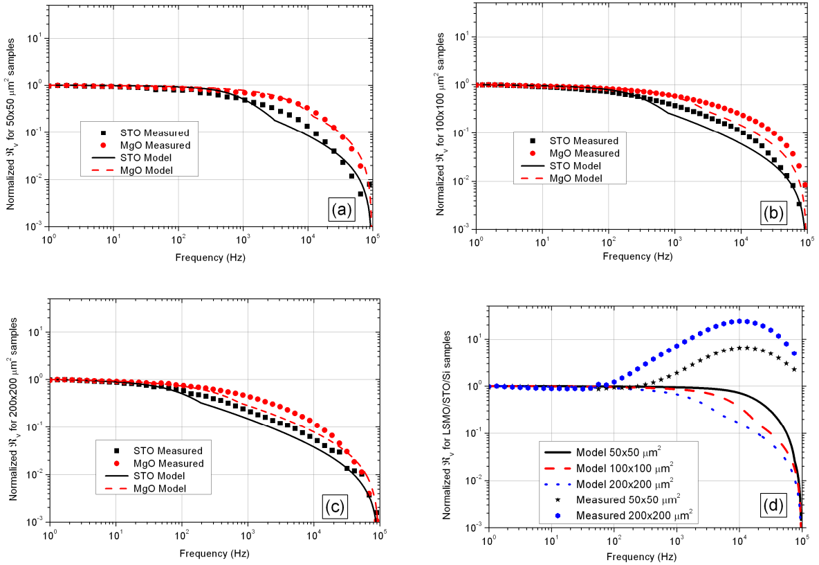
Figure 3-35. Measured and calculated normalized (at 1 Hz) optical responsivity at T_{\text{opt}} of LSMO film on STO (G568) and MgO (G623) substrates materials for (a) 50×50 μm 2 sample size, (b) 100×100 μm 2 sample size, (c) 200×200 μm 2 sample size, (d) and LSMO/STO/Si (G621) samples
