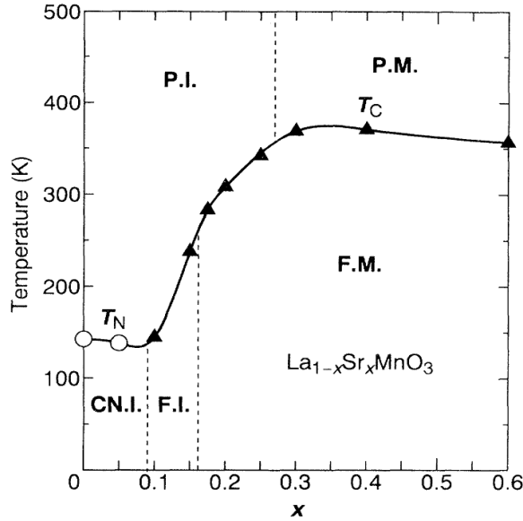
Figure 1-14. Phase diagram of La_{1-x}Sr_xMnO_3 . Open circles and filled triangles are the Neel ( T_N ) and Curie ( T_C ) temperatures, respectively. The abbreviations mean paramagnetic insulator (PI), paramagnetic metal (PM), spin-canted insulator (CNI), ferromagnetic insulator (FI), and ferromagnetic metal (FM) [36]
