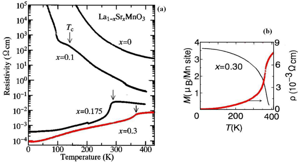
Figure 1-15. (a) Temperature dependence of the electrical resistivity in crystals of La_{1-x}Sr_xMnO_3 . Arrows indicate the respective Curie temperature T_c [37], (b) electrical resistivity versus temperature for x=0.3 [36]
