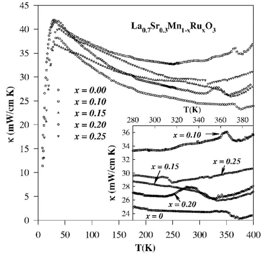
Figure 1-17. Temperature-dependent thermal conductivities for La_{0.7}Sr_{0.3}Mn_{1-x}Ru_xO_3 with 0 \leq x \leq 0.25 . The inset shows the blow-up plot near phase transitions [49]
