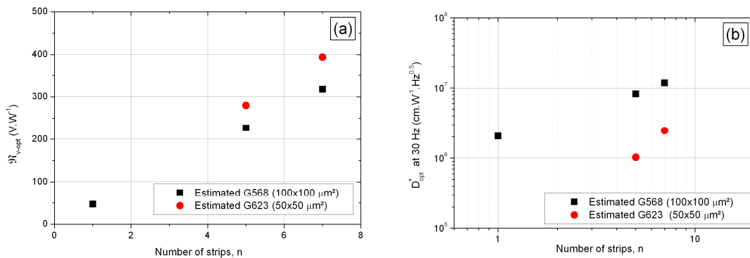
Figure 3-46. Optical responsivity (a) and specific detectivity (b) versus number on strips for LSMO film on STO and MgO substrates at I_{\text{opt}} and T_{\text{opt}}
