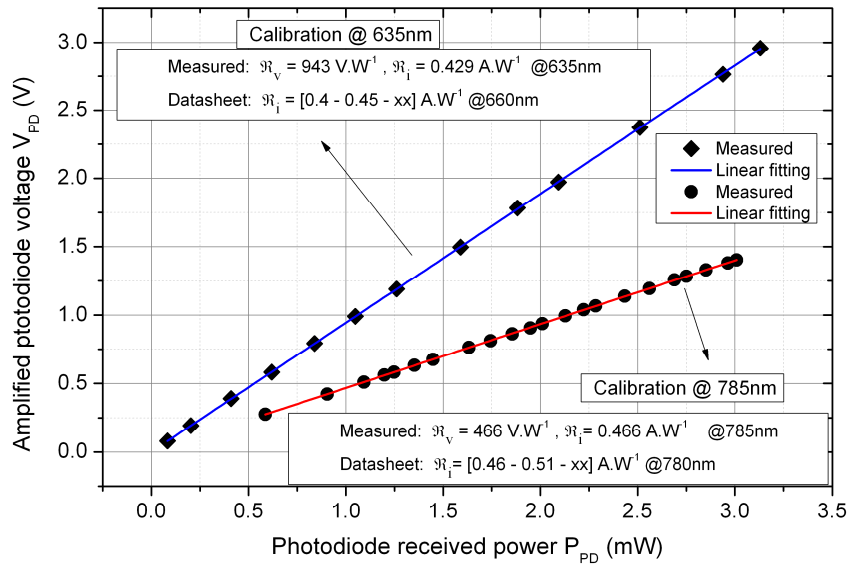
Figure 2-15. Static calibration of S10784 photodiode with I/V Amplifier at 635 nm and 785 nm wavelength. The legends show measured and datasheet characteristics
