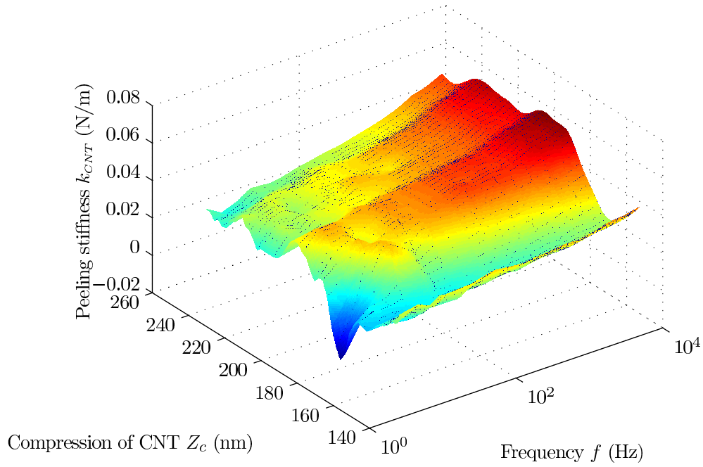
FIGURE 6.20 – 3D plot of peeling stiffness of the nanotube k_{CNT} as a function of frequency f and compression of nanotube z_c .
