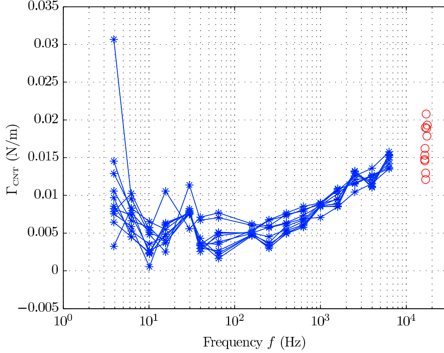
FIGURE 6.16 – Dissipation as a function of frequency at various positions along the nanotube while it is being peeled from the surface with the excitation applied by the piezo. The red circles correspond to the dissipation inferred from the time-frequency analysis of the thermal noise.
