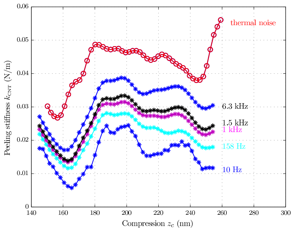
FIGURE 6.19 – Peeling stiffness k_{\text{CNT}} as a function of the compression of the nanotube for various frequencies. The obvious tendency of k_{\text{CNT}} to increase with the frequency can be found. The shape of those curves implies that the mechanical properties of the CNT are not uniform as it is being peeled with a compression from z_c = 270 nm to 140 nm.
