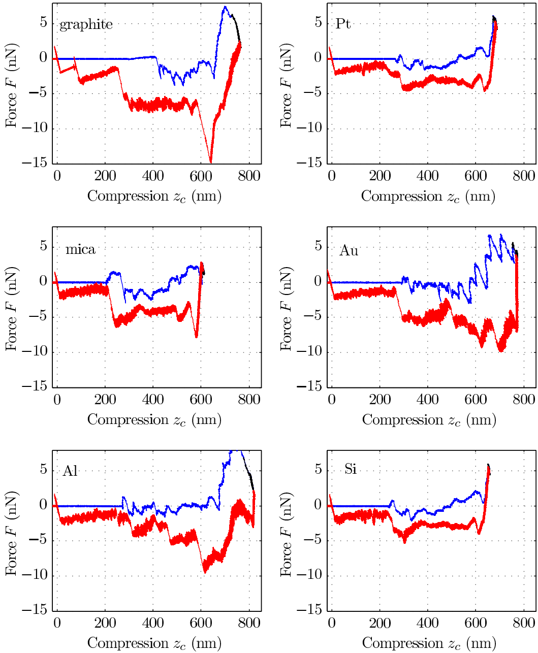
FIGURE 5.3 – Measured force curves on various substrates : graphite, Pt, mica, Au, Al, and Si as a function of compression. We compute the value of E_a from the longest force plateau, around 300 nm to 500 nm.
