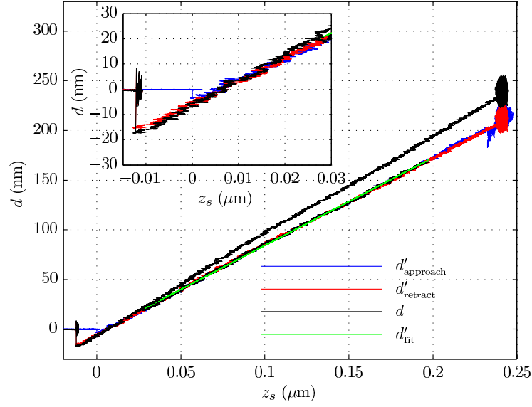
FIGURE 5.6 – Deflexion d as a function of the position of piezo z_s in hard contact, the inset figure illustrates the area where the cantilever tip get and loose contact with the surface. By fitting the curve (red), the real deflexion of the cantilever can be given by d = d'/\alpha .
