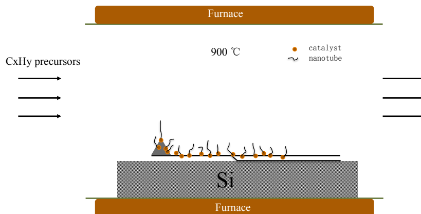
FIGURE 4.4 – Schematic diagram of CVD reaction chamber. Nanotubes grow everywhere on the cantilever and tip from the catalyst nanoparticles
