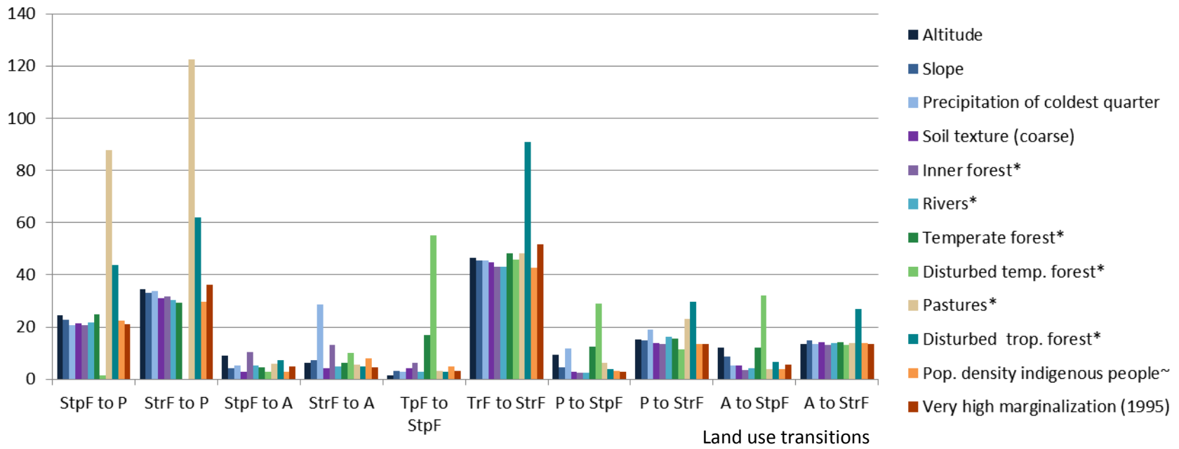
Figure 6. Importance of drivers as the % of individual contribution to variance of major LUCC transitions for 1993-2002 (for explanation of abbreviations see figure 3, * euclidean distance).
