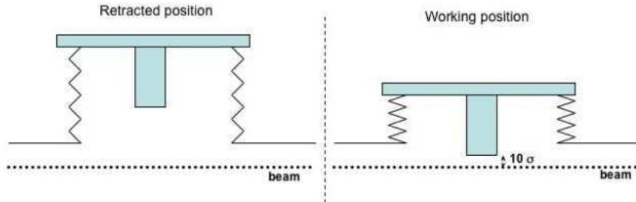
Figure 2.22: Roman Pot concept: on the left the retracted position is shown where the pot is in parking position, whereas on the right – in working position, 10 \sigma close from the beam centre, where \sigma is a Gaussian width of the beam.
