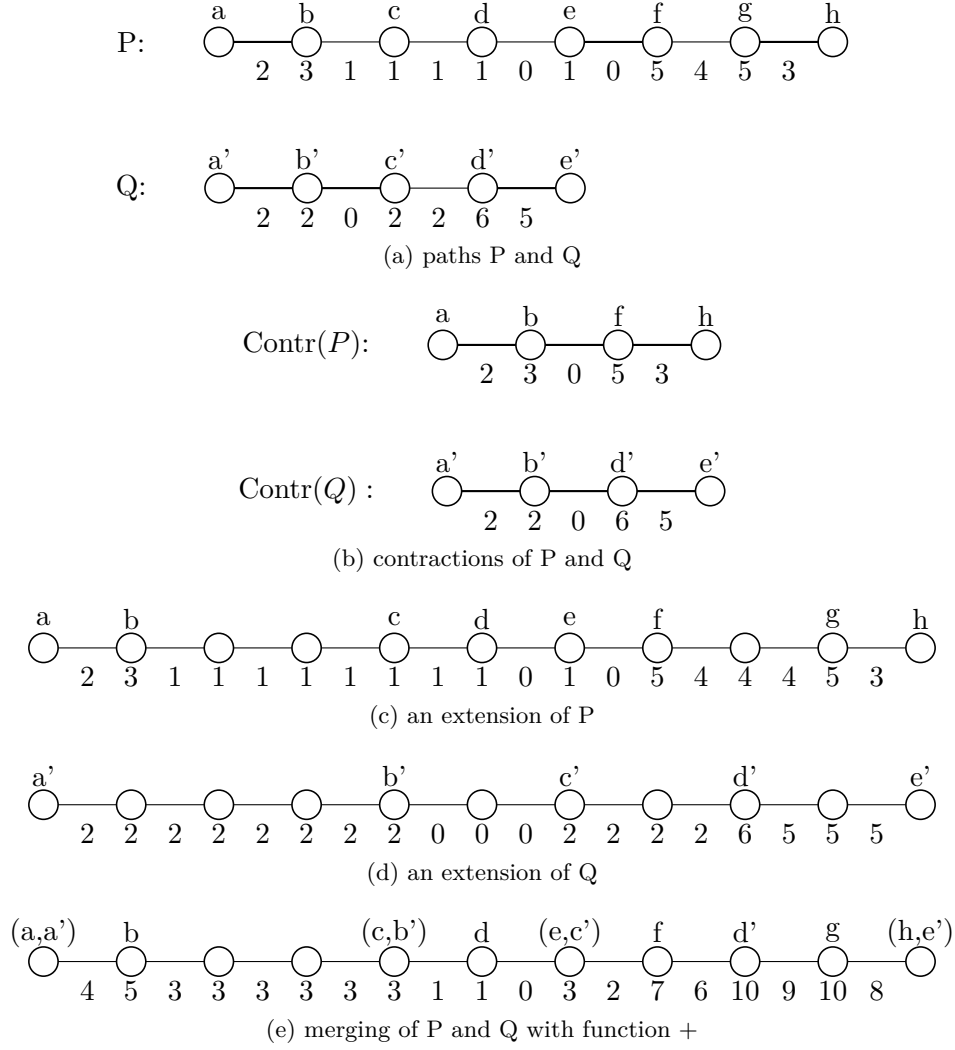
Figure 4.2: labelled paths: contraction, extension and merging. The labels of first and last vertex are omitted, since they do not change with any operation.
