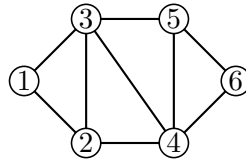
Figure 5.1: Example of a dismanttable graph, with vertices numbered according to the ordering.
