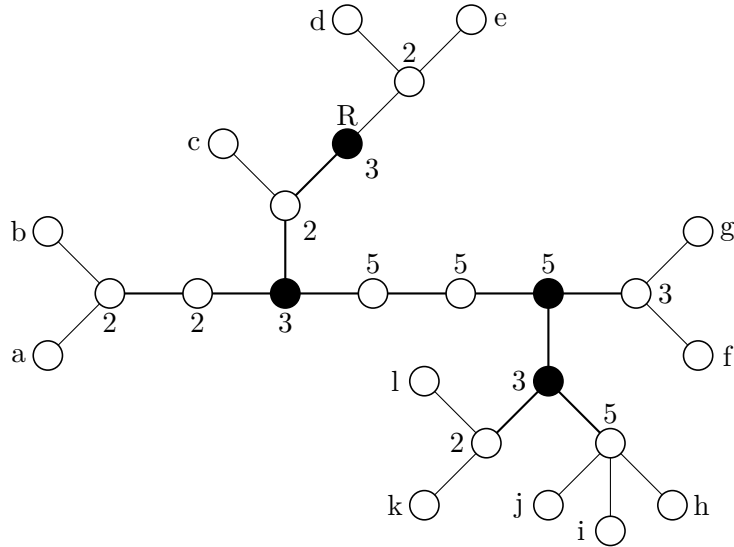
(a) labelled partitioning tree
