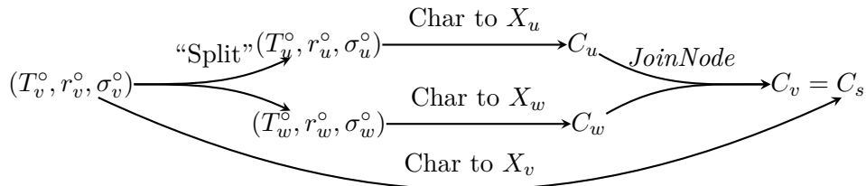
Figure 4.8: Scheme of proof of Lemma 37.
