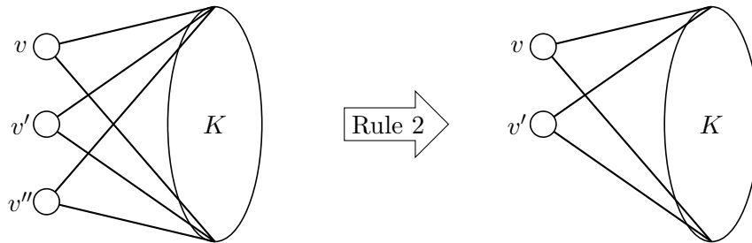
Figure 9.6: False twin vertices v, v' and v'' have their neighbourhood represented by the ellipse. The vertex v'' is identified into v after application of Rule 2.
