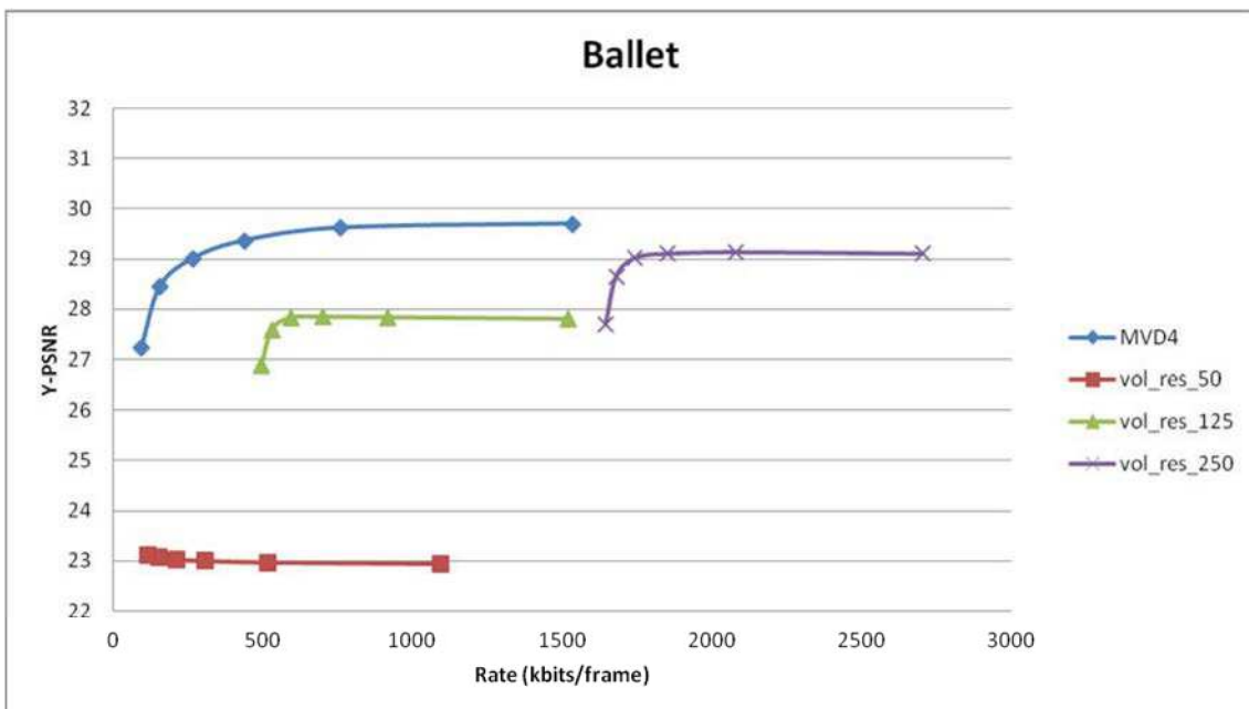
Figure 11.7: Rate/distortion curves for varying volumetric resolutions vs. reference model for ballet sequence.
