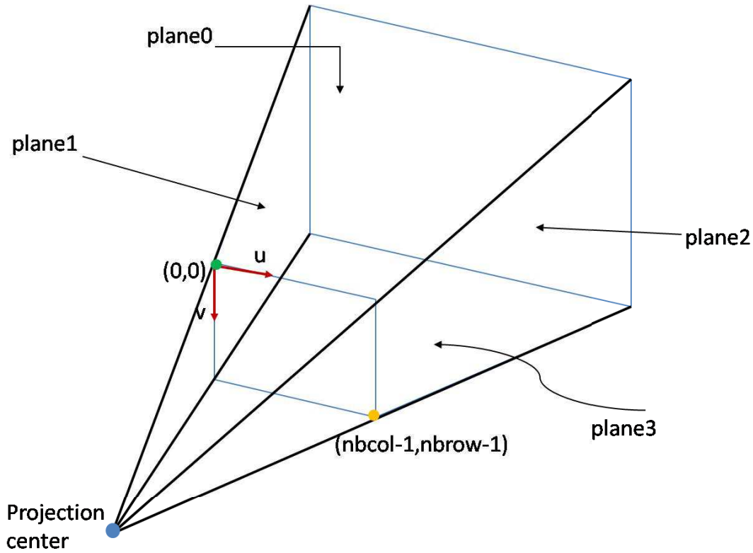
Figure 1.2: Calcul des plans du Frustum de projection.
