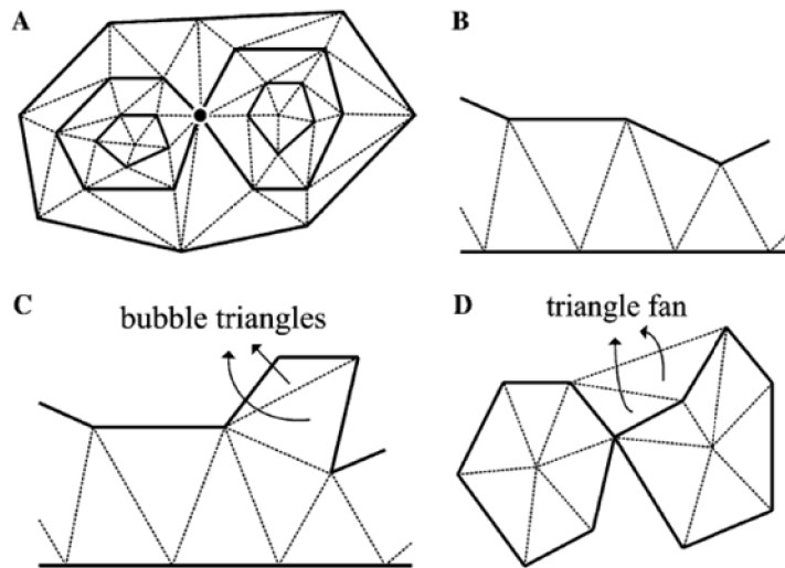
Figure 10.4: Layered decomposition method. (A): Layered vertex structure showing a different contours (thick lines) and branching point (black dot); (B): Triangle strip; (C): Bubble triangles: all vertices are belong to one contour; and (D): Triangle fan (image from [Peng et al., 2005]).
