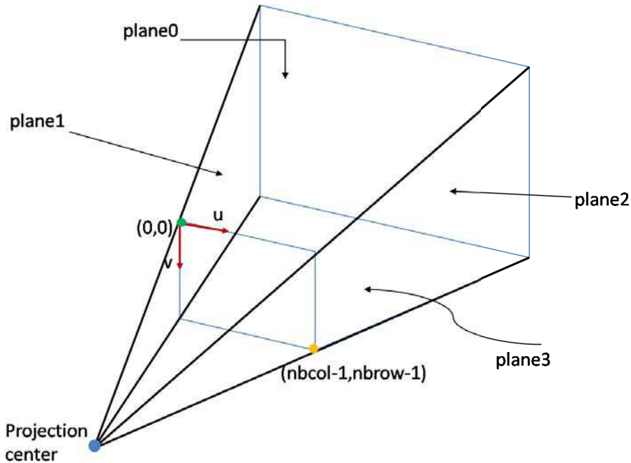
Figure 6.3: Frustum planes computation.
