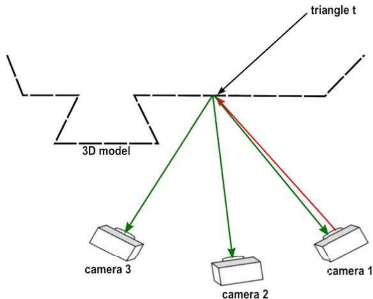
Figure 8.1: Best texture determination using photoconsistency. Red arrow for texture mapping operation and green arrow for projection operation.
