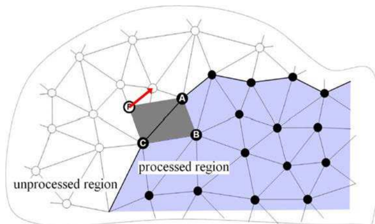
Figure 10.7: Parallelogram prediction rule (image from [Isenburg and Alliez, 2002])
