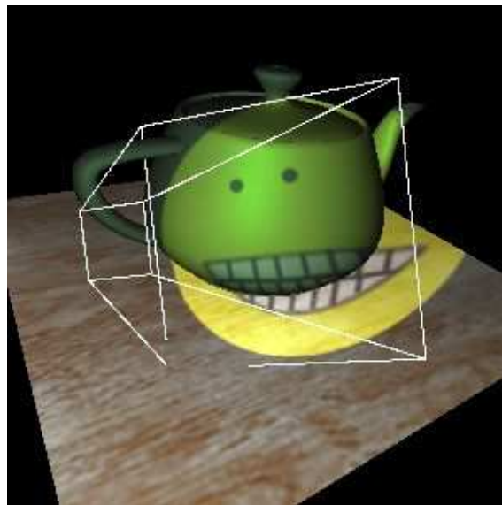
Figure 7.4: Projective texture mapping. A slide projector is projecting a smiley face onto the teapot. (image from http://home.xyzw.us/~cass/demo_images )
