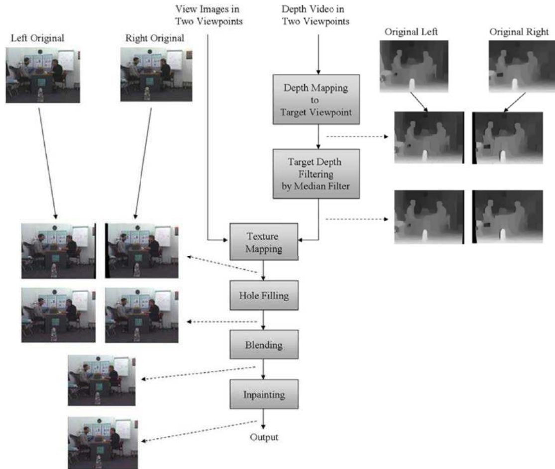
Figure 9.6: View synthesis in VSRS2.0 (image from [Tanimoto and Suzuki, 2009].)
