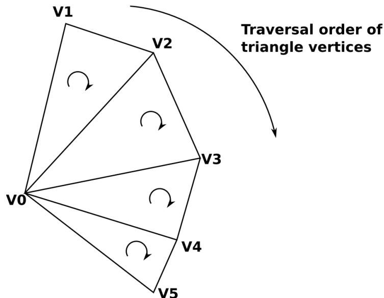
Figure 10.13: Triangle fan of degree 4.
