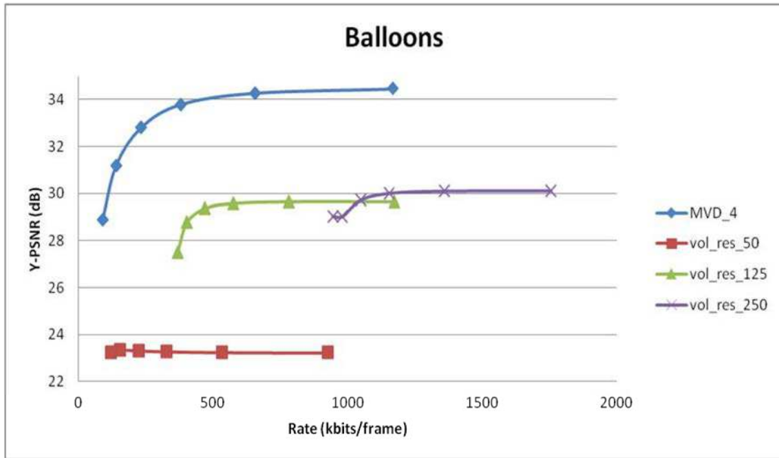
Figure 11.8: Rate/distortion curves for varying volumetric resolutions vs. reference model for balloons sequence.
