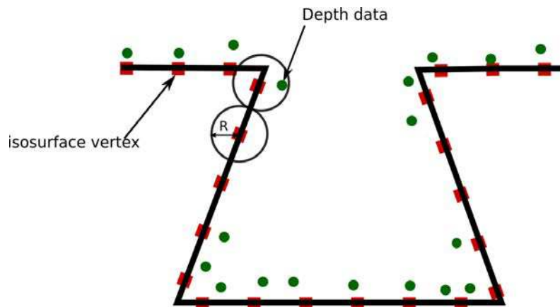
Figure 6.9: Post processing the merged mesh. A merged-mesh vertex represented with red square is mapped to the closest input-mesh-vertex represented with green circle if the distance between the vertices is below R .
