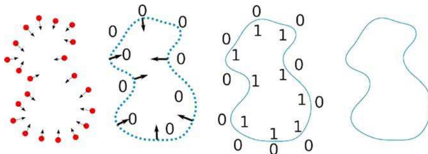
Figure 5.5: Poisson surface reconstruction. From left to right: an oriented point set \vec{V} , gradient of the indicator function \nabla\chi , indicator function \chi , final surface S .
