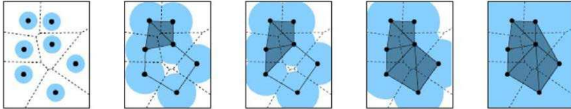
Figure 5.4: Construction of alpha shapes with increasing ball radius (image from [Dey et al., 2003]).
