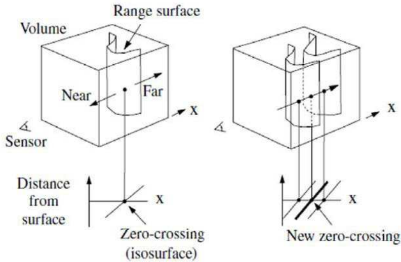
Figure 5.6: Unweighted signed distance functions in 3D. Left: A range sensor looking down the x -axis observes a range image, shown here as a range surface. Following one line of sight down the x -axis, a signed distance function as shown. The zero crossing of this function is a point on the range surface. Right: The range sensor repeats the measurement, but noise in the range sensing process results in a slightly different range surface. In general, the second surface would overlap the first, but we have shown it as an offset from the first surface for purposes of illustration. Following the same line of sight as before, we obtain another signed distance function. By summing these functions, a cumulative function can be obtained with a new zero crossing positioned midway between the original range measurements. See equations 5.2 and 5.3. Image from [Curless and Levoy, 1996]
