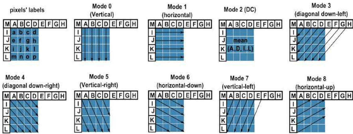
Figure 3.2: Spatial prediction modes.
