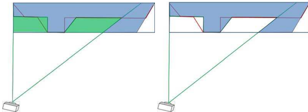
Figure 6.5: Space carving according to the left camera. Rays are cast from the camera center to the corresponding VMH (left). Green areas are carved. The result of this carving operation according to the green camera is shown on the right.
