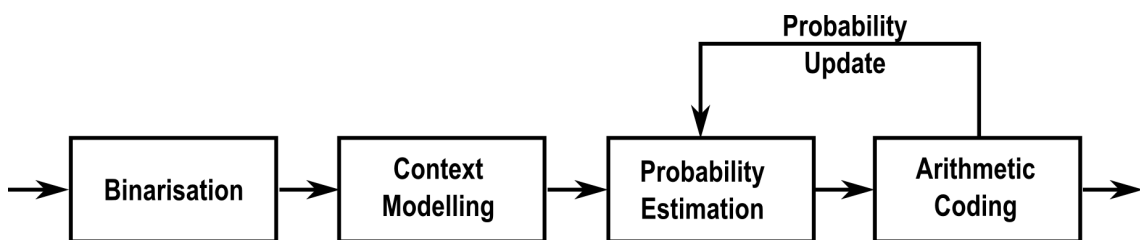
Figure 3.7: CABAC bloc diagram.
