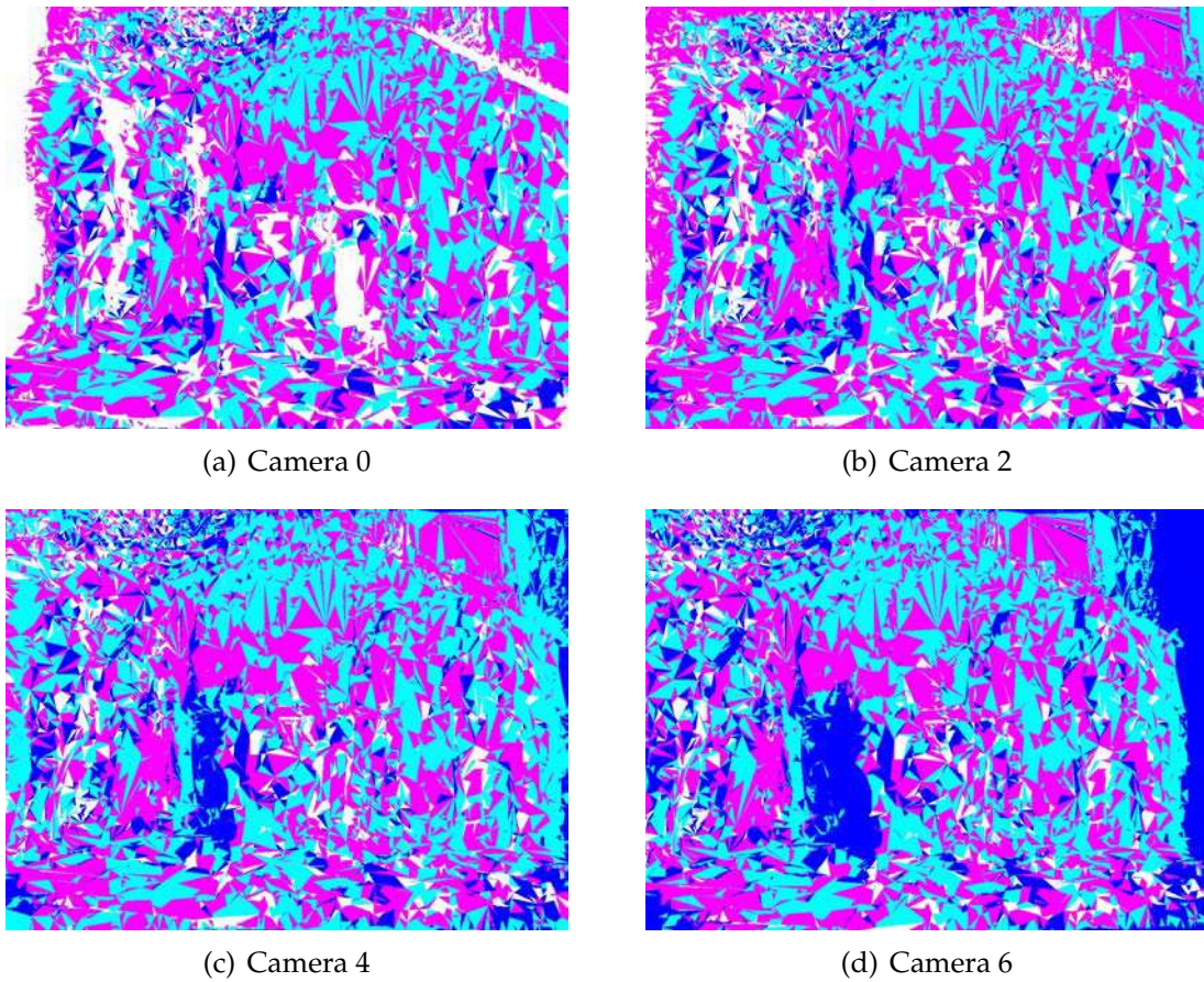
Figure 8.5: Best texture distribution for breakdancers sequence. White: camera 0, Magenta: camera 2, Cyan: camera 4, Blue: camera 6.
