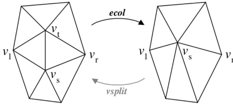
Figure 6.8: Edge collapse operation for mesh simplification (image from [Lindstrom and Turk, 2000]).
