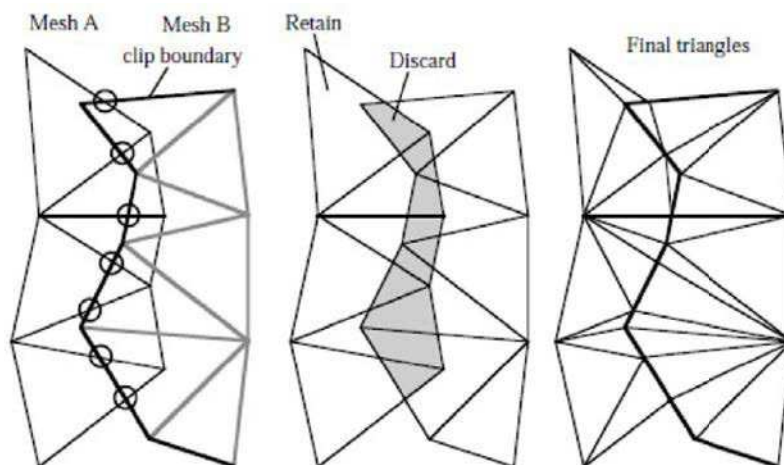
Figure 4.7: Mesh A is clipped against the boundary of mesh B. Circles (left) show intersection between edges of A and B's boundary. Portions of triangles from A are discarded (middle) and then both meshes incorporate the points of intersection (right) [Turk and Levoy, 1994].
