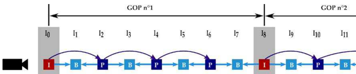
Figure 3.5: Prediction structures in earlier MPEG video standards.
