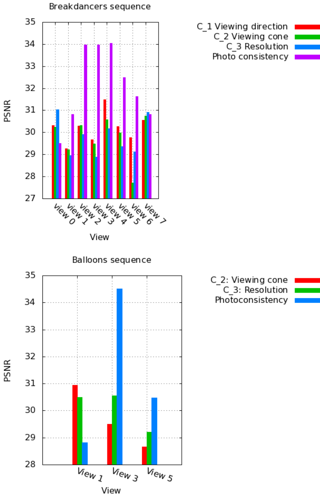
Figure 8.8: PSNR evolution through different views using different criteria for Breakdancers and Balloons sequences.
