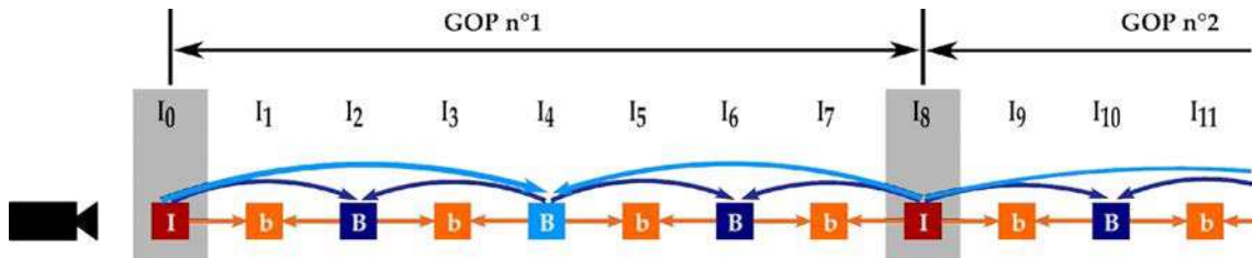
Figure 3.6: Prediction structures in H.264/AVC standard yielding a hierarchical GOP predicting structure.
