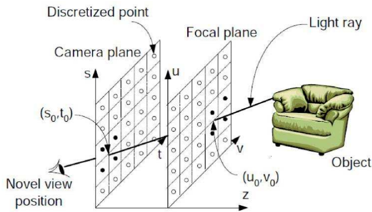
Figure 4.2: Representation of a light field (image from [Shum and Kang, 2000]).
