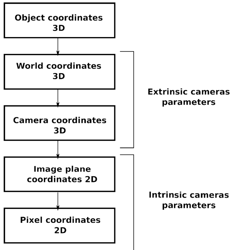
Figure 9.1: World to image coordinate system conversion.
