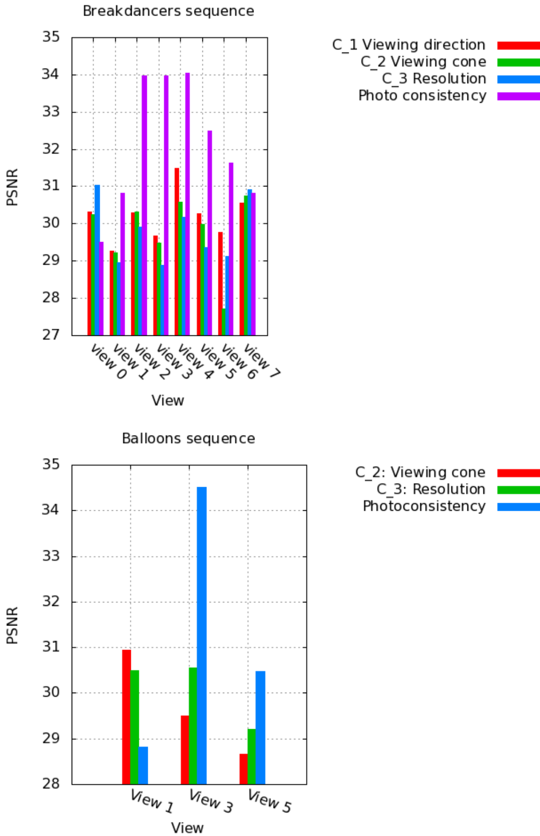
Figure 1.11: PSNR evolution through different views using different criteria for Breakdancers and Balloons sequences.
