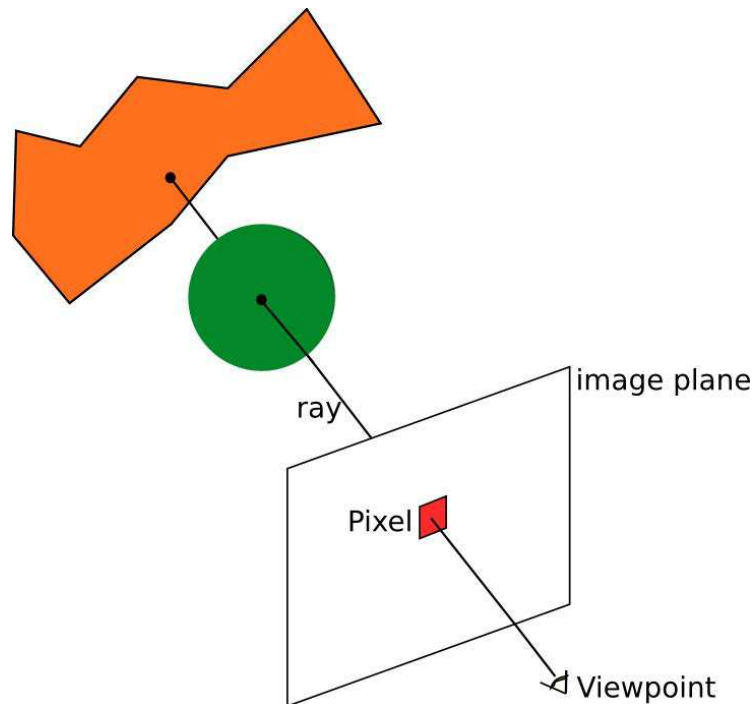
Figure 7.5: Ray casting algorithm for visibility determination. A ray is cast from the viewpoint to each pixel in order to determine the closest object intersected.
