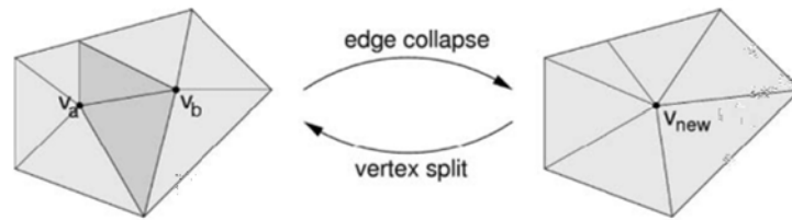
Figure 10.9: Edge collapse operation and its inverse: edge split (image from [Ozaktas and Onural, 2007])
