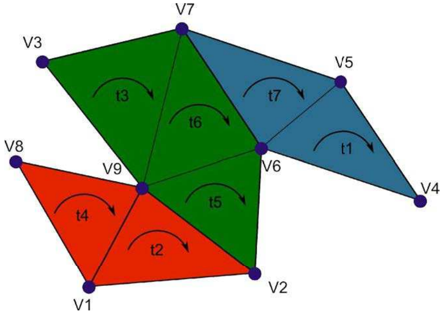
Figure 10.15: Decomposition of mesh connectivity into three triangle fans: TF_1 = \{v_1, v_8, v_9, v_2\} , TF_2 = \{v_9, v_3, v_7, v_6, v_2\} , TF_3 = \{v_6, v_7, v_5, v_4\} .
