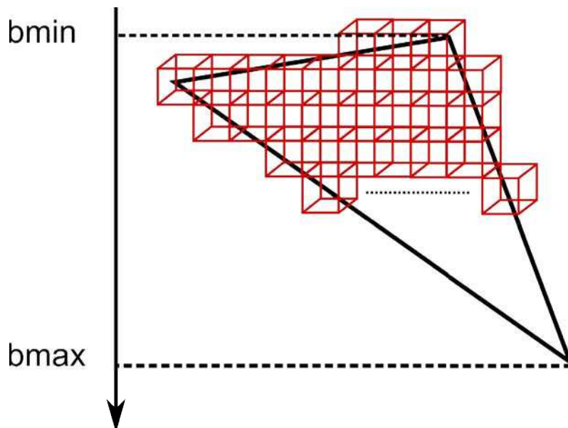
Figure 6.4: Construction of the VMH for a mesh triangle using scanline fill algorithm (See also algorithm 10).
