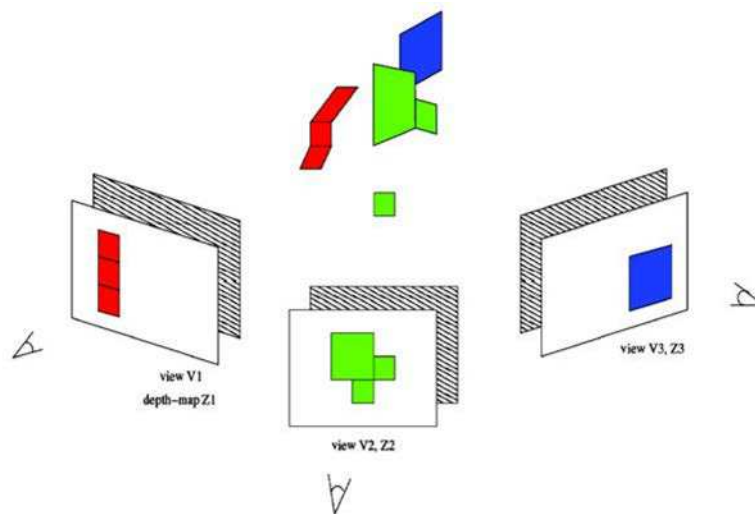
Figure 4.12: Polygon soup representation: a set of 3D polygons. Each 3D polygon is defined by a 2D polygon in one of the acquired views, and by the depth information for each corner of the polygon (image from [Colleu et al., 2010]).
