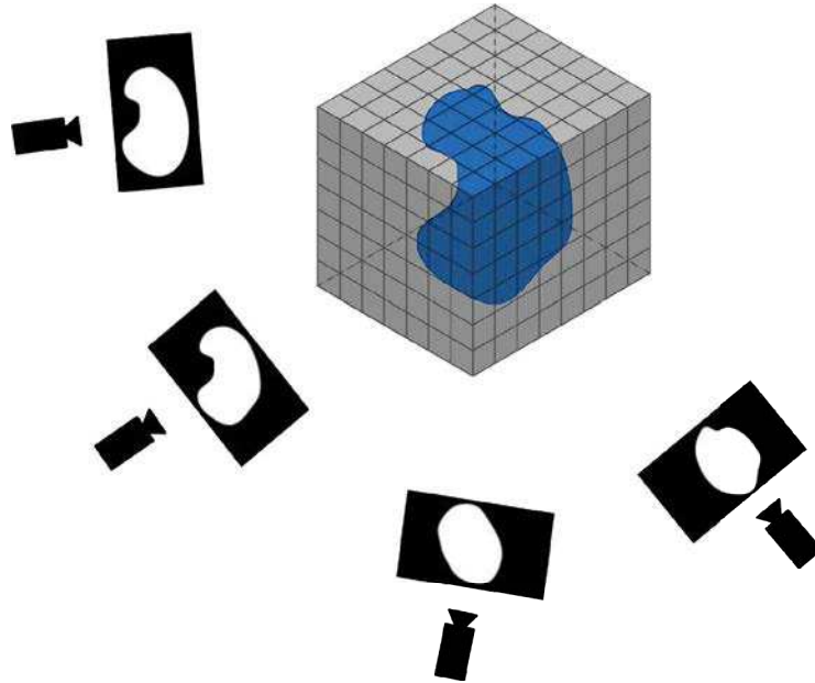
Figure 5.1: Volumetric reconstruction using shape from silhouette technique on a regular grid.
