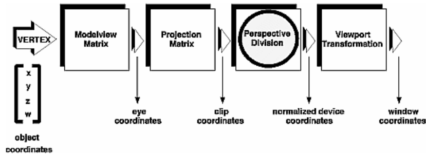
Figure 9.3: OpenGL stages of vertex transformations (image from [Shreiner et al., 2004])
