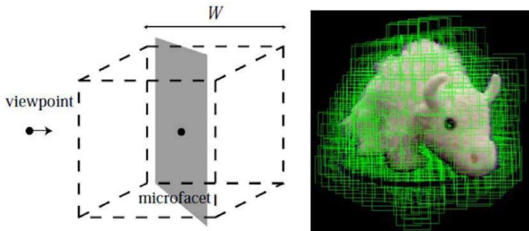
Figure 4.11: Microfacet billboarding. Left: a microfacet is a slice that intersects the center of the voxel and is vertical to the viewing direction. Right: microfacet billboarding result.
