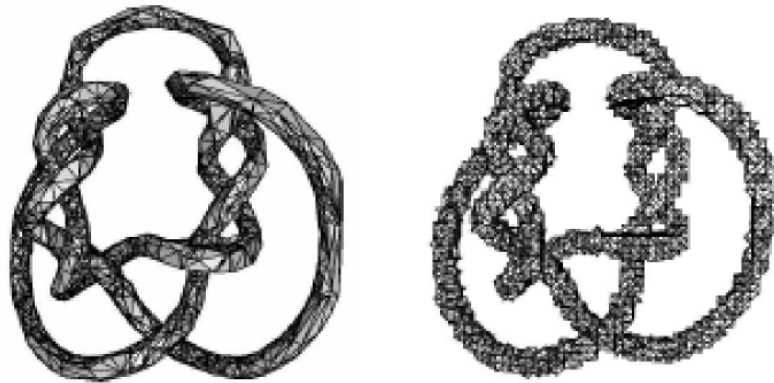
Figure 5.2: Reconstruction example on the knots dataset using tetrahedrons (left) versus regular grid (right) (image from [Boyer et al., 2003]).
