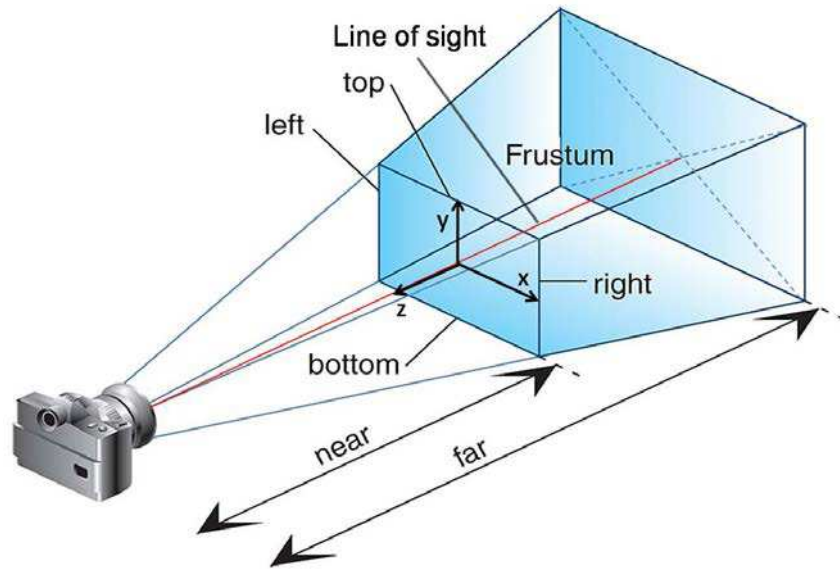
Figure 9.5: Perspective Viewing Volume Specified by glFrustum .
