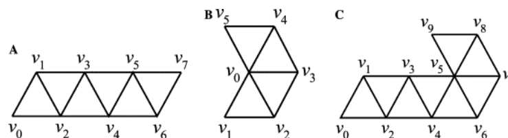
Figure 10.2: A triangle strip (A), a triangle fan (B), and the corresponding generalized triangle strip (C) (image from [Peng et al., 2005])
