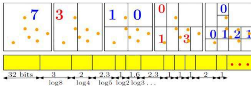
Figure 10.12: Kd-tree decomposition of mesh geometry in 2D (image from [Alliez and Gotsman, 2003]).
