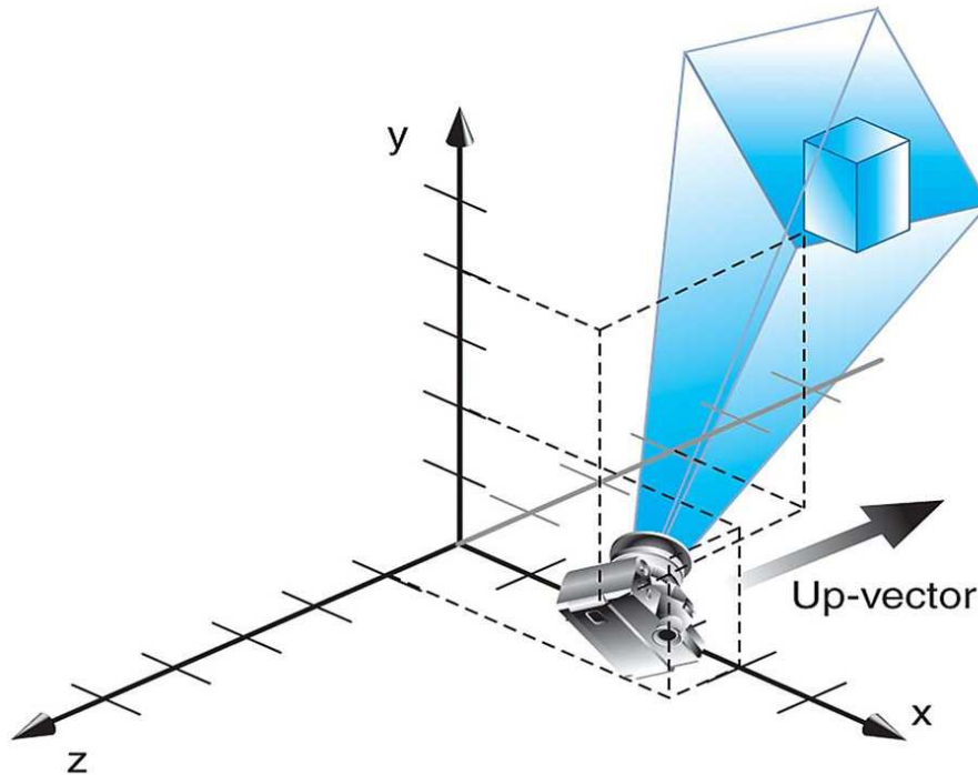
Figure 9.4: Call to gluLookat(4.0,2.0,1.0,2.0,4.0,-3.0,2.0,2.0,-1.0) , the camera position is at (4,2,1) , the reference point is at (2,4,-3) and the view up vector is at (2,2,-1) .
