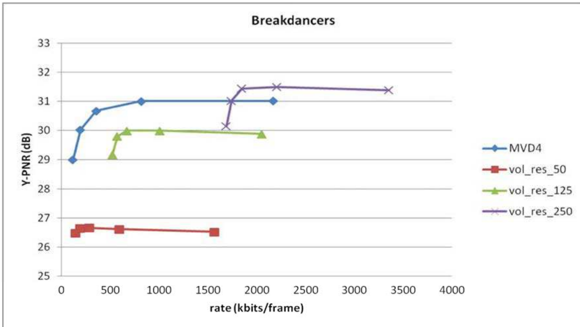
Figure 11.6: Rate/distortion curves for varying volumetric resolutions vs. reference model for breakdancers sequence.
