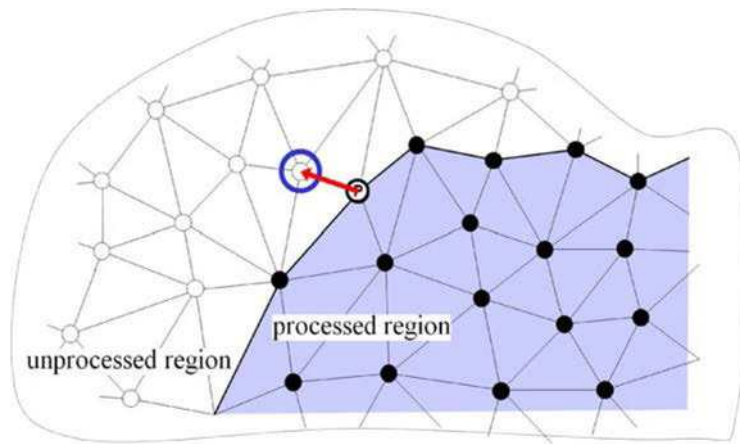
Figure 10.5: Delta prediction rule (image from [Isenburg and Alliez, 2002])
