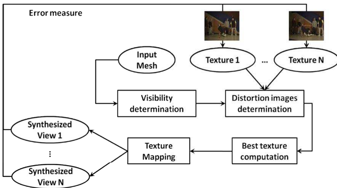
Figure 8.2: The proposed multi-texturing framework.
