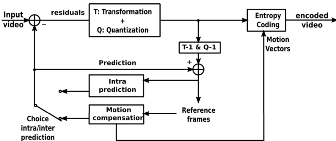
Figure 3.1: Video coding block diagram.
