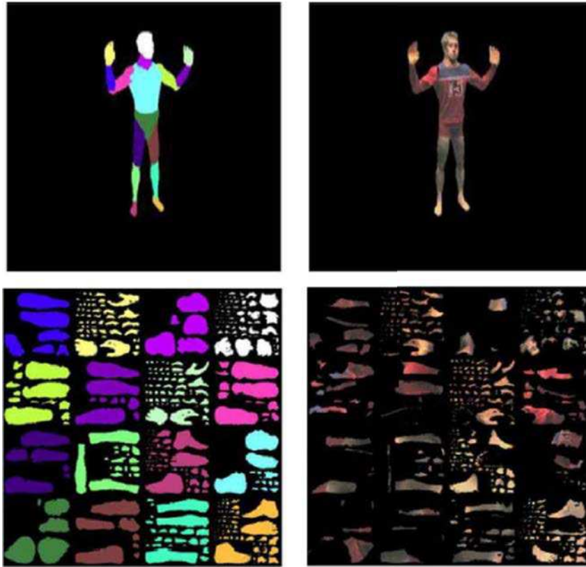
Figure 7.8: Use of texture atlas in the context of 3D Video. From top to bottom and from left to right: mesh partition into charts, textured model, charts are parametrized and then packed, texture atlas [Ziegler et al., 2004].
