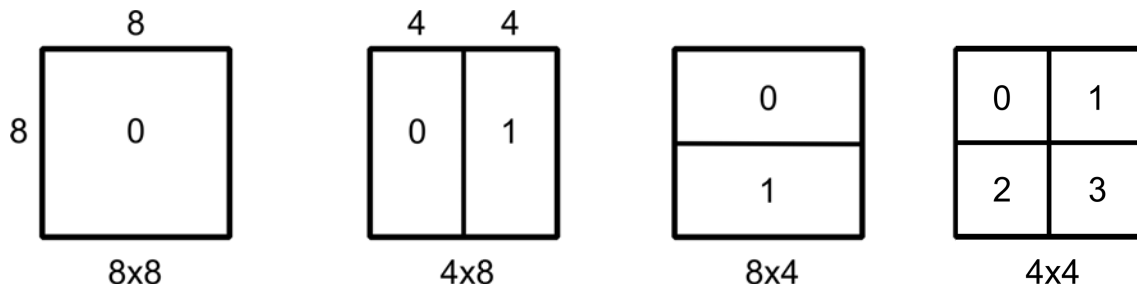
Figure 3.4: Sub-macroblock partitions: 8 \times 8 , 4 \times 8 , 8 \times 4 , 4 \times 4 .
