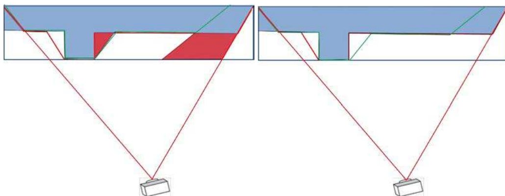
Figure 6.6: Space carving according to the right camera. For the carved volume to be updated, rays are cast from the right camera to its corresponding VMH (left). Red areas are carved. The result of this carving step is shown in the right image.
