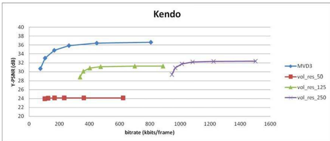
Figure 11.9: Rate/distortion curves for varying volumetric resolutions vs. reference model for kendo sequence.
