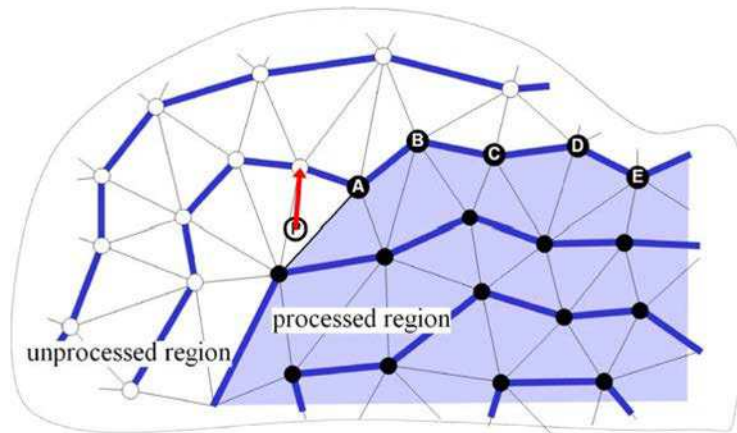
Figure 10.6: Linear prediction rule (image from [Isenburg and Alliez, 2002])
