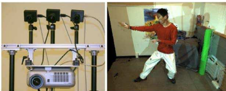
Figure 4.6: Left: the proposed 3D video brick with camera and projector. Right: rendering of the 3D video from new viewpoint [Waschbüsch et al. , 2007a].
