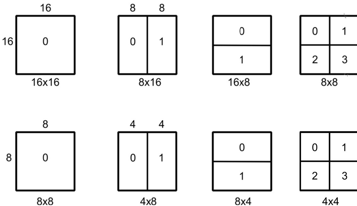
Figure 3.3: Macroblock partitions: 16 \times 16 , 8 \times 16 , 16 \times 8 , 8 \times 8 .
