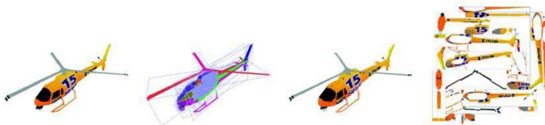
Figure 4.9: Example of a billboard cloud. From left to right: Original model (5,138 polygons), false-color rendering using one color per billboard to show the faces that were grouped, View of the (automatically generated) 32 textured billboards, the billboards side by side (image from [Décoret et al., 2003]).
