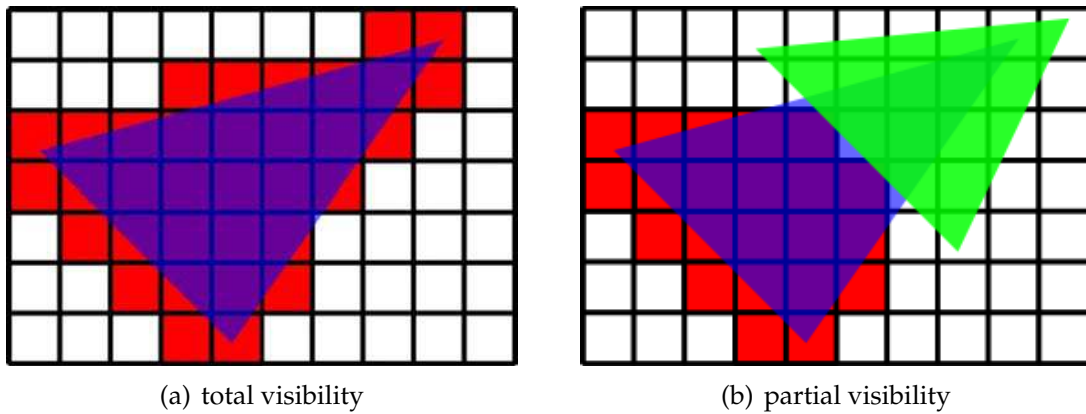
Figure 8.3: Best texture computation. Handling partial/global visibility.
