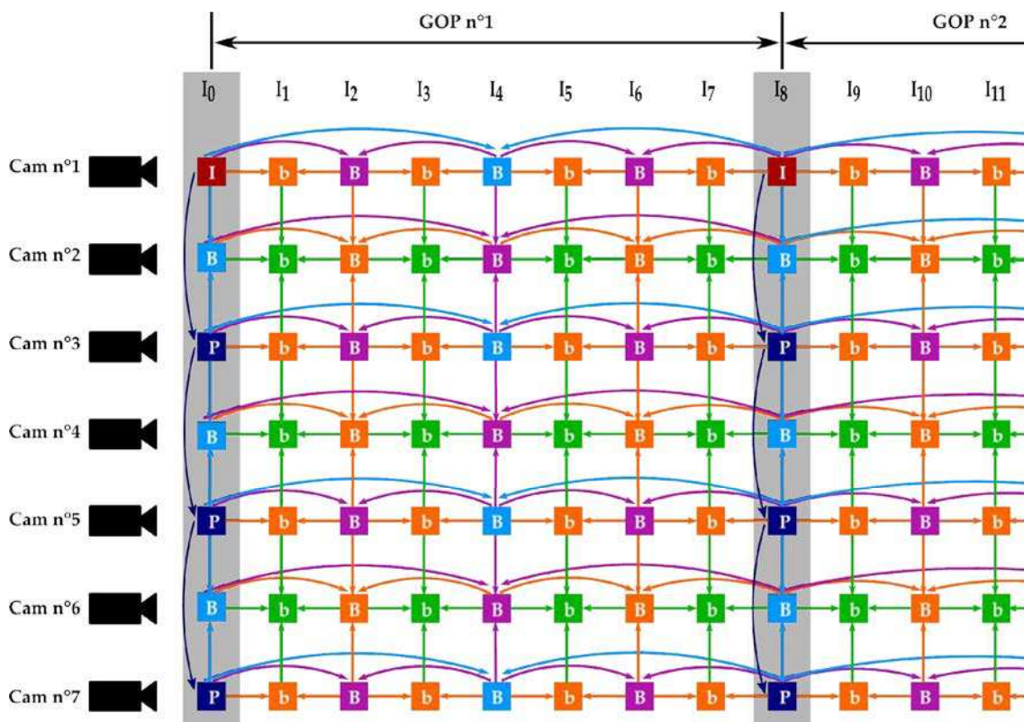
Figure 3.8: Prediction structures in MVC.
