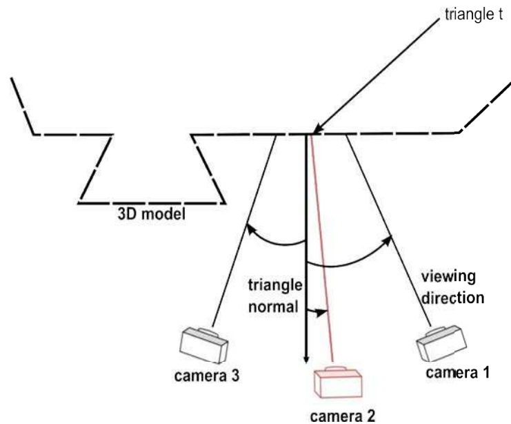
Figure 7.7: Best texture selection using triangle normal criterion.
