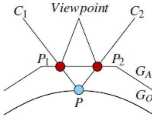
Figure 7.1: Geometric inaccuracies in multi-texturing a 3D model. A point P on the original surface G_O is erroneously projected to 3D-position P_1 from camera C_1 and to 3D-position P_2 from camera C_2 when the approximate geometry proxy G_A is available.(image from [Eisemann et al., 2008])
