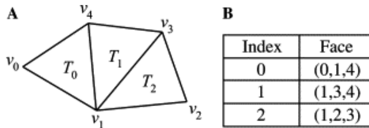
Figure 10.1: The indexed face set method: (A) an example of mesh and (B) its face array (image from [Peng et al., 2005]).
