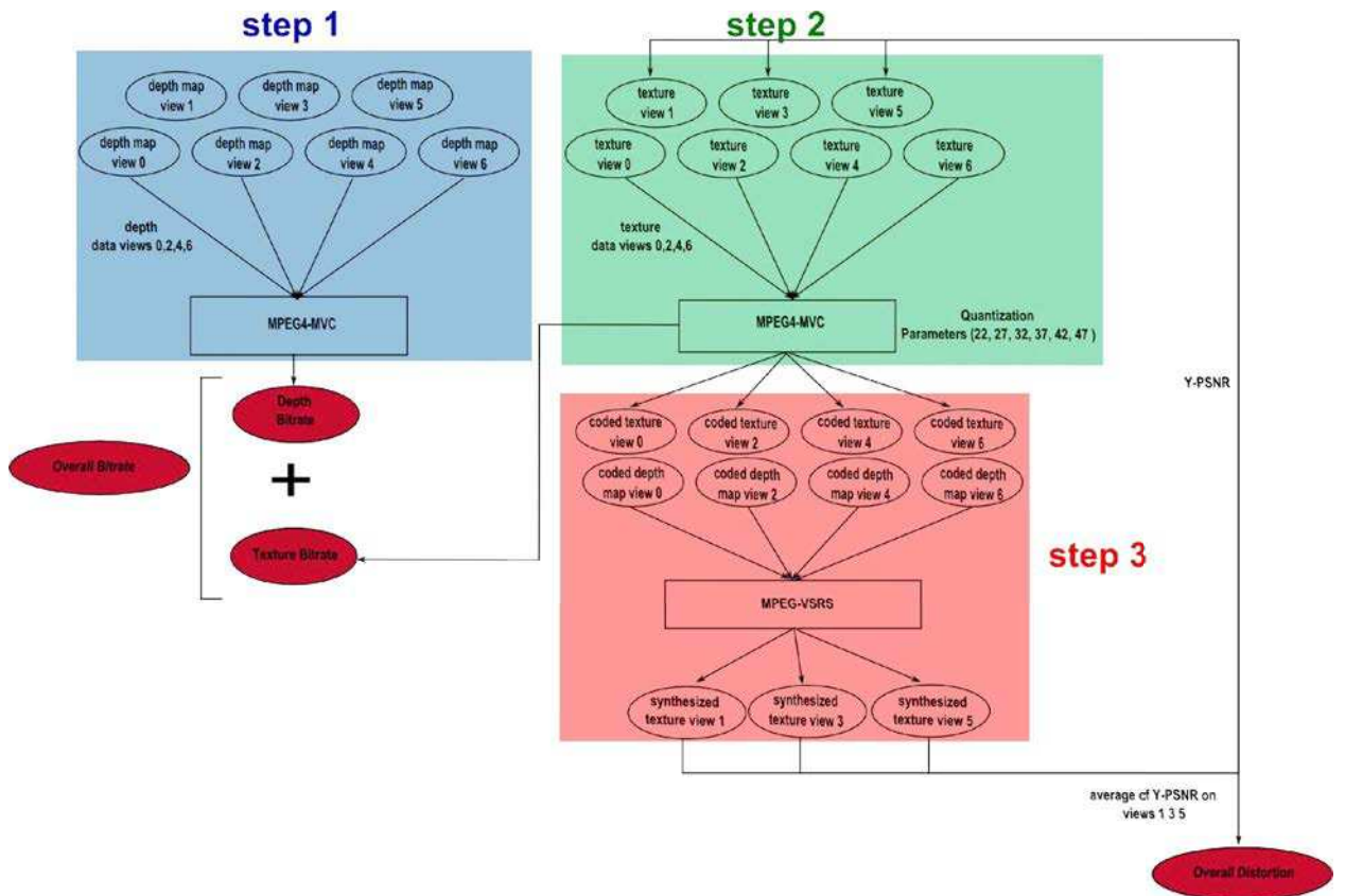
Figure 11.4: Evaluation of the reference model for Microsoft ballet and break-dancers sequences.
