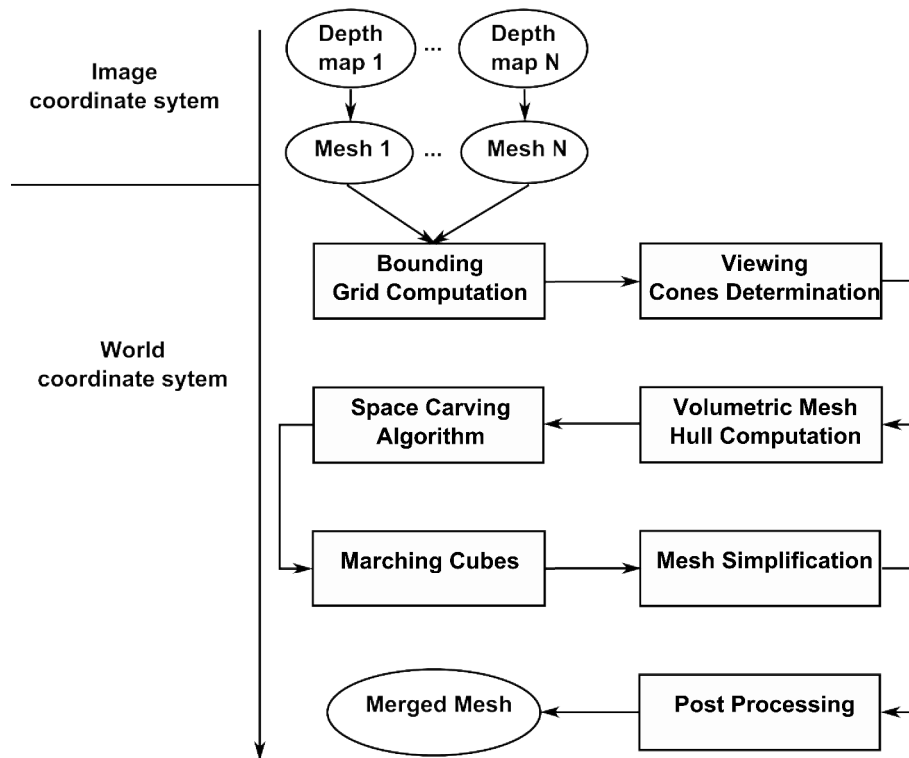
Figure 6.1: Our volumetric framework for depth maps fusion.
