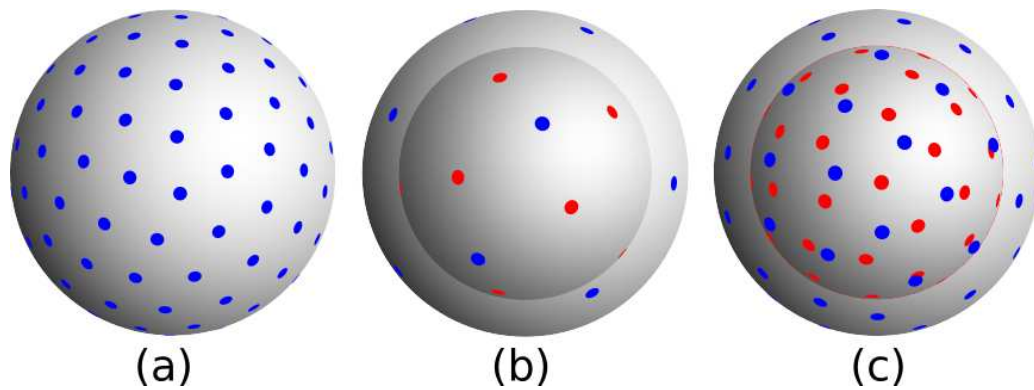
Figure 7.5: Sampling schemes used for validation. (a) A single shell sampling scheme with 64 measurements uniformly spread on one shell at a b-value b = 3000 \text{ s} \cdot \text{mm}^{-2} . (b) A multiple shells sampling scheme with 15 measurements spread on 2 shells at b-values b = 1500, 2500 \text{ s} \cdot \text{mm}^{-2} . (c) A multiple shells sampling scheme with 64 measurements spread on 2 shells at b-values b = 1500, 2500 \text{ s} \cdot \text{mm}^{-2} .
