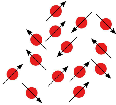
Figure 3.2: Magnetic dipoles, or spins, with different directions.
