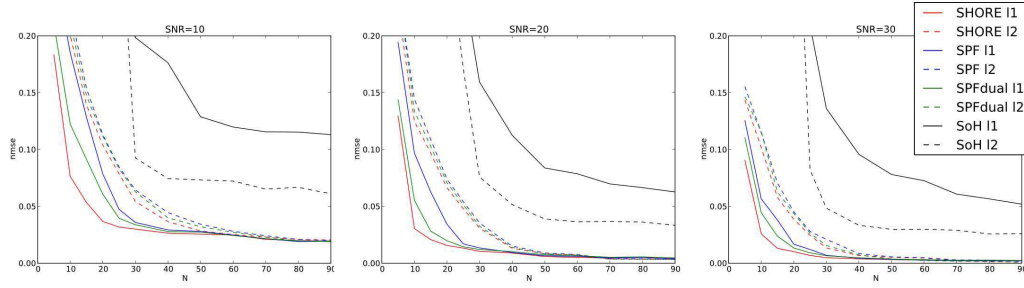
Figure 6.4: NMSE for noisy and synthetic reconstruction with SNR=10 to SNR=30 (left to right). Results for \ell_1 recovery is represented in plain line and results for \ell_2 recovery is represented in dash line. We consider the SPF (in blue), SPFdual (in green), SoH (in black) and SHORE (in red) bases for the reconstruction.
