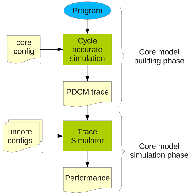
Figure 3.2: Simulation flow for PDCM behavioral core model.
