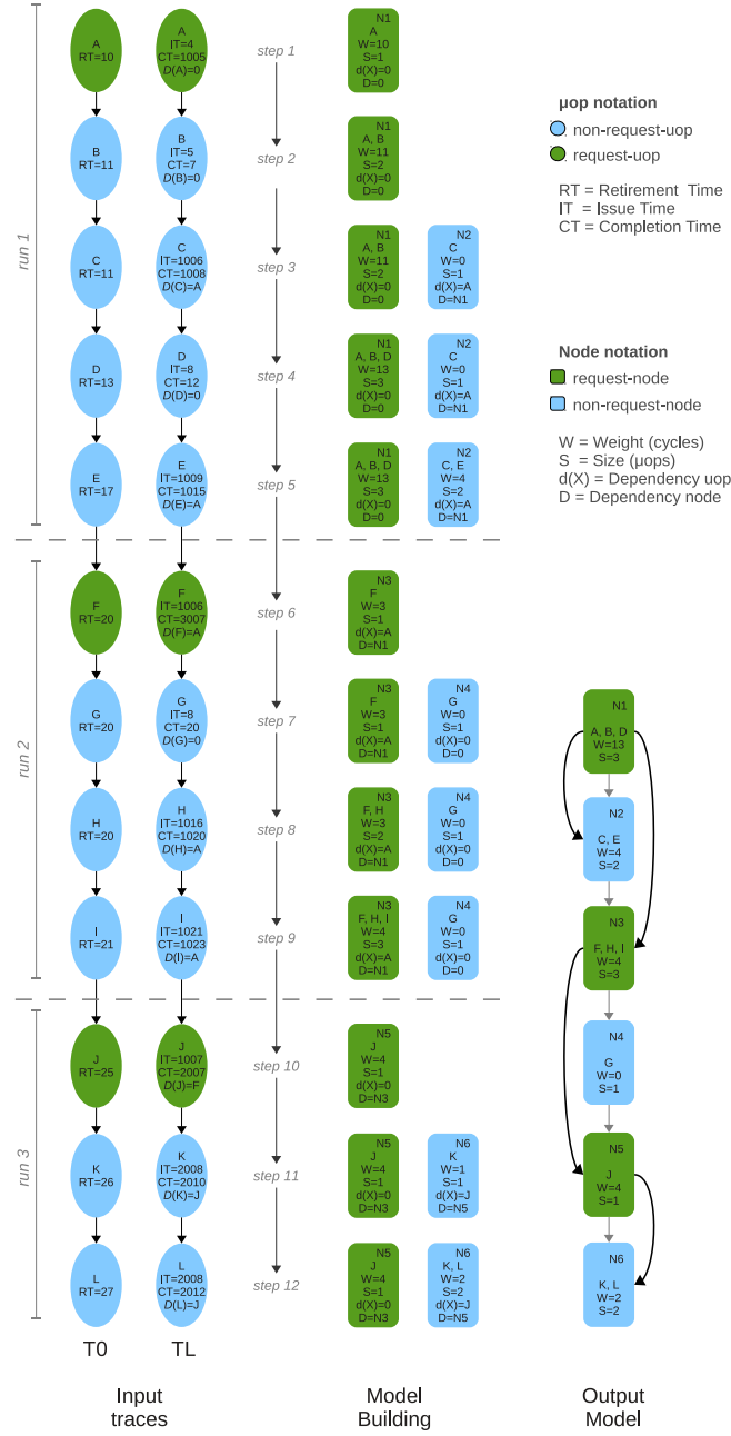
Figure 3.5: Example of BADCO model building: Input traces T0 and TL containing the same 12 dynamic \mu ops in sequential order at the left, \mu op-by- \mu op processing of the traces at the center, and the final BADCO model featuring 6 nodes at the right.
