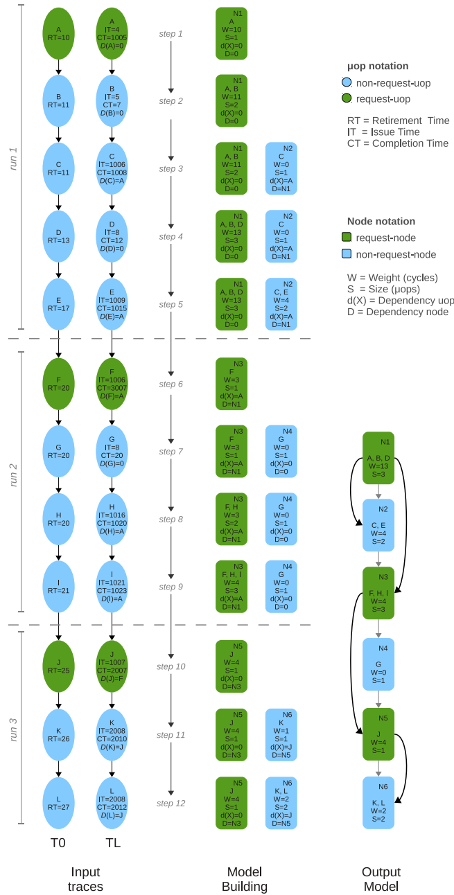
Figure 3.5: Example of BADCO model building: Input traces T0 and TL containing the same 12 dynamic \mu\text{ops} in sequential order at the left, \mu\text{op} -by- \mu\text{op} processing of the traces at the center, and the final BADCO model featuring 6 nodes at the right.
