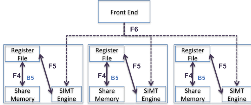
Figure 2.5: Analytical Model of TPC with Data Flow
