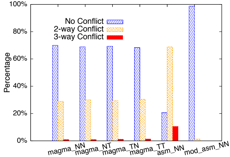
Figure 4.8: Register Conflict of FFMA Instruction
