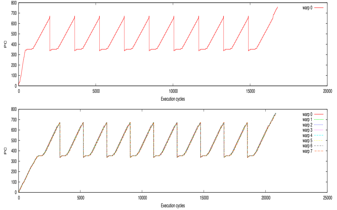
Figure 3.8: PC Trace
