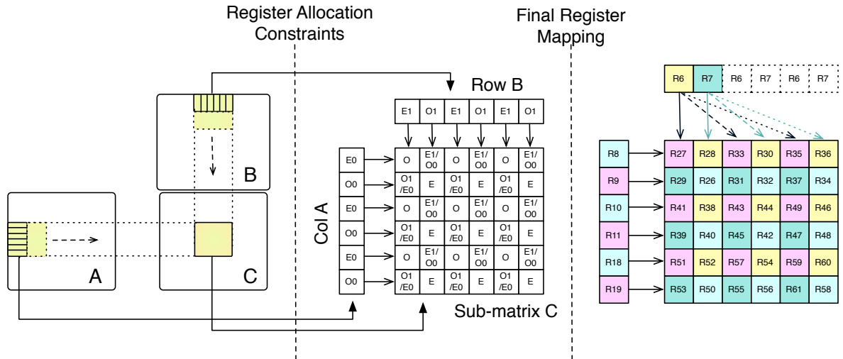
Figure 4.9: Register Allocation
