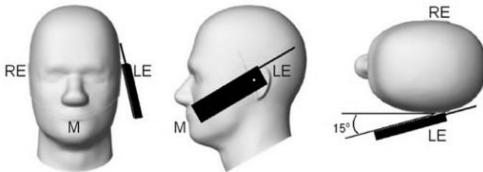
Figure 19 : Configuration Tilt [39]
