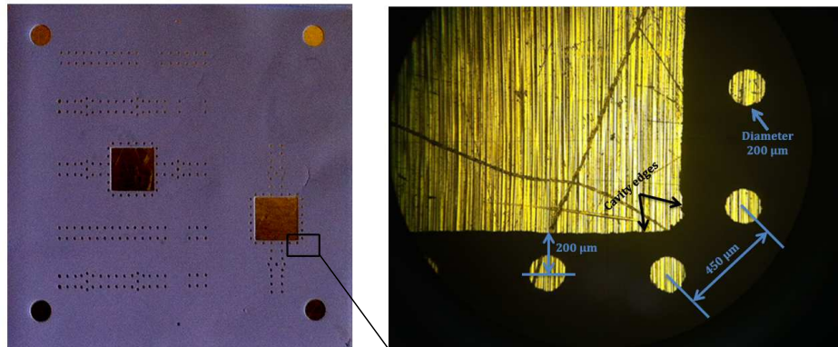
Figure 2.10: 224 drilled vias of a 106 \mu\text{m} ESL41110 tape using ND-YAG laser system. The via diameter is 200 \mu\text{m} , the via pitch is 450 \mu\text{m} and the via to cavity edge distance is 200 \mu\text{m}
