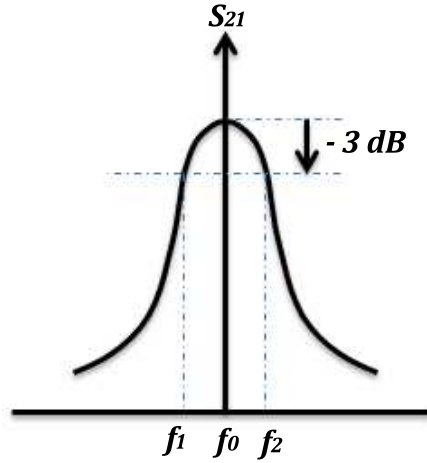
Figure 3.16: The loaded Q factor measurement of ring resonator
