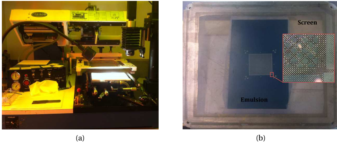
Figure 2.13: Screen printing operations: (a) PRESCO CP-465 machine printer with camera for optical alignment. (b) A 325 screen mesh count of a meshed ground plane with emulsion thickness of 20 \mu m
