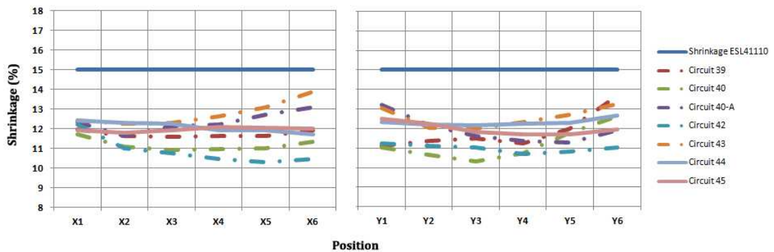
Figure 2.36: Measured shrinkage values of LTCC circuits with cross patterns in x and y directions
