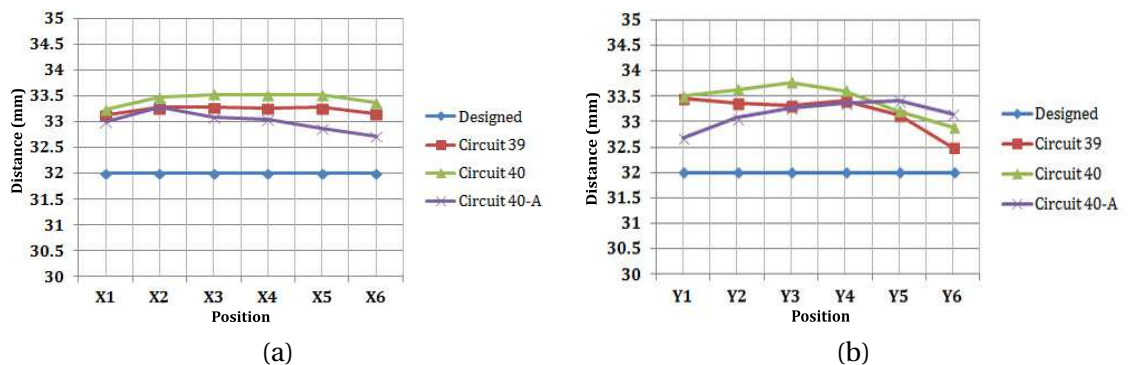
Figure 2.32: Dimensional measurement of the distortion on the fabricated LTCC circuits: (a) Horizontally and (b) vertically
