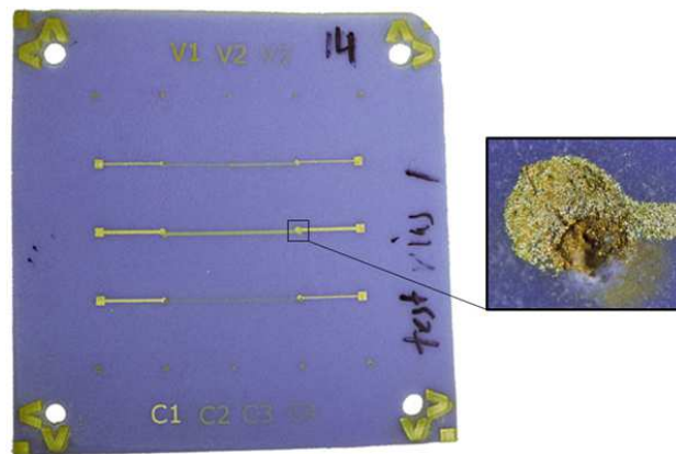
Figure 2.48: Via fill problems: misalignment and incomplete via fill
