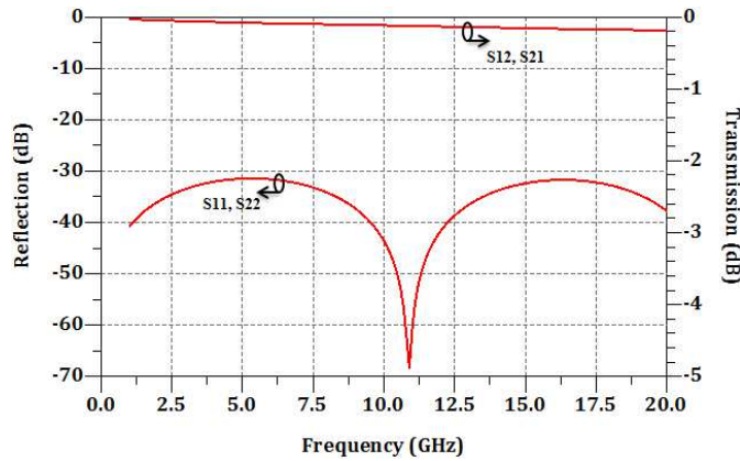
Figure 3.19: S-parameter results of simulated CBCPW line using eight ESL41110 layers
