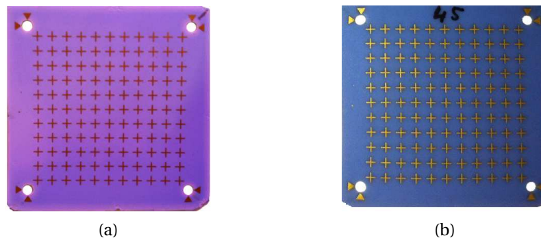
Figure 2.34: Six LTCC layers with cross patterns: (a) Laminated without pin fixture. (b) Fired in the box furnace
