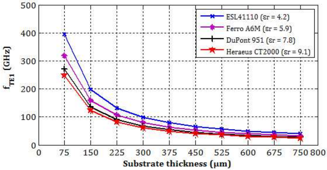
Figure 2.3: Cut-off frequency TE_1 of some commercial LTCC tapes as a function of the substrate thickness
