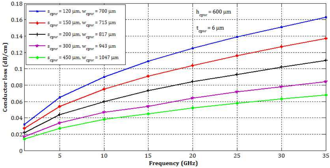
Figure 3.10: Conductor losses of a 50 Ω CBCPW line in ESL41110 substrate with varying spacing of the center conductor to top ground planes
