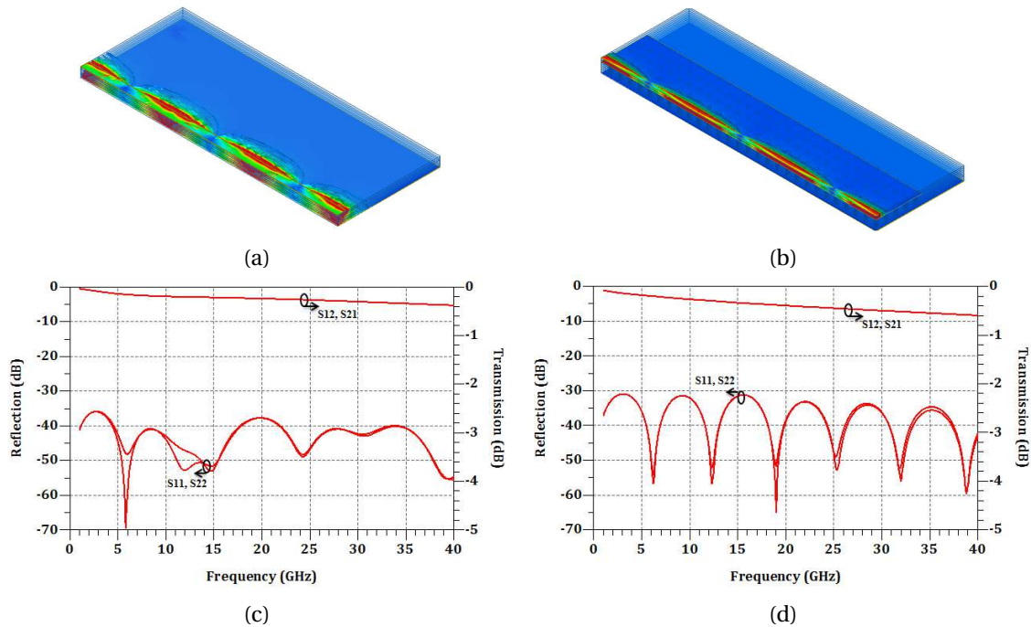
Figure 3.18: HFSS simulation of two 50 Ω microstrip lines: (a) E-field at 20 GHz in microstrip line of "Line 1" on six ESL41110 layers. (b) E-field in microstrip line of "Line 2" on eight ESL41110 layers with intermediate ground plane. (c) S-parameter results of "Line 1". (d) S-parameter results of "Line 2"
