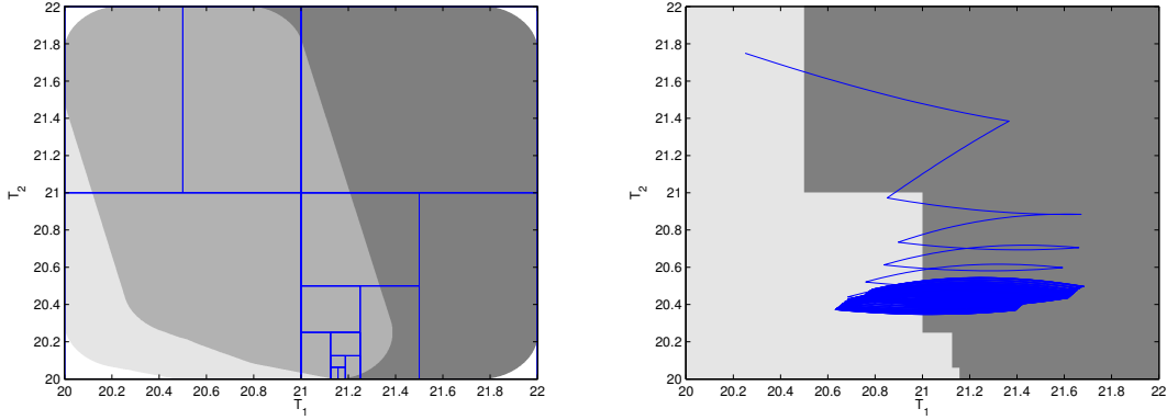
Figure 3.5: Set-valued map \mathcal{K} : [\mathbb{R}^2]_\eta \cap Y_s \rightarrow 2^P (white: \emptyset , light gray: \{1\} , medium gray: P , dark gray: \{0\} ). The number of elements in [\mathbb{R}^2]_\eta \cap Y_s is about 1 million. In blue, we represented the partition used for the representation of \mathcal{K}_d , a determinization of \mathcal{K} ; the resulting tree structure has only 27 nodes (left). Determinization \mathcal{K}_d of the map \mathcal{K} (light gray: 1, dark gray: 0). In blue, a trajectory of the switched system controlled using the controller \mathcal{C}_d = \mathcal{K}_d \circ Q_\eta (right).
