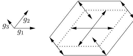
Figure 5.1: Example of a zonotope with three generators
