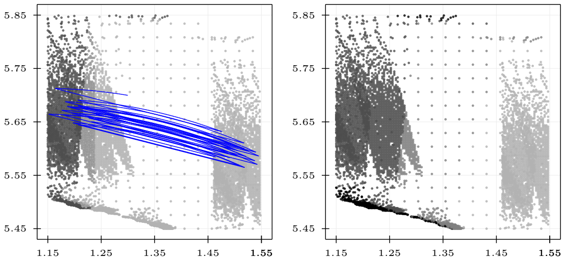
Figure 3.7: The maximal lazy safety controller for T_{\tau,\eta}^N(\Sigma) . Mode map (left) - dark gray : mode 1, light gray : mode 2, medium gray : both modes are enabled; Duration map (right) - light gray : 4, medium gray : 2, dark gray : 1, black : 0.5.
