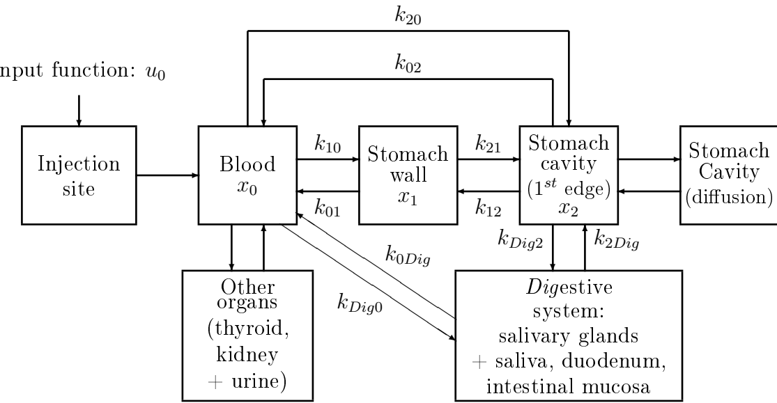
Figure 6.2: Complete compartmental model describing the studied problem: kinetic of iodide uptake in the murine stomach.
