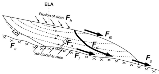
Fig. 10. A sketch of the clast flux in a glacial environment. The clasts supplied by hillslope erosion ( F_n ) are either incorporated in the glacier ( F_d ) or delivered to the lateral or frontal moraines ( F_m ). The sediment load of a subglacial stream ( F_s ) is a mixture of two components: erosion at the base of the temperate glacier ( F_t ) and clasts supplied by hillslope erosion and incorporated in the glacier ( F_u ). Erosion at the base of the cold glacier ( F_c ) and upward transport from base to surface ( F_u ) were found to be very low within the Bossons glacier (see section 4 in the main text).
