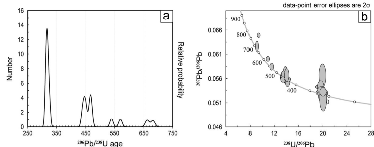
Fig. 4. Zircons of the metamorphics of the Bossons watershed: (a) ^{206}\text{Pb}/^{238}\text{U} age distribution for 26 zircons of Gn1 sample; (b) Zircon ages in a Tera and Wasserburg (1972) diagram (Gn2 Sample).
