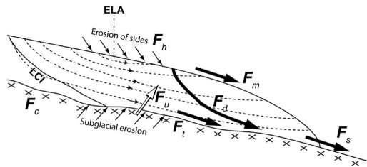
Fig. 10. A sketch of the clast flux in a glacial environment. The clasts supplied by hillslope erosion ( F_n ) are either incorporated in the glacier ( F_d ) or delivered to the lateral or frontal moraines ( F_m ). The sediment load of a subglacial stream ( F_s ) is a mixture of two components: erosion at the base of the temperate glacier ( F_t ) and clasts supplied by hillslope erosion and incorporated in the glacier ( F_u ). Erosion at the base of the cold glacier ( F_c ) and upward transport from base to surface ( F_u ) were found to be very low within the Bossons glacier (see section 4 in the main text).
