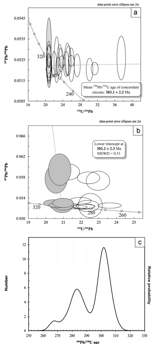
Fig. 5. Zircon age signature of granite. (a) Concordia diagram for in situ sample of granite (Gr sample); (b) Mer de glace basal moraine: Tera and Wasserburg (1972) diagram; (c) Mer de Glace basal moraine: ^{206}\text{Pb}/^{238}\text{U} age distribution for 22 zircons.
