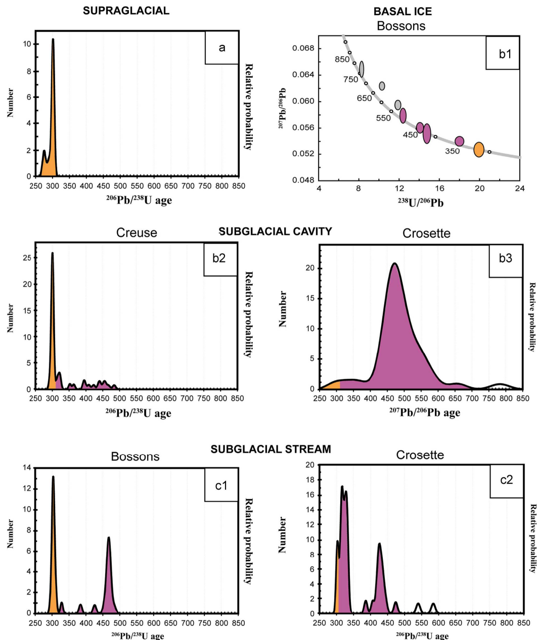
Fig. 7. Detrital zircons from the Bossons glacier (yellow for granite and purple for gneiss or metamorphics). These results, weighted by a Zr content ratio are used to estimate the lithologic distribution of the fine-grained fraction in Fig. 8: (a) Supraglacial load (Pyramids right sample; 12 dated zircons); (b) Basal ice. (b1) "Bossons ice" sample (8 zircons), (b2) "Creuse basal moraine" (44 zircons); (b3) "Crosette Cavity" sample (34 zircons); (c) Outlets of subglacial streams: (c1) Bossons stream (39 zircons) and (c2) Crosette stream (44 zircons). (For interpretation of the references to color in this figure legend, the reader is referred to the web version of this article.)
