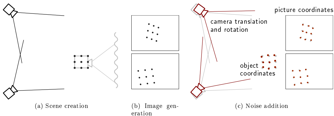
Figure 3.3: First three simulation steps.
