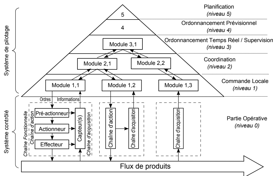
FIGURE 1.4 – Architecture CIM
