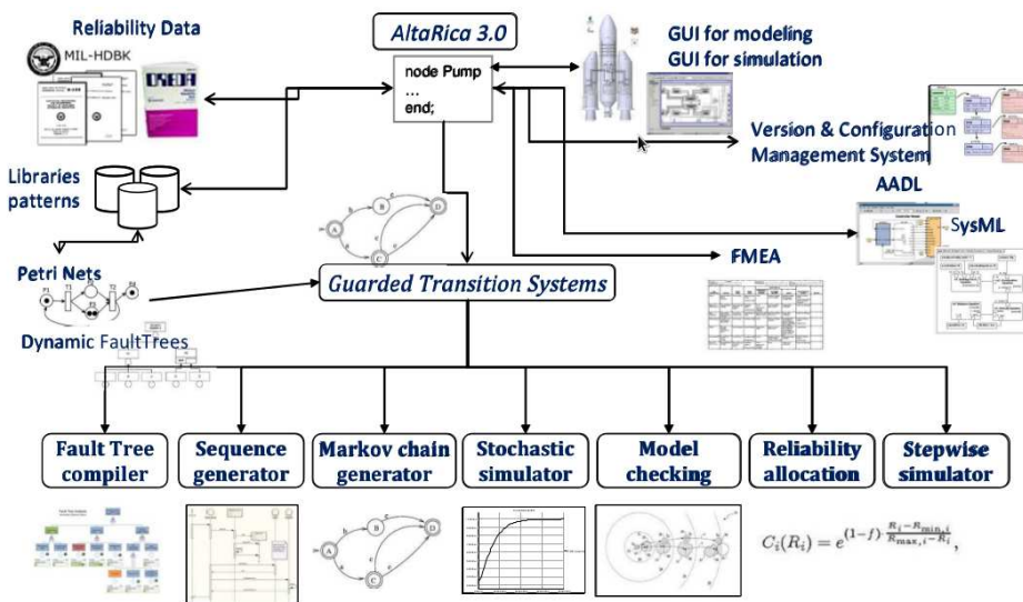
Figure 1.20 – Architecture du projet ALTARICA [PR12]
