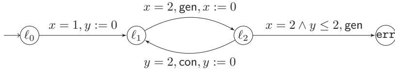
Figure 2.2: The timed automaton \mathcal{A}^1 modelling the producer-consumer system of Fig. 2.1 instantiated for N = 1 . The transition from \ell_0 to \ell_1 models an offset of 1 time unit given for the consumer.
