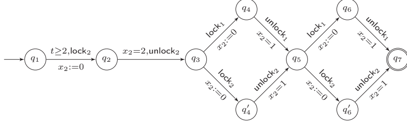
Figure 2.6: Timed automaton \mathcal{P}_2 modeling Process 2.
