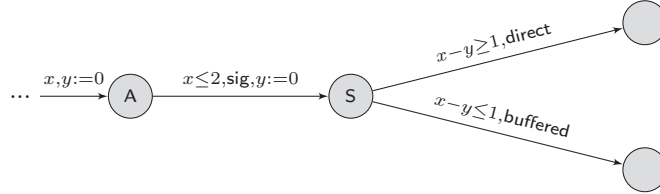
Figure 6.2: Timed automaton \mathcal{A}^3 .
