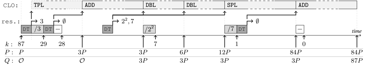
Figure 4.11: MBNS recoding and scalar multiplication illustration for k = 87 .
