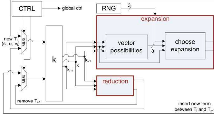
Figure 2.3: Architecture of the on-the-fly recoding unit with random DBNS chains.
