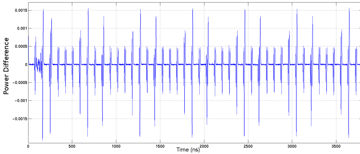
Figure 3.4: Difference between mean traces for 2 keys.
