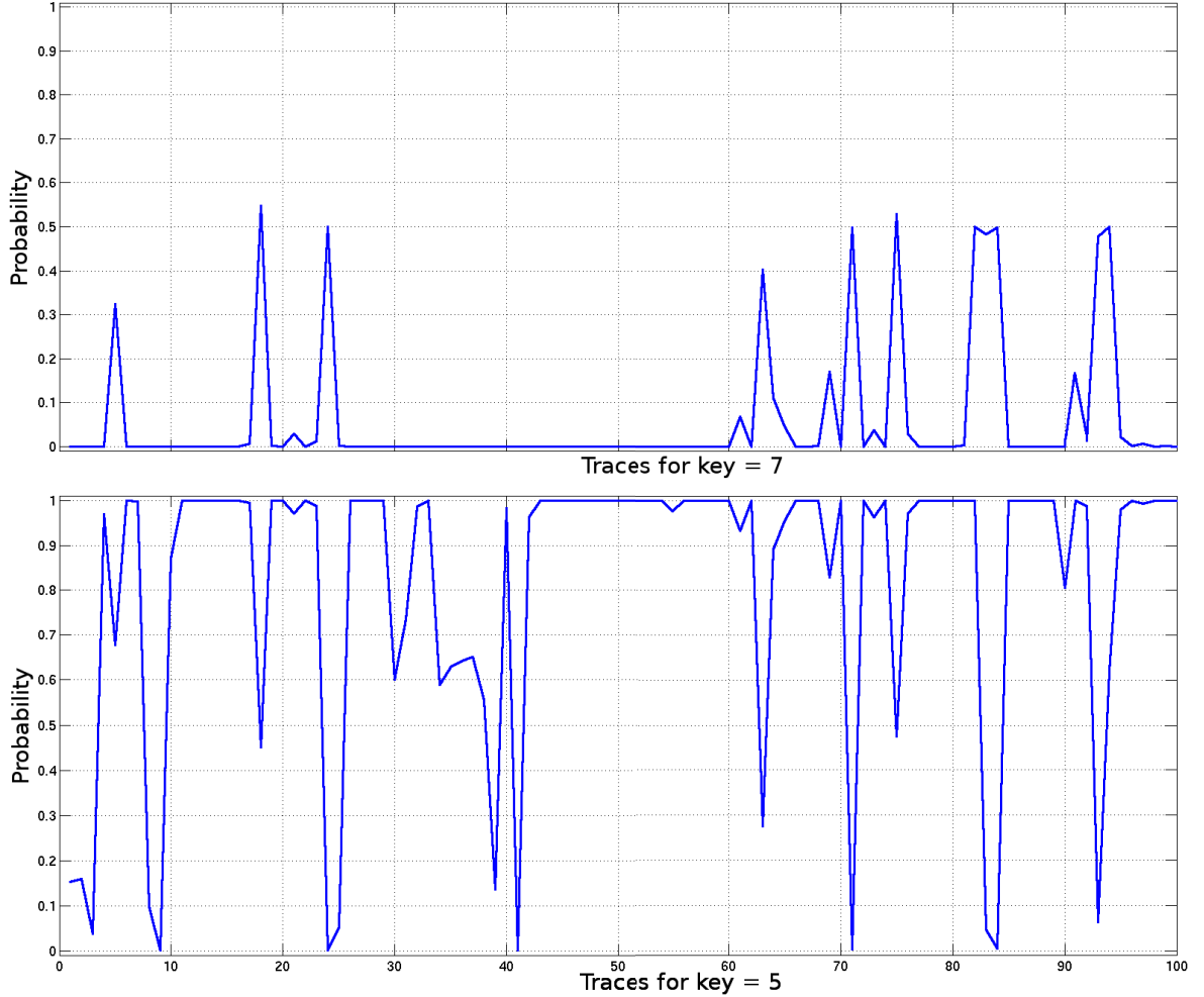
Figure 3.7: The probabilities pr(k^{(i)}|t) for each trace t with k^{(i)} = 7 and k^{(i)} = 5 .
