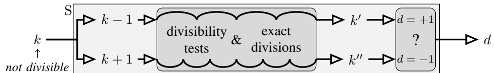
Figure 4.13: Principle of the min selection function.
