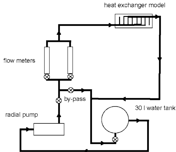
Fig. 1 Hydraulic loop
