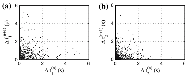
Fig. 17 (n + 1) th lifetime of mode (a) f_1 , (b) f_2 with respect to the n th one
