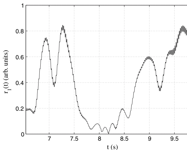
Fig. 12 Radius in the phase space, defined as r(t) = \sqrt{(X_1(t) - \bar{X}_1)^2 + (X_2(t) - \bar{X}_2)^2} , versus time, here for the mode f_1 . Small amplitude, high frequency oscillations at 2f_1 , can be seen on the slowly varying radius dynamics
