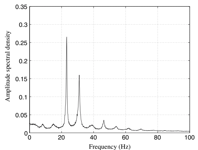
Fig. 2 Square root of the power spectral density, normalized to 1, of the LDV time series s(t) . Incoming flow velocity U_e = 2.09 m/s, aspect ratio R = 2 . Two main modes emerge at f_1 = 23.2 Hz and f_2 = 31.0 Hz. The other peaks are nonlinear combinations of f_1 and f_2
