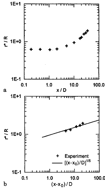
Fig. 3. a Axial variation of the radius of the wake from the trailing edge of the body; b axial variation of the radius of the the wake from its virtual origin
