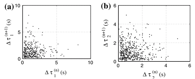
Fig. 18 (n + 1) th cycle of rising/disappearance of mode (a) f_1 , (b) f_2 in the signal with respect to the n th one
