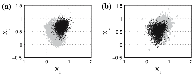
Fig. 20 Poincaré section (\Pi) , as defined by Eq. 7. a Dark points are the (\Pi) intersections with mode f_1 , grey points are the (\Pi) intersections with mode f_2 , b colours are inversed with respect to the previous case
