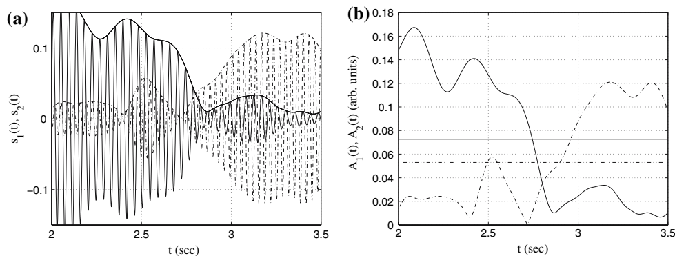
Fig. 5 Amplitudes A_1(t) (solid line) and A_2(t) (broken line) of modes f_1 and f_2 in signals s_1(t) and s_2(t) , a with, or b without, the carrier. The threshold amplitudes \bar{A}_1 and \bar{A}_2 are plotted as horizontal solid and broken lines, respectively, in b
