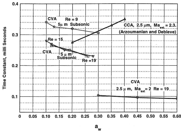
FIG. 2. Measured time constants of the hot wires at different overheated values ( a_w ).
