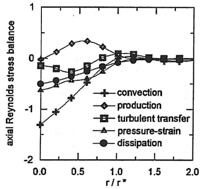
Fig. 9 Axial Reynolds stress balance.
