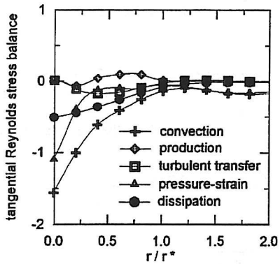
Fig. 11 Tangential Reynolds stress balance.
