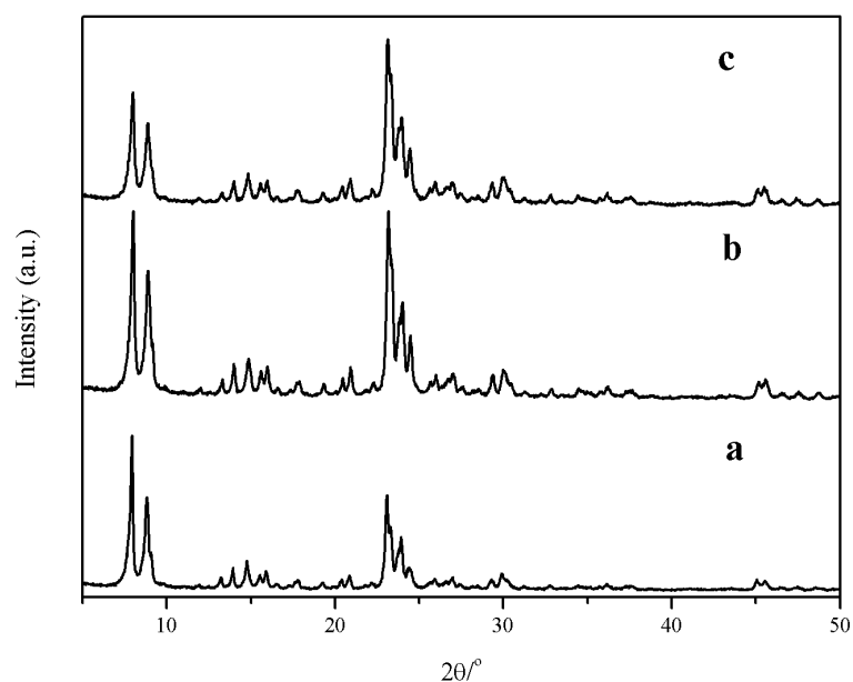
Figure 12. XRD patterns of the hierarchical micro/mesoporous ZSM-5 prepared by use of the C/SiO 2 composite with 18 wt% carbon content and with the Si/Al ratios of (a) 83, (b) 29 and (c) 16.
