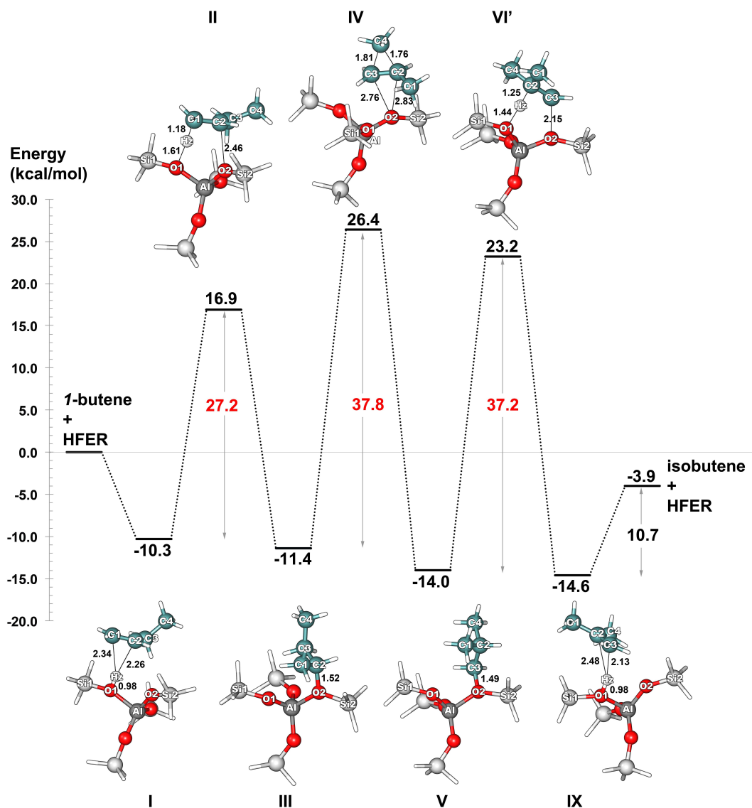
Figure 33. The reaction energy profile of the 1-butene skeletal isomerization determined for the 5T H-FER zeolite model by optimization calculations at the MP2/6-31g(d,p) level of theory. Geometrical parameters and energies are in Å and kcal/mol, respectively.
