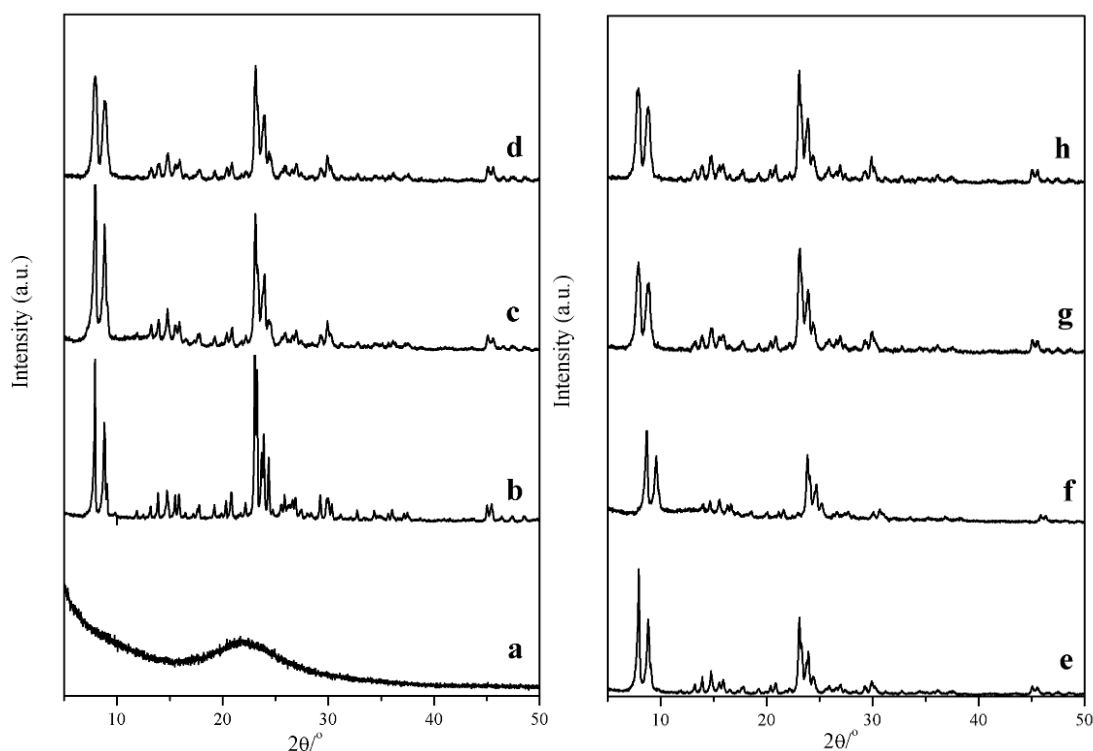
Figure 6. XRD patterns of (a) raw silica gel, (b) the reference zeolite sample (conventional ZSM-5, ALSI-PENTA Zeolithe GmbH (APZ)), (c) 0% carbon-ZSM-5, (d) 5% C_2H_2 -60 min-ZSM-5, (e) 5% C_2H_2 -120 min-ZSM-5, (f) 10% C_2H_2 -120 min-ZSM-5, (g) 5% C_3H_8 -120 min-ZSM-5, and (h) 10% C_3H_8 -120 min-ZSM-5.
