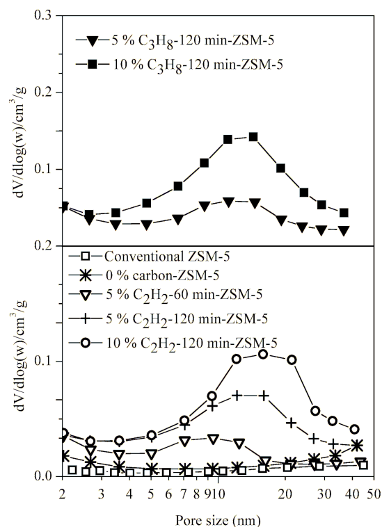
Figure 10. Size distribution of the mesopores of the synthesized zeolite samples calculated from the adsorption branch of the isotherm.
