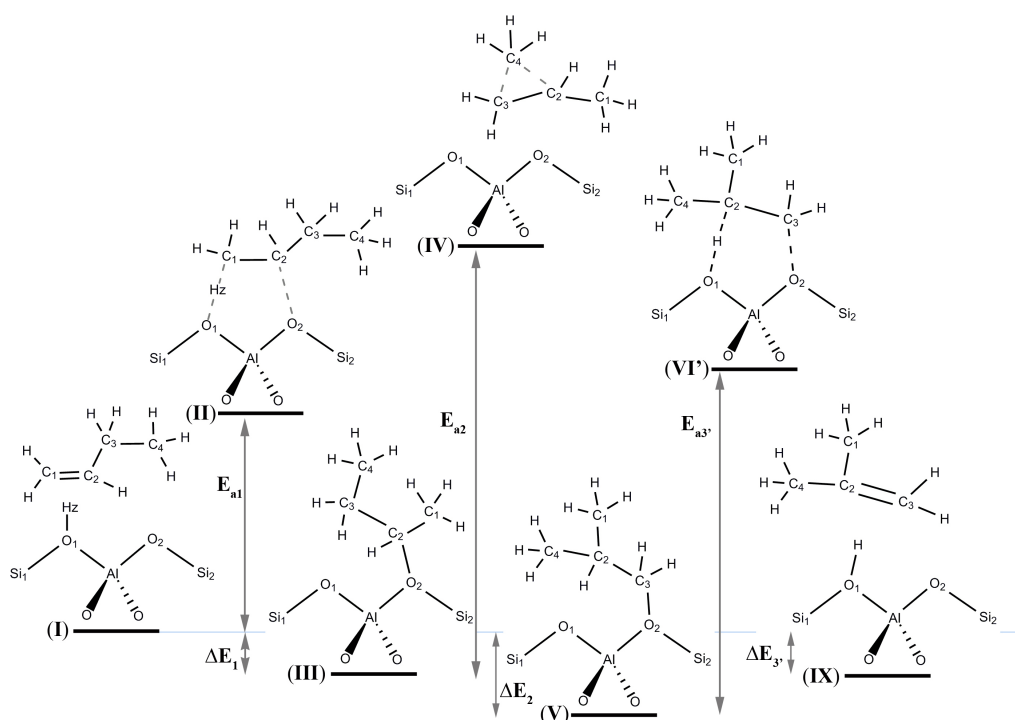
Scheme 6. Monomolecular mechanism for the skeletal isomerization of I -butene to isobutene using the 5T model.
