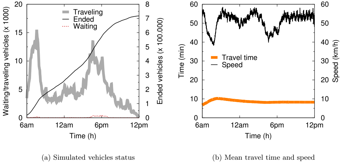
Figure 3.10: Final TAPASCologne dataset. Traffic features over time
