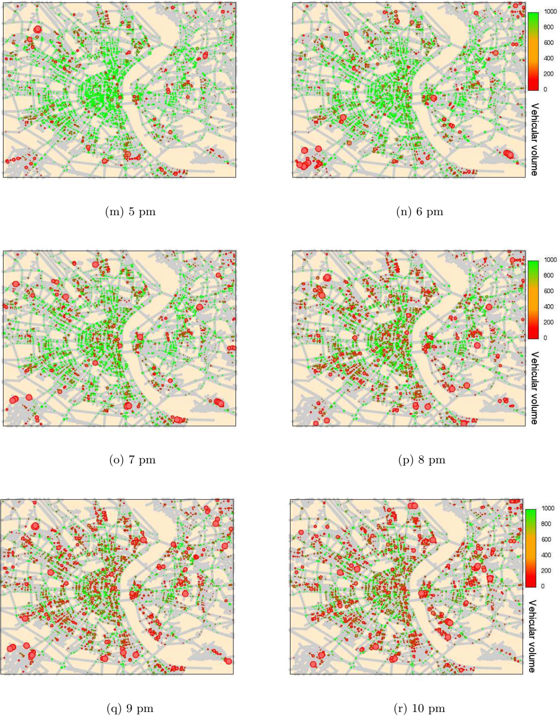
Figure 5.19: Road network: Spatiotemporal distribution of order-2 prediction error and vehicular volume (5 pm to 10 pm)
