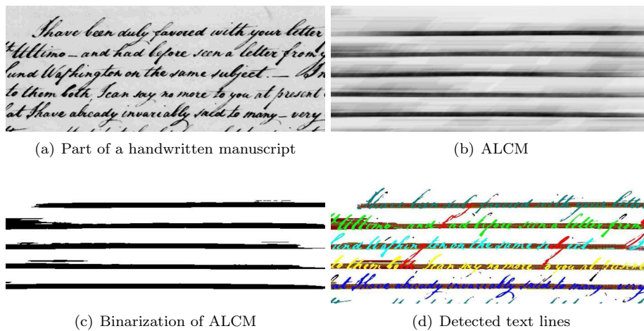
Figure 2.10: Text line detection method in [87] using adaptive local connectivity map.
