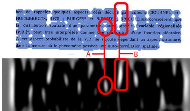
Figure 4.13: This figure displays two types of error that frequently occur in the results of text region detection. They happen when there are gaps between words. If the gap is located in the middle of the text region, it appears as holes A and if it exists near the border of the text region, it causes penetrations B . Both problems can be fixed in the post-processing stage.
