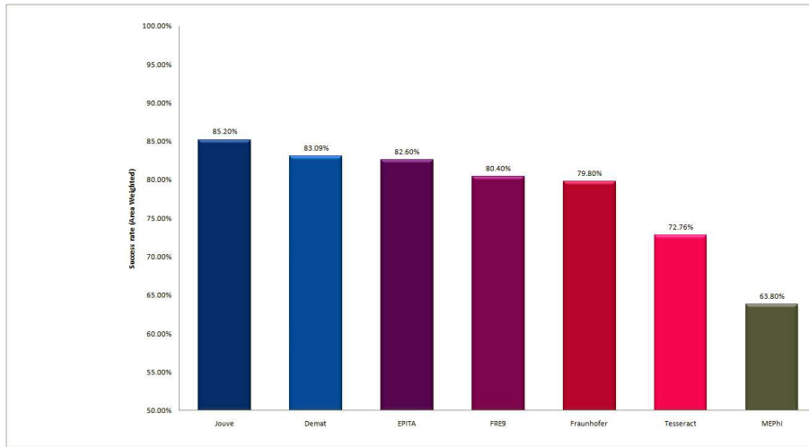
Figure 6.3: Updated results reported in [4] based on scaled estimates. In this figure, the results from our method (Demat) and Tesseract-OCR are added based on scaled estimates by using results of EPITA as a reference.
