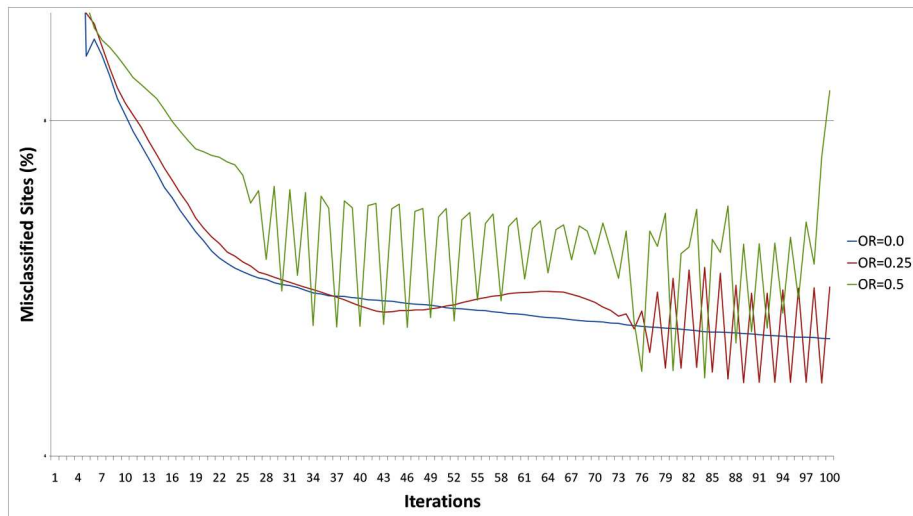
Figure 4.17: This figure shows the evolution of training error rate with 3 different overlapping ratios.
