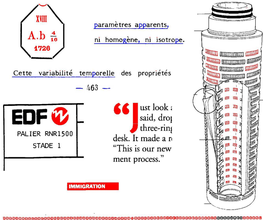
Figure 3.7: Some of the misclassified components gathered from our own documents. Black components are labelled correctly. Red components should have been assigned a graphics label but they are incorrectly labelled as text. Blue components on the other hand have text label in ground-truth, however they are misclassified as graphics.
