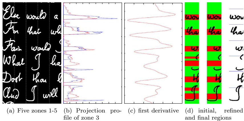
Figure 2.13: Steps for locating text line separators in part of document image. [75]
