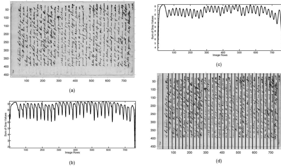
Figure 2.9: Images [62] show line segmentation steps. a A rotated image. b Vertical projection profile of the rotated image. c Smoothed version of the vertical projection profile. d Detected text line separators by detecting peaks in the smoothed projection profile.
