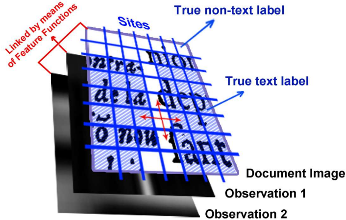
Figure 4.2: This figure shows our two-dimensional conditional random fields model. Blue lines represent the boundaries between site. We divide the document image into rectangular blocks with equal heights and equal widths. The label on each site depends on the label of sites in its vicinity and observations defined for that site. Sites depend on observations by means of feature functions. The ground truth label for each site is also available for the purpose of training and evaluation. Note that the area that is shown on the image is part of a document that shows text lines from the main text and part of a side note. Width and height of sites in this image are not correct according and are shown for visualization purposes only.
