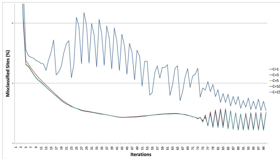
Figure 4.18: This figure displays the number of misclassified sites per iteration for 5 experiments with different maximum number of ICM cycles.
