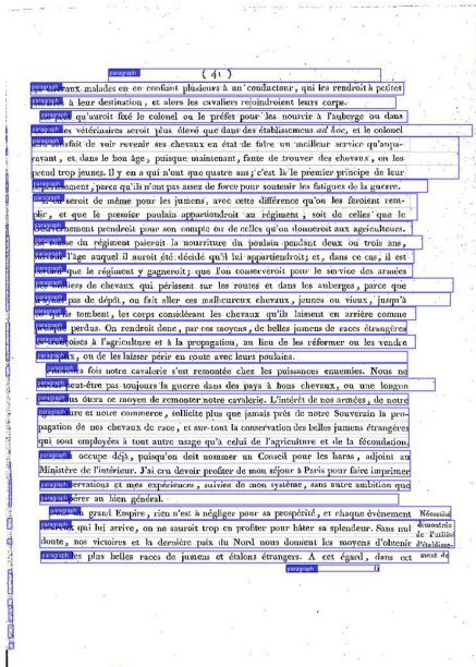
(a) Tesseract-OCR
