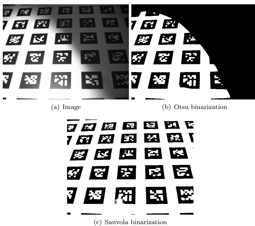
Figure 3.1: When dealing with low quality documents or documents that are captured in bad lighting condition, Sauvola's binarization method is preferable to Otsu's binarization. Image is from [11]
