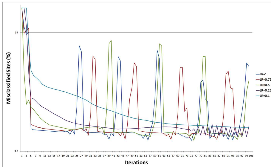
Figure 4.16: This figure shows the evolution of training error rate with 5 different learning rates. All other parameters remain the same.
