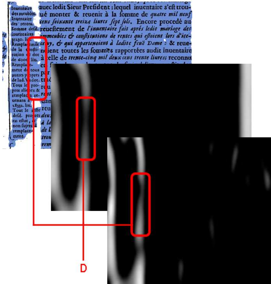
Figure 4.15: This figure illustrates a problem when side notes are very close to main text and the main text is slightly slanted. In such situation, Gabor filters are not able to capture the small gap between side notes which cause both text region to be merged.
