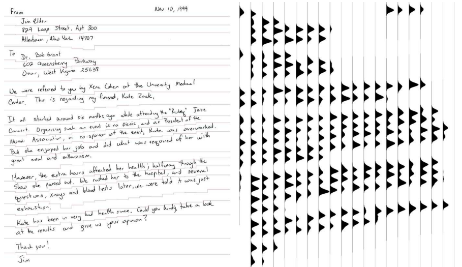
Figure 2.12: Left image shows segmented lines from a document in [7] and Right image displays projection profiles of vertical strips.
