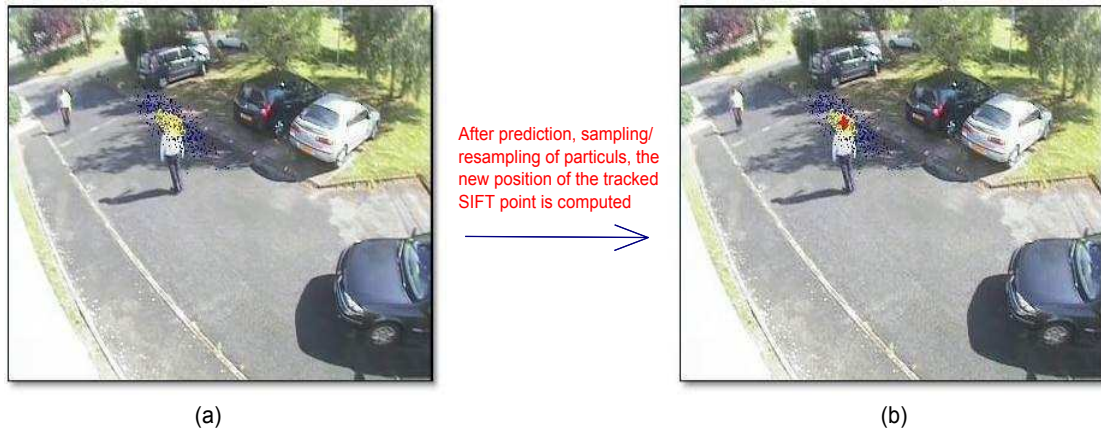
Figure 5.17: Tracking of one SIFT point on the head of a person by particle filter: (a) the predicted position of all particles in blue and yellow. The yellow particles are the sampled ones, which will be used to generate new ones to replace degenerated particles in blue. (b) in red, the new location of the tracked SIFT point, computed as the barycentre of all weighted sampled particles.
