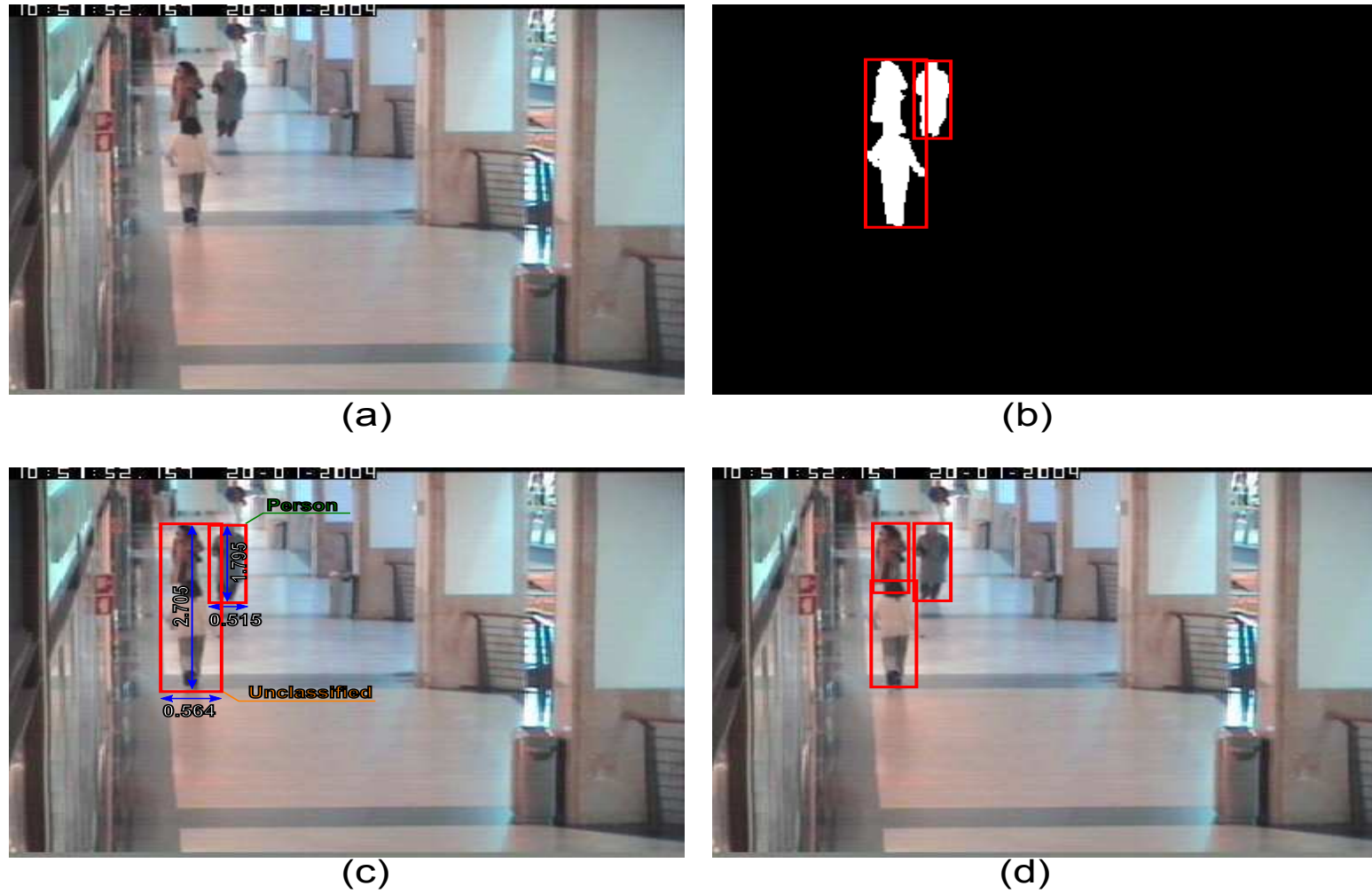
Figure 5.8: Use of people detector to split grouped persons. (a) Original frame. (b) Background subtraction result. Two persons are grouped due to the connected foreground pixels. (c) Failure of the classification of grouped people by real dimension estimation. (d) Result of our people detector applied in the restricted area of unclassified object (by real dimension estimation)
