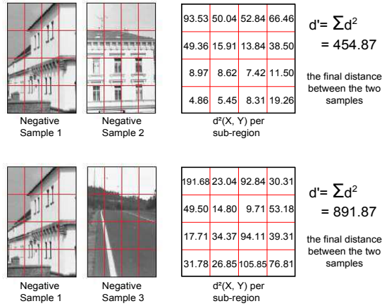
Figure 4.10: Negative image distance in the last pyramid level (4 x 4 subdivision), computed as the sum of squared distances between each pair of covariance matrices of the same subregion.
