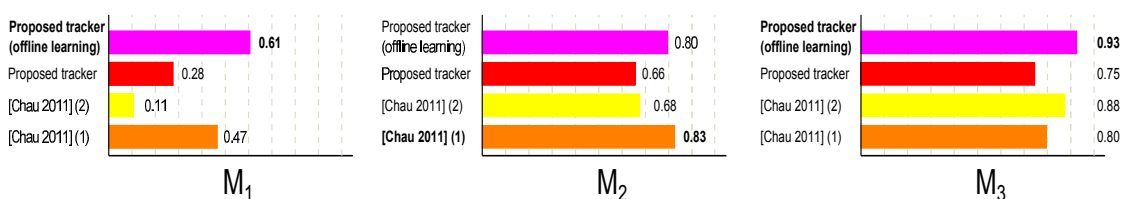
Figure 7.16: Comparative results on Caretaker sequence. [Chau 2011](1) refers to an off-line learning based tracker; [Chau 2011](2) is an estimator-based tracker.
