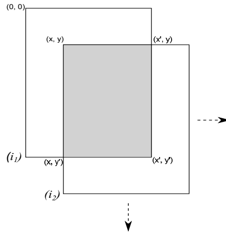
Figure 6.6: Images alignment
