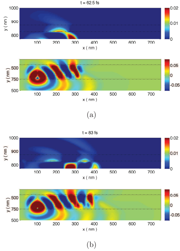
Figure 4.18: Snapshots of the structure after two elapsed times: (a) t_1 = 62.5 \text{ fs} , the SP_d mode is excited for the first time. (b) t_2 = 83 \text{ fs} , the SP_d mode is excited again after one period T_t . The structure is mapped in two parts because of the relative weakness of the field's amplitude for the surface mode, as compared to the guided mode.
