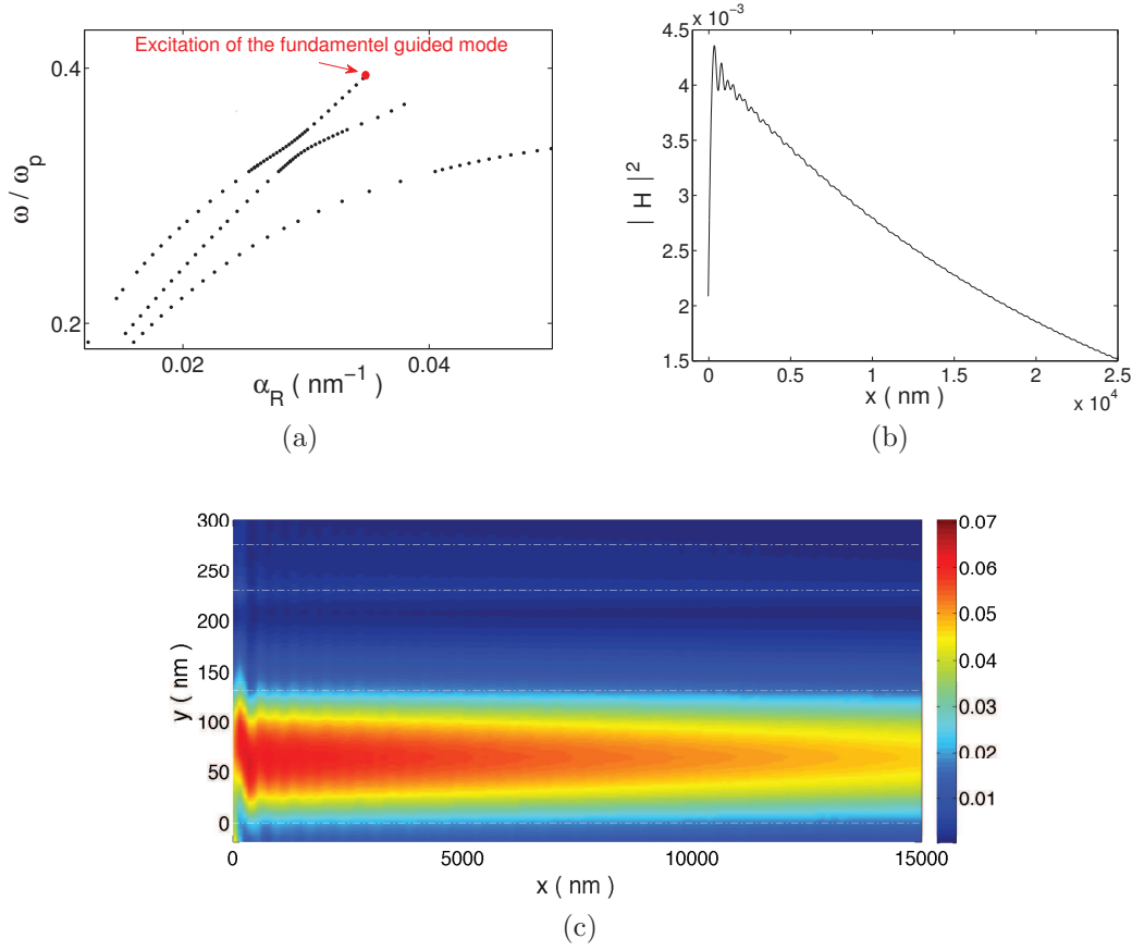
Figure 4.23: The fundamental guided mode far away from the anticrossing, excited by an evanescent gaussian beam with the Palik data [81]. (a) In the dispersion curves, we consider the point noted by a red dot characterized by \alpha_R = 0.0346 \text{ nm}^{-1} , at a wavelength \lambda = 349.5 \text{ nm} . (b) In one dimension, the intensity of the field in the center of the waveguide. (c) The corresponding map of the field in the plane (x, y) .
