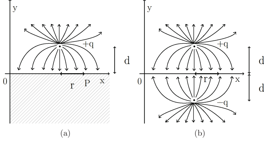
Figure 2.17: (a) Field lines created by an electric charge +q near a PEC substrate. (b) Field lines created by an electric dipole with a dipolar moment 2dq .
