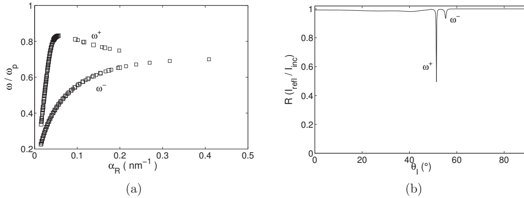
Figure 2.16: (a) Dispersion curves \omega^+ and \omega^- of the LRSP and the SRSP modes, respectively. \varepsilon_d = 1 is the permittivity of vacuum and the permittivity of the metal \varepsilon_m is taken from the experimental data of Palik [81]. The metallic thickness is e_m = 30 nm. (b) In the same conditions, the reflectivity is plotted as a function of the incident angle \theta_i . The half-width of the mode \omega^+ is smaller than the half-width of the mode \omega^- . Thus, the absorption of the LRSP mode is smaller than that of the SRSP mode.
