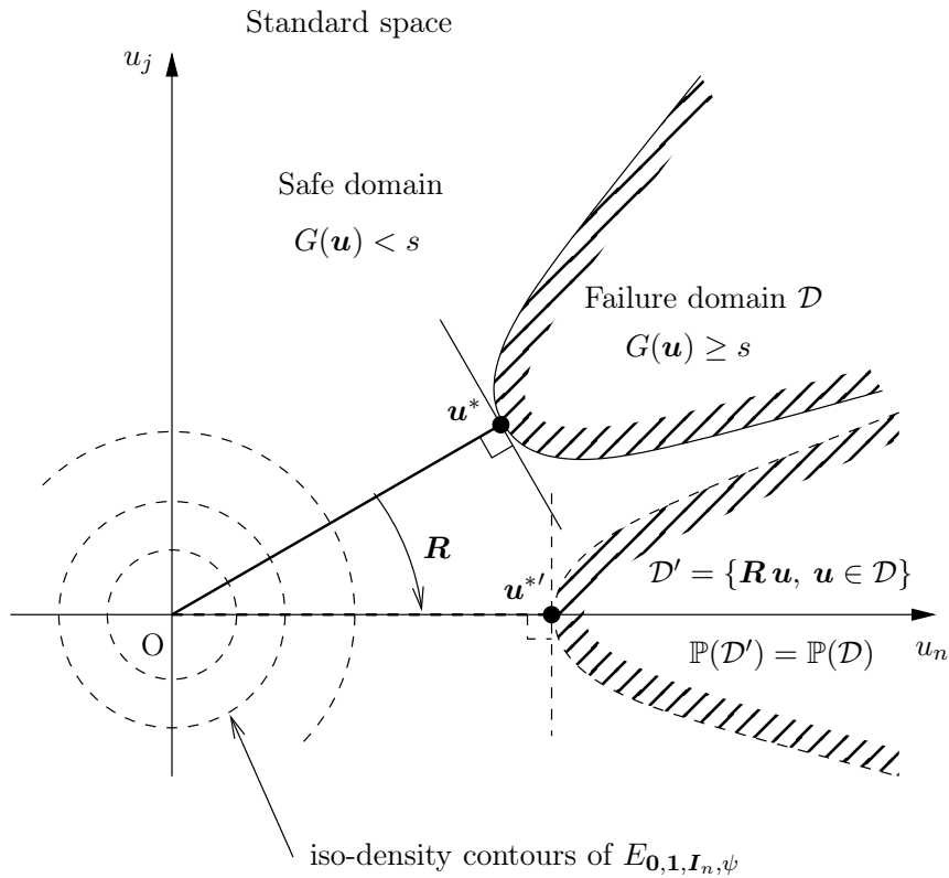
Figure 4.2: Rotational invariance after the application of the generalized Nataf transformation. The rotational invariance of \mathcal{E}_{\mathbf{0},\mathbf{1},\mathbf{I}_n,\psi} allows one to focus on the situation depicted in dashed form without loss of generality, thanks to the rotation \mathbf{R} that maps a general failure domain \mathcal{D} to a domain \mathcal{D}' for which the design point \mathbf{u}^{*'} is supported by the last axis.
