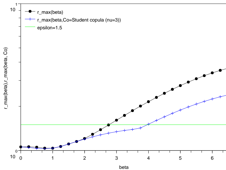
Figure 2.5: Evolution of r_{max}(\beta) and r_{max}(C_0, \beta) for \rho_S = 0.5 . We see that the range over which the estimate is quantitative is larger, even if it is still quite limited, and we see that the estimate is always at least qualitative.
