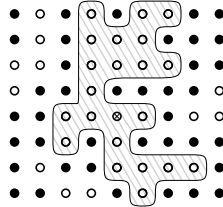
Figure D.2: Here the origin is crossed, the connected cluster of active sites is hatched and f(\eta) = 4 .
