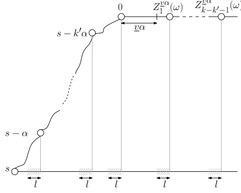
Figure B.3: The event \mathcal{Z} is such that the configuration at time s has a zero in each shaded box. The positions of these boxes depend on the initial configuration and on the dynamics up to the intermediate times s - i\alpha (via the positions of the front at times s - i\alpha ).
