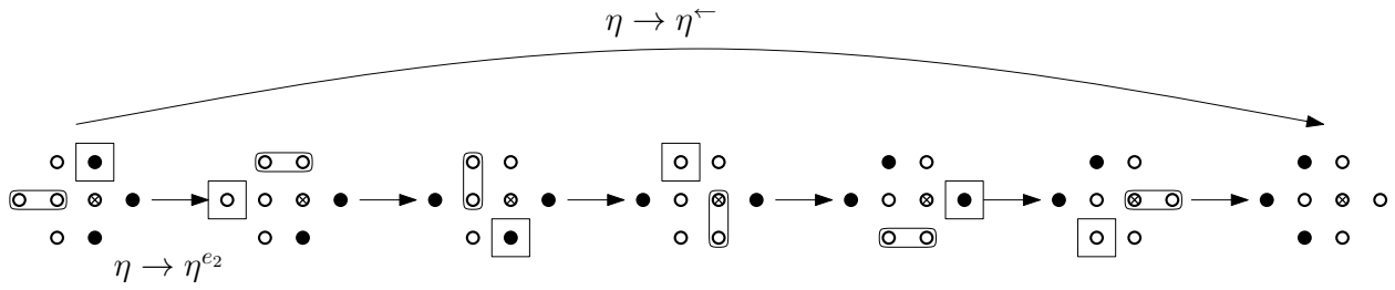
Figure C.8: An example of the reconstitution of the swap \eta \rightarrow \eta^{\leftarrow} using only legal flips and an extra zero (in the zone concerned, at any step there are at most 5 + 1 zeros). Before each step, the site to-be-flipped is inside a square, and the zeros that make the flip legal circled.
