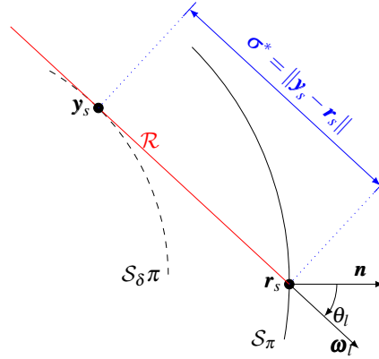
FIGURE 4: Existence du point \mathbf{y}_s
