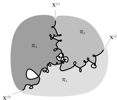
Figure 2.15 – Illustration de la preuve.
