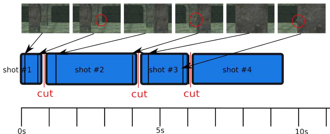
Figure 3.17 – Example #4: enforcing a full occlusion. In this example, the visibility is set to no visibility (interval [0;0] ). Therefore as soon as a part of the character is visible, the system automatically cuts to a new viewpoint where the character is occluded. On shots 2, 4 and 6 parts of the character which start to be visible are highlighted with a red circle, just before the system cuts to another viewpoint (time 0.9s, 4.3s and 6.1s).
