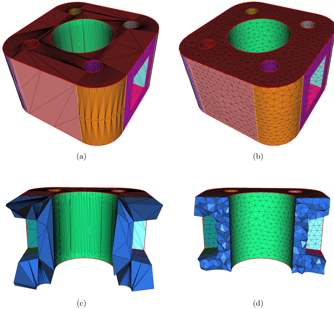
Figure 8.33: Remeshing of the model02 model, enclosed in a box of dimensions 0.199 \times 0.199 \times 0.12 . The parameters used for the computation are: h_{min} = 0.001 , h_{max} = 0.1 , h_{grad} = 1.2 and \varepsilon = 0.001 . (a)-(c) Initial mesh \mathcal{T} ; (b)-(d) final result \tilde{\mathcal{T}} .
