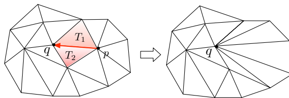
Figure 3.15: Point p is collapsed onto q ; the shell Sh(pq) vanishes in the process (in red), and the other triangles of \mathcal{B}(p) are updated.
