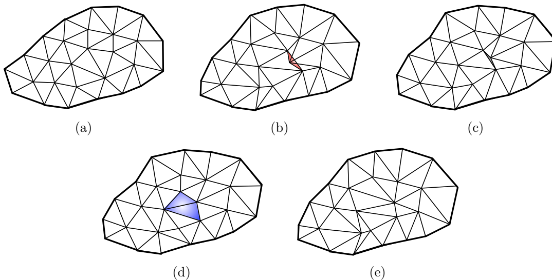
Figure 3.20: An example of mesh deformation procedure; (a) Initial mesh \mathcal{T} , (b) the invalid, advected mesh \mathcal{T}' (the element in red has been inverted), (c) the partially advected mesh \mathcal{T}' ; the greyed element is on the cusp of inversion, (d) the remeshed, partially advected configuration \widetilde{\mathcal{T}} ; an edge swap has made it possible to resolve the nearly degenerate configuration (in blue); (e) the final configuration \widetilde{\mathcal{T}} .
