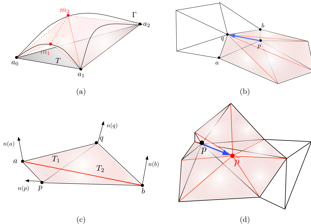
Figure 9.3: The four local remeshing operators, applied on a boundary configuration. In all four pictures, the previous configuration is shown in black, and the resulting one in red: (a) split of two edges a_0a_1 , a_0a_2 of a surface triangle T , (b) collapse along a boundary edge pq ; (c) swap of a boundary edge pq ; (d) relocation of a vertex p to an improving position \tilde{p} .
