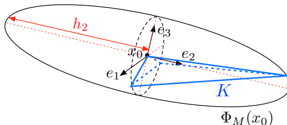
Figure 3.3: The unit ellipsoid \Phi_M(x_0) associated to a (constant) Riemannian metric M , with principal axis e_1, e_2, e_3 , and associated principal radii h_1, h_2, h_3 . In blue, a unit simplex K with respect to M , sharing x_0 as a vertex, is depicted.
