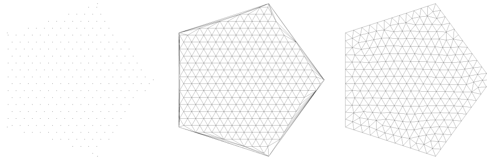
Figure 3.12: Illustration of Persson's method; ( left ) initial set of points \mathcal{P} , ( middle ) Delaunay triangulation of \text{conv}(\mathcal{P}) , and ( right ) final mesh after node relocations.
