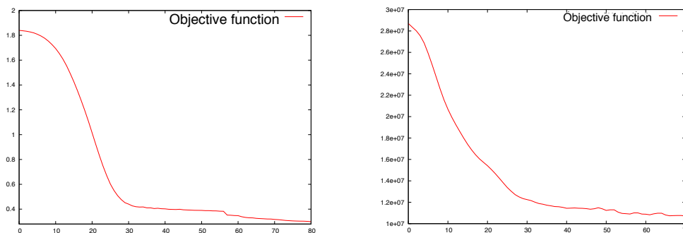
Figure 9.13: (Left) convergence history for the 3d Cantilever test-case, (right) convergence history for the 3d Optimal Bridge test-case.
