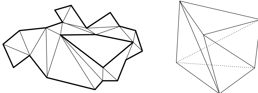
Figure 3.4: ( Left ): In two dimensions, any polygonal domain can be triangulated using only the vertices of its boundary; ( right ) in three dimensions, Schönardt's polyhedron is a non-convex polyhedron obtained by twisting a certain partition of a regular prism. It cannot be meshed without introducing any internal point.
