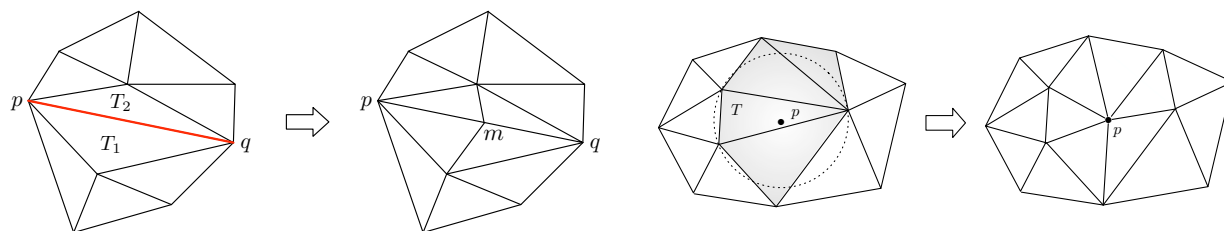
Figure 3.14: In two dimensions, ( left ) Splitting an edge pq leads to the formation of four triangles, ( right ) illustration of the Delaunay refinement procedure: the centre p of the circumcircle of T is inserted in \mathcal{T} , using the Delaunay kernel.
