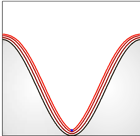
Figure 1.3: Several positions \Omega(t) , for t = 0, 0.02, 0.04 , and t = 0.055 (from bottom to top), in the flame propagation model. \Omega(0) (in grey) is of class C^\infty ; however, a singularity (blue dot) develops at a finite time, at approximately t = t_c = 0.055 .
