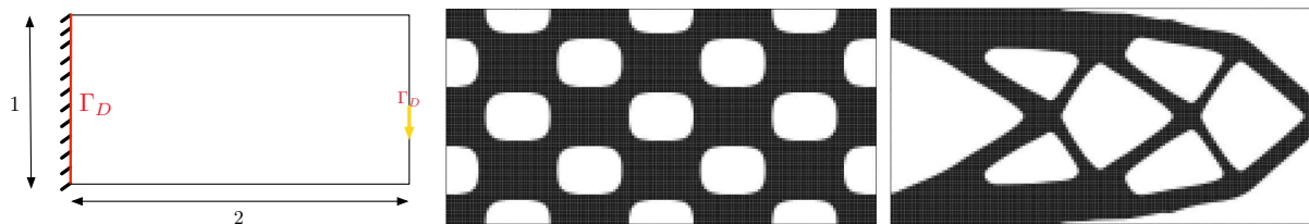
Figure 2.4: (Left) Boundary conditions, (middle) initialization, and (right) resulting shape in the cantilever test case (reprinted from [14]).
