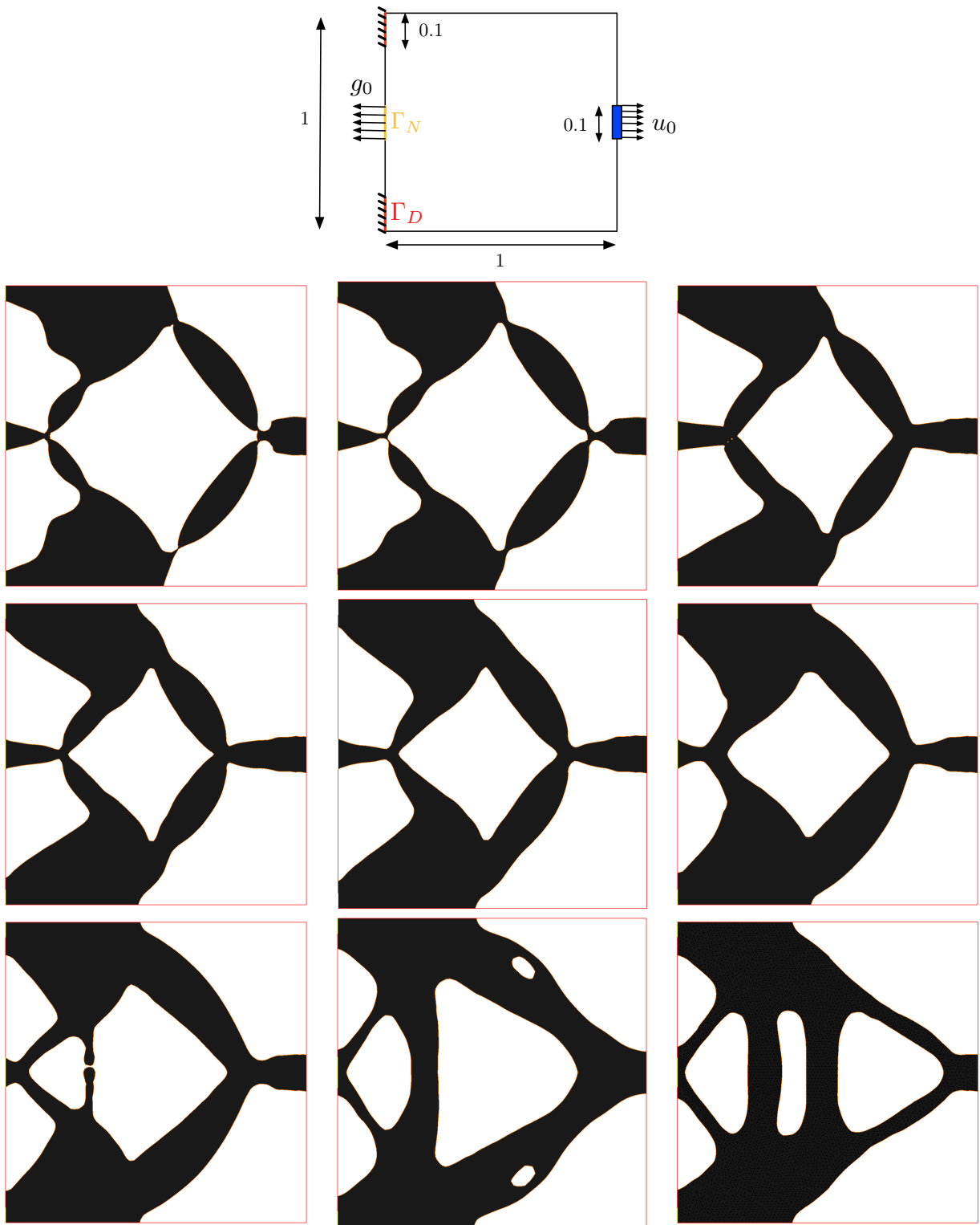
Figure 5.14: (From left to right, top to bottom): details of the test-case, optimal shape for the worst case force inverter test case, with perturbations over the Lamé coefficients of the material of magnitude m = 0, 0.001, 0.002, 0.003, 0.0045, 0.0075, 0.01, 0.02, 0.1 .
