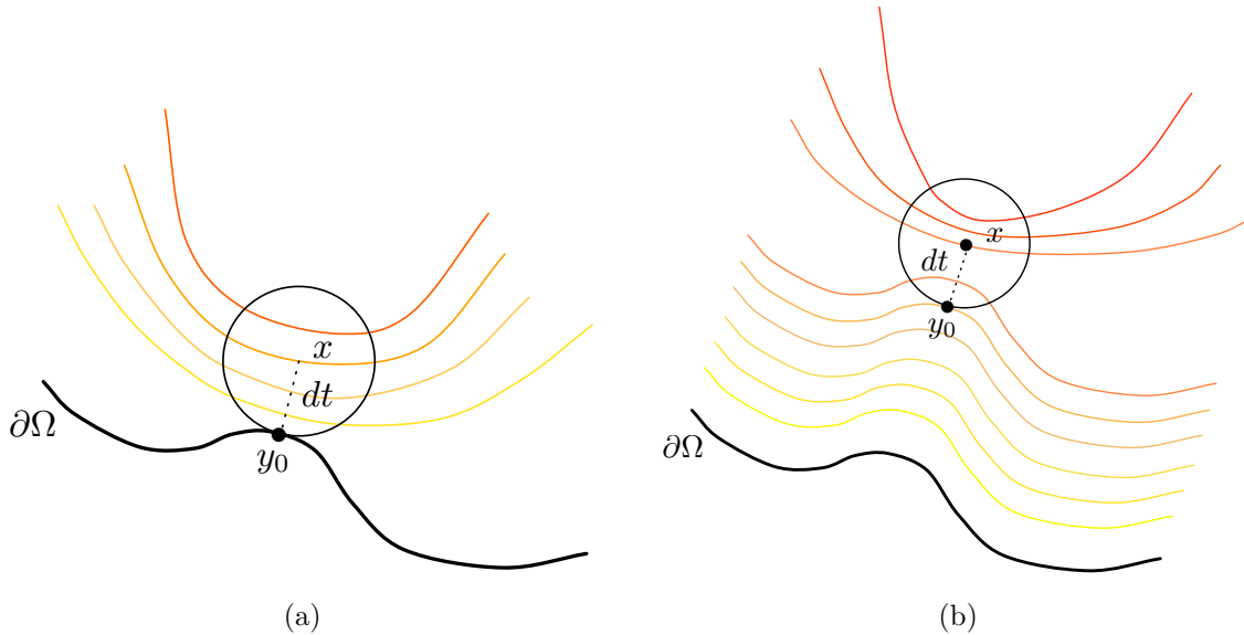
Figure 6.1: At a given iteration n , the proposed numerical scheme amounts to ‘straighten up’ the value of d^n at point x from its value at point y_0 in such a way that d^n(y_0) = \inf_{y \in B(x, dt)} d^n(y) with the property of unitary gradient, (a) e.g. for a point x at distance dt from \partial\Omega , d^1(x) = d_0(y_0) + dt = dt = d(x, \partial\Omega) . (b) The property of unit gradient ‘propagates’ from the boundary \partial\Omega , near which values of d^n are ‘regularized’ at an early stage.
