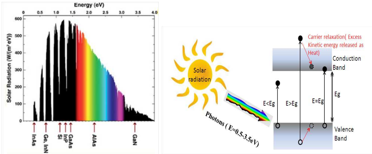
(a) AM 1.5 solar spectrum. Arrows indicate the bandgaps of some semiconductors.
