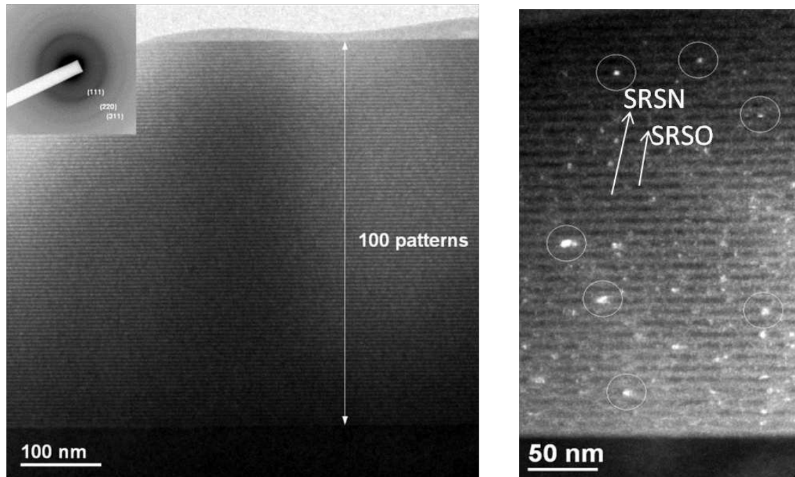
(a) General microstructure and electron diffraction pattern.
