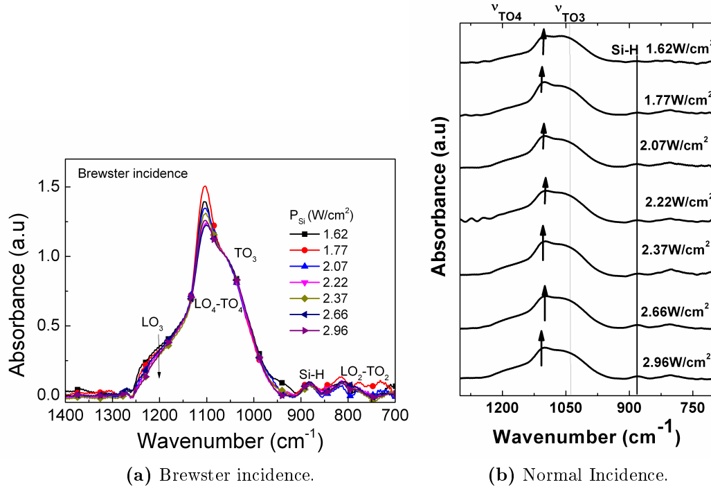
Figure 3.10: FTIR Spectra- Effect of P_{Si} on the SRSO film structure.
