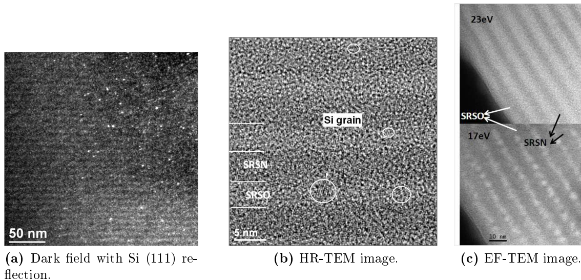
Figure 4.34: Microstructural investigations by (a) TEM, (b) HR-TEM and (c) EF-TEM imaged with Si (17eV) plasmon and O (23eV) plasmon.
