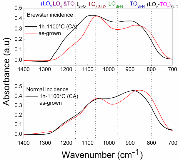
Figure 4.20: FTIR spectra of as-grown and CA 100(3.5/5) ML.
