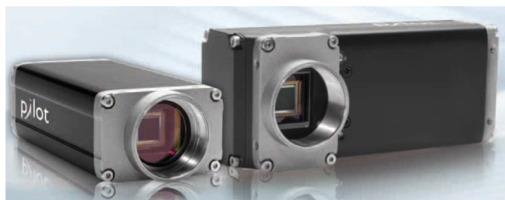
Figure 1.2: Basler high speed camera, Pilot piA640-210gm model, 648 x 488 resolution, 210 fps, monochrome, with GigE Vision interface. The camera achieves 210 fps at full resolution. Frame rate can still be increased by reducing the resolution. This is an industrial camera that can adapt to entry level high speed applications in reduced resolution mode with a moderate cost, typically several hundred euros. Image courtesy of Basler user manual Pilot series.
