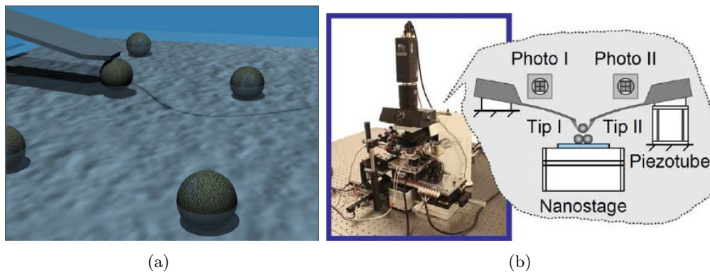
Figure 1.19: (a) Haptic feedback serves as a virtual guide to keep the user's motion on a specified path. Image courtesy of [Ammi 2007]. (b) Virtual guides for pick-and-place operation of microspheres based on two atomic force microscopy cantilevers. The laser beams have to be aligned with the cantilevers and photodiodes. Image courtesy of [Bolo pion 2012].
