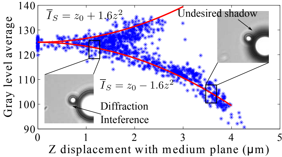
Figure 3.3: A non-linear relation exists between the z displacement of probe with respect to the medium line of the 10\ \mu\text{m} sphere and the average gray level intensity \bar{I}_S . A second order polynomial is used to approximate this relation. The branch above (the '+' sign part of the fitted equation) shows the relation when the displacement of the probe in z is upwards with respect to the medium line of the target, while the branch below (the '-' sign part) signify the displacement downwards. The insets shows diffraction ring interferences and undesired shadow projection on the probe.
