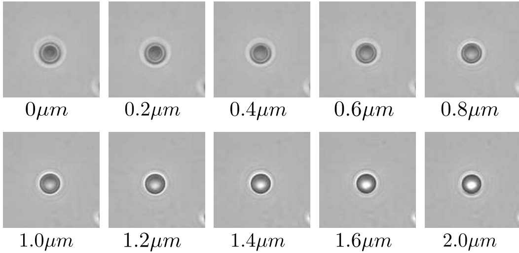
Figure 3.1: An sphere of diameter 3 \mu\text{m} stays in the same location of the xy plane but varies in z . Diffraction generates the spherical radial profile that exhibits oscillating light intensities.
