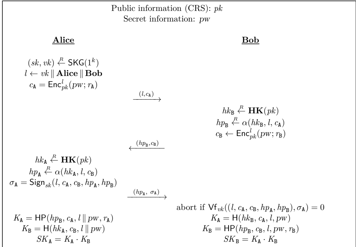
Figure 2.4: An overview of the Gennaro-Lindell PAKE protocol [GL03]. (KG, Enc, Dec) are the key generation, encryption, and decryption algorithms of a labeled public-key encryption scheme [Sho04]. (SKG, Sign, Vf) are the key generation, signing, and verification algorithms of a one-time signature scheme [EGM96]. (HK, \alpha , H, HP) are the key generation, key projection, hashing, and projected hashing algorithms of a family of smooth projective hash functions for the language L consisting of triples \{(c, \ell, pw)\} such that c is an encryption of the password pw with label \ell .
