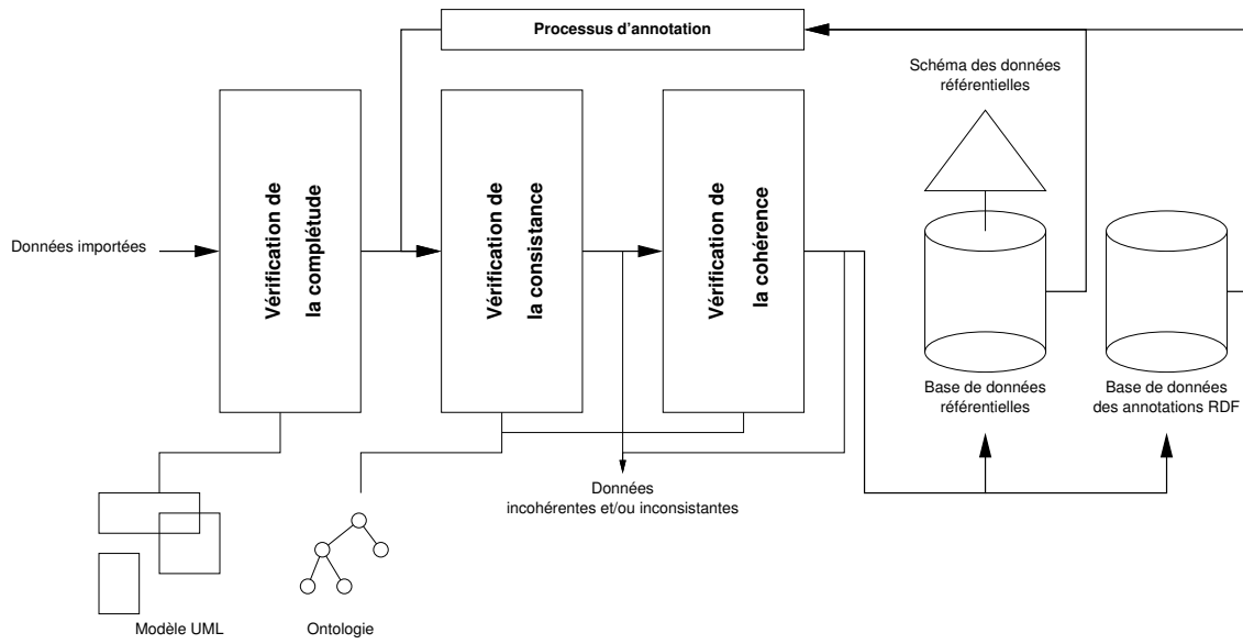
FIGURE 5.3 – Architecture du composant eClims
